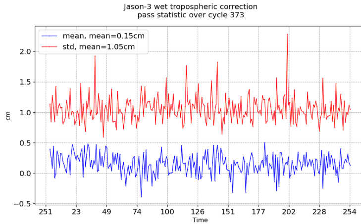
FIGURE 11 – Pass monitoring of wet troposphere differences between radiometer and ECMWF model for Jason-3 cycle 373
