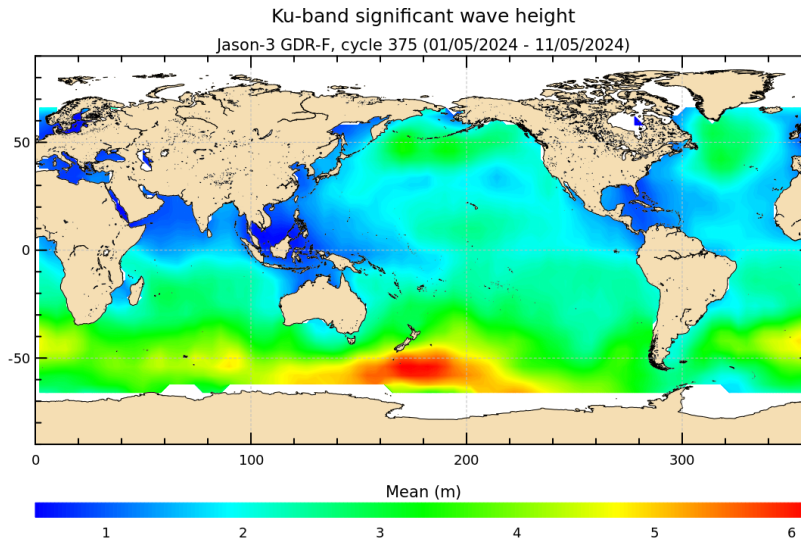
FIGURE 5 – Significant wave height for cycle 375.
