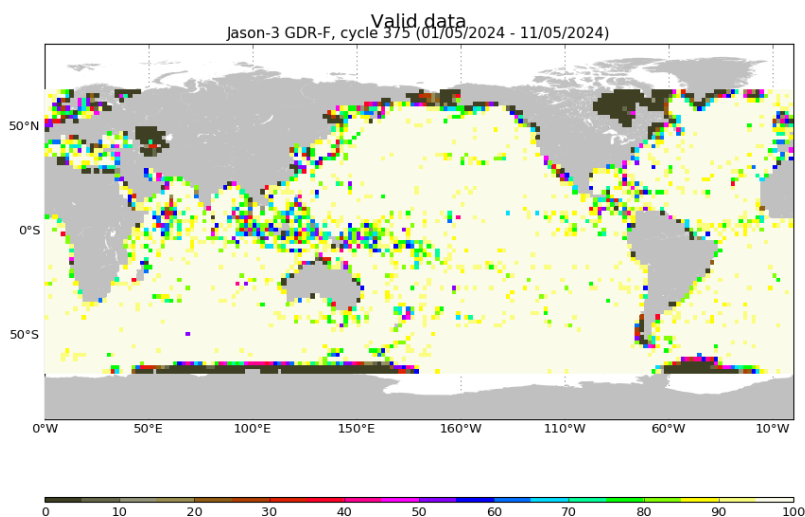
FIGURE 3 – Percentage of valid measurements for cycle 375.
