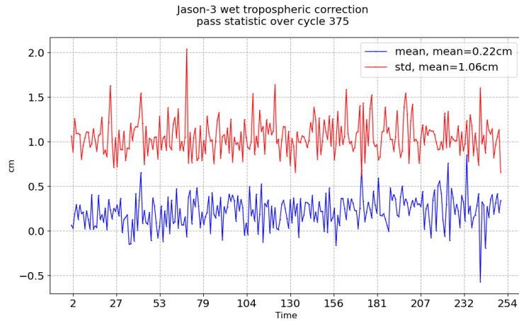
FIGURE 11 – Pass monitoring of wet troposphere differences between radiometer and ECMWF model for Jason-3 cycle 375
