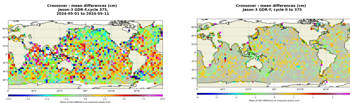
FIGURE 13 – Mean SSH at crossovers for cycle 375 (left) and over the whole Jason-3 period (right).
