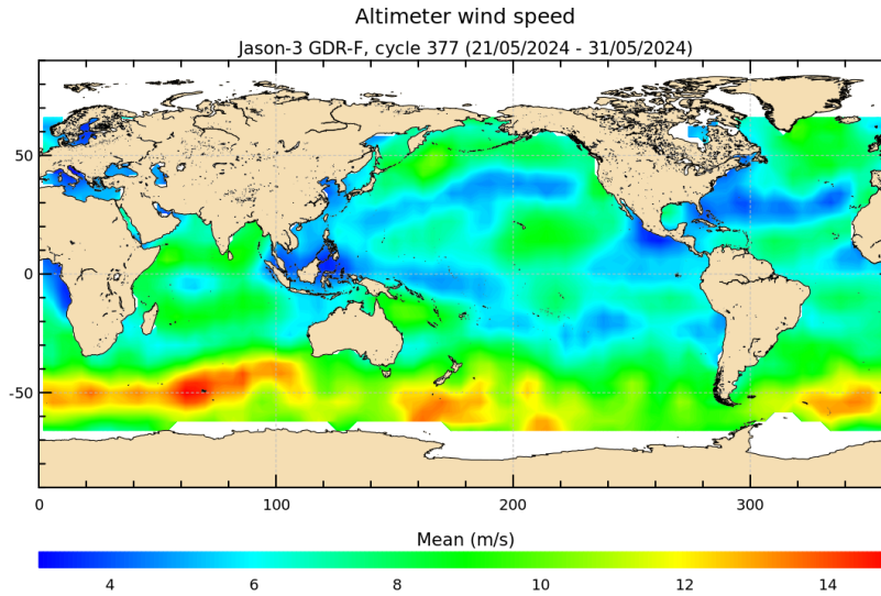
FIGURE 9 – Altimeter wind speed for cycle 377.
