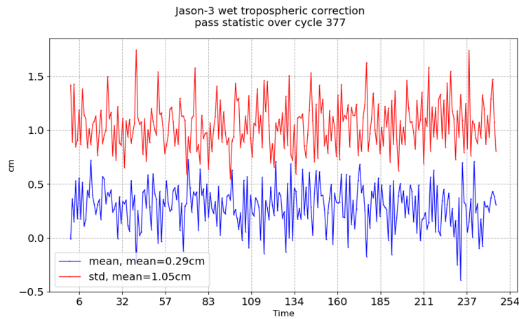
FIGURE 11 – Pass monitoring of wet troposphere differences between radiometer and ECMWF model for Jason-3 cycle 377
