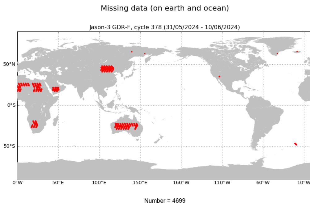
FIGURE 1 – Missing measurements for cycle 378.
