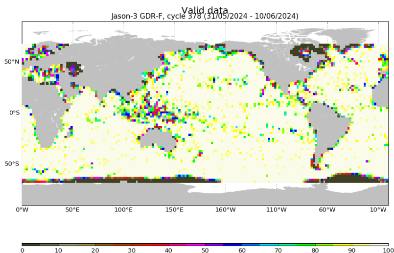
FIGURE 3 – Percentage of valid measurements for cycle 378.
