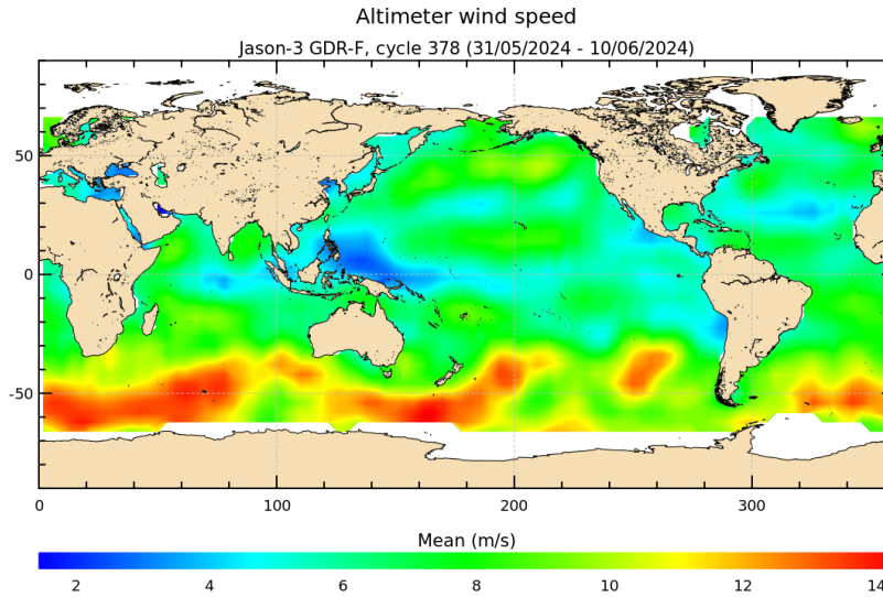
FIGURE 9 – Altimeter wind speed for cycle 378.
