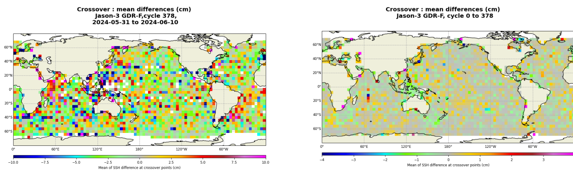
FIGURE 13 – Mean SSH at crossovers for cycle 378 (left) and over the whole Jason-3 period (right).
