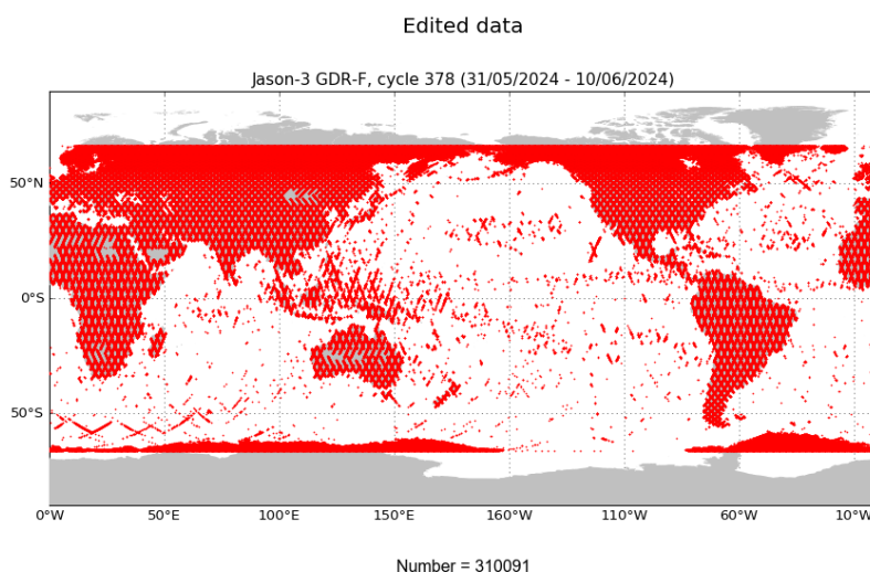
FIGURE 2 – Edited measurements for cycle 378.
