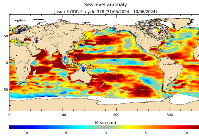
FIGURE 18 – Sea level anomaly relative to MSS for cycle 378.
