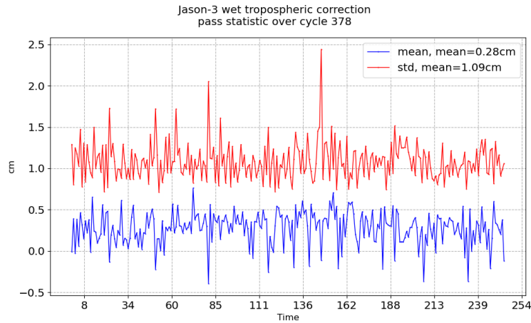
FIGURE 11 – Pass monitoring of wet troposphere differences between radiometer and ECMWF model for Jason-3 cycle 378
