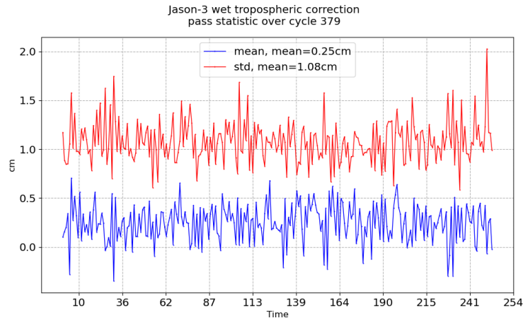
FIGURE 11 – Pass monitoring of wet troposphere differences between radiometer and ECMWF model for Jason-3 cycle 379
