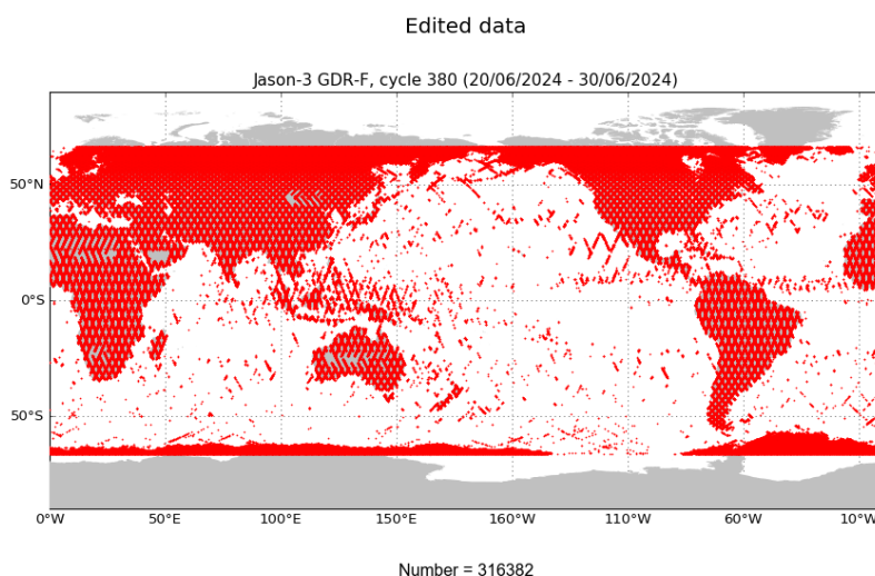
FIGURE 2 – Edited measurements for cycle 380.
