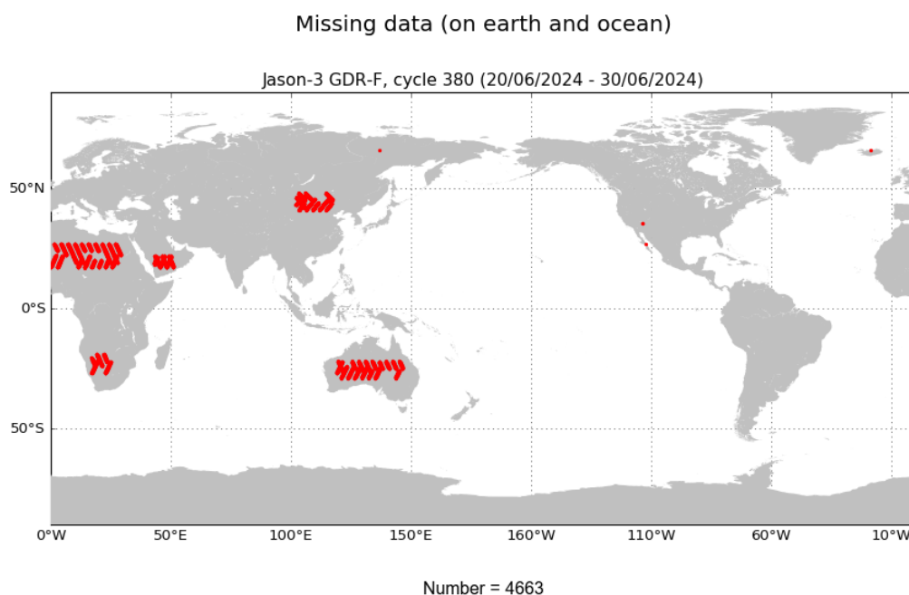
FIGURE 1 – Missing measurements for cycle 380.
