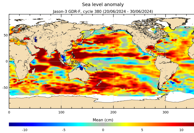
FIGURE 18 – Sea level anomaly relative to MSS for cycle 380.
