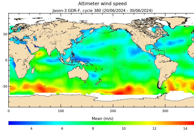
FIGURE 9 – Altimeter wind speed for cycle 380.
