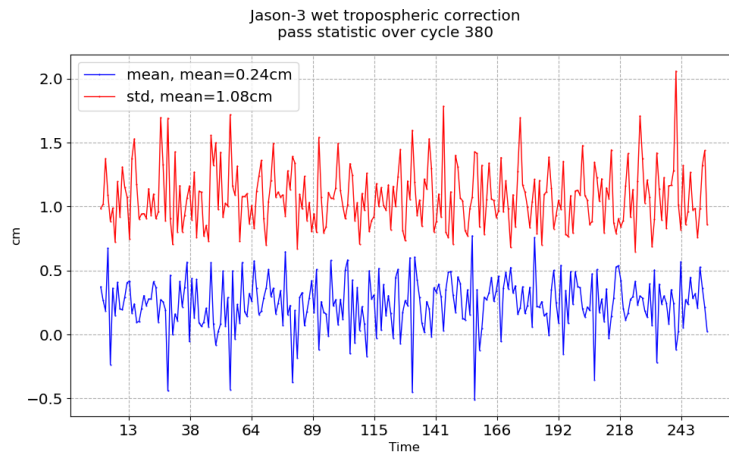
FIGURE 11 – Pass monitoring of wet troposphere differences between radiometer and ECMWF model for Jason-3 cycle 380
