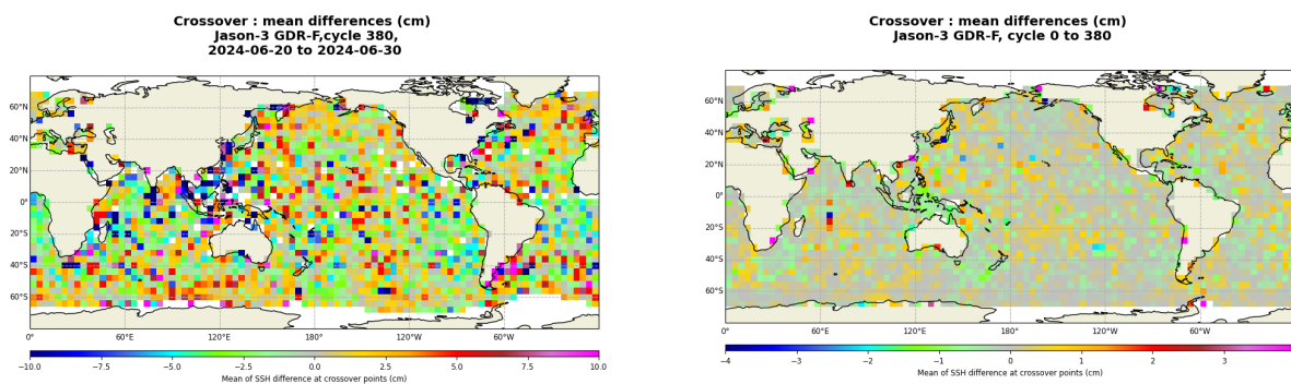
FIGURE 13 – Mean SSH at crossovers for cycle 380 (left) and over the whole Jason-3 period (right).
