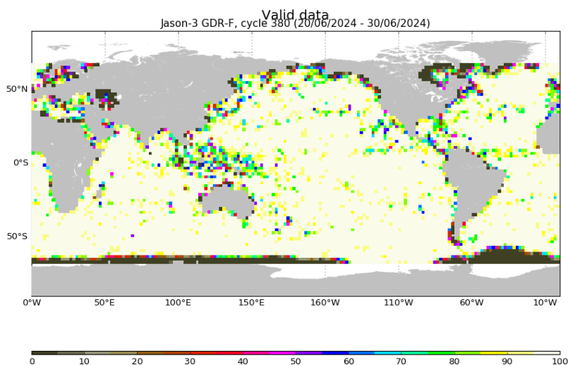
FIGURE 3 – Percentage of valid measurements for cycle 380.
