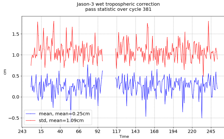
FIGURE 11 – Pass monitoring of wet troposphere differences between radiometer and ECMWF model for Jason-3 cycle 381
