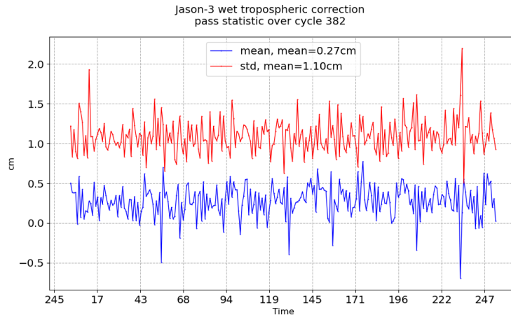
FIGURE 11 – Pass monitoring of wet troposphere differences between radiometer and ECMWF model for Jason-3 cycle 382
