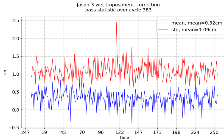
FIGURE 11 – Pass monitoring of wet troposphere differences between radiometer and ECMWF model for Jason-3 cycle 383
