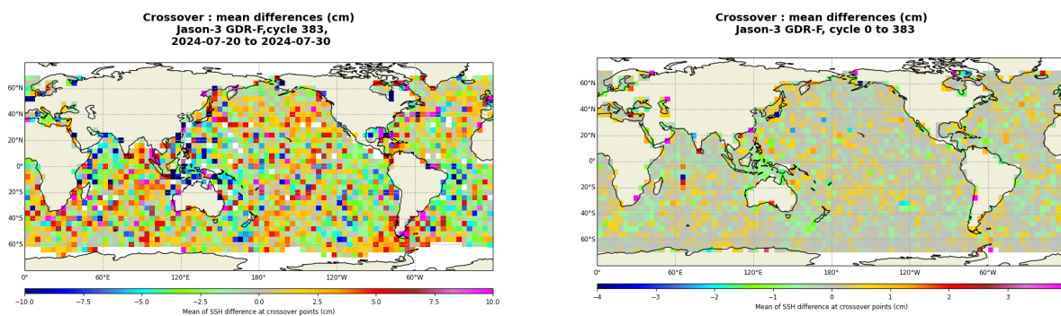
FIGURE 13 – Mean SSH at crossovers for cycle 383 (left) and over the whole Jason-3 period (right).
