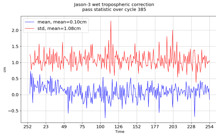
FIGURE 11 – Pass monitoring of wet troposphere differences between radiometer and ECMWF model for Jason-3 cycle 385
