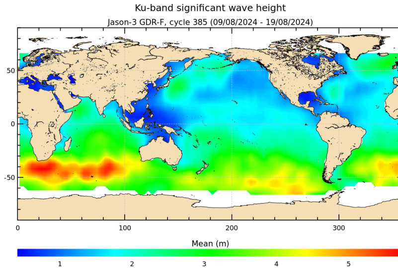
FIGURE 5 – Significant wave height for cycle 385.
