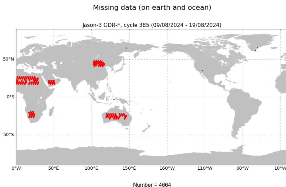
FIGURE 1 – Missing measurements for cycle 385.
