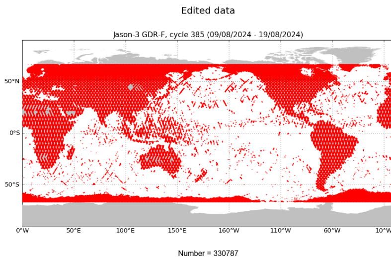
FIGURE 2 – Edited measurements for cycle 385.
