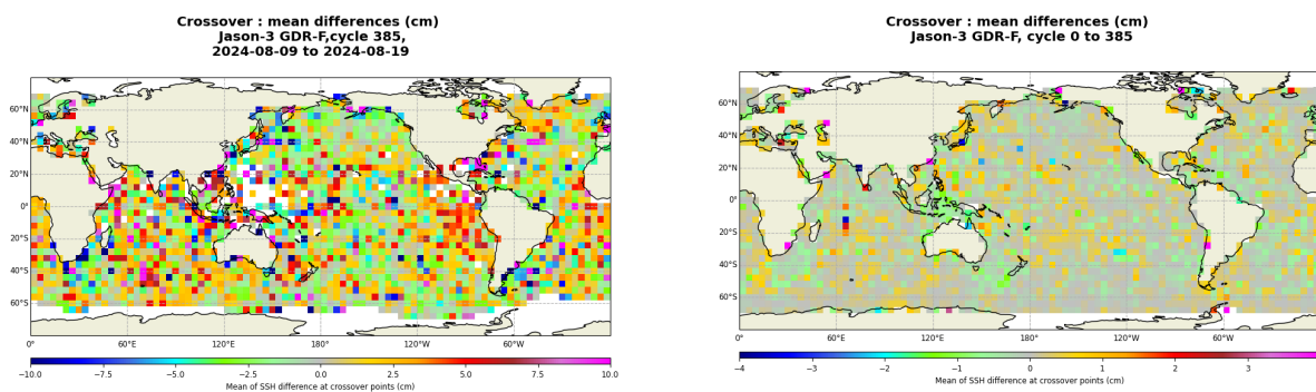
FIGURE 13 – Mean SSH at crossovers for cycle 385 (left) and over the whole Jason-3 period (right).
