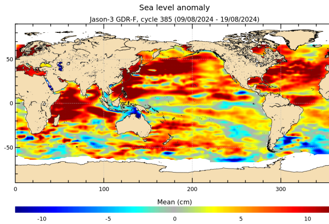
FIGURE 18 – Sea level anomaly relative to MSS for cycle 385.
