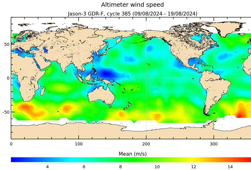
FIGURE 9 – Altimeter wind speed for cycle 385.
