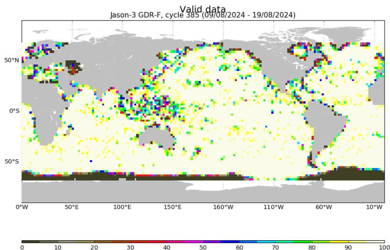
FIGURE 3 – Percentage of valid measurements for cycle 385.
