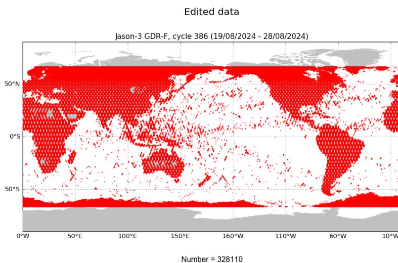
FIGURE 2 – Edited measurements for cycle 386.
