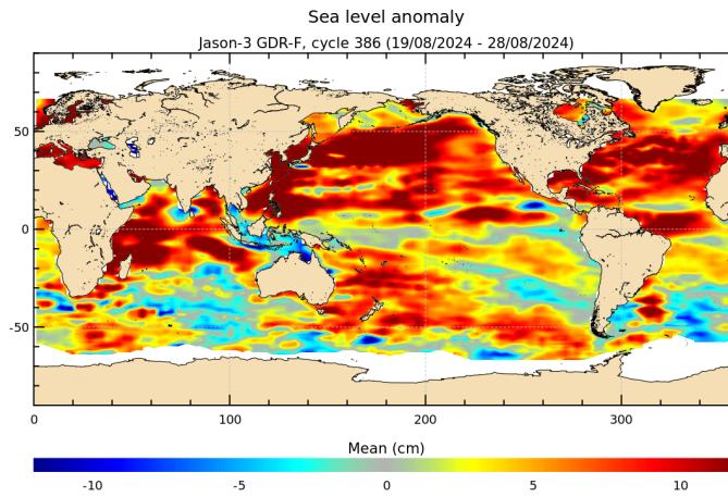
FIGURE 18 – Sea level anomaly relative to MSS for cycle 386.
