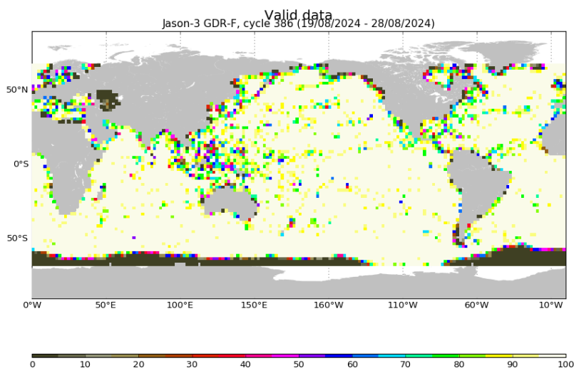
FIGURE 3 – Percentage of valid measurements for cycle 386.
