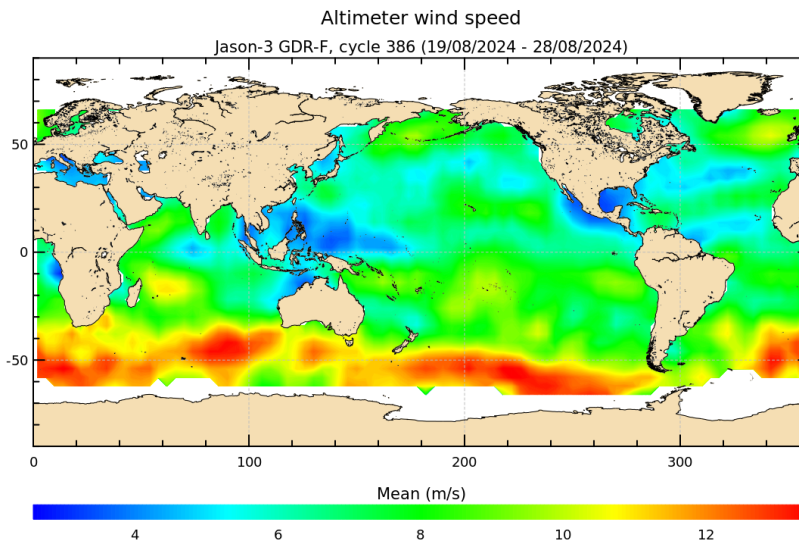
FIGURE 9 – Altimeter wind speed for cycle 386.
