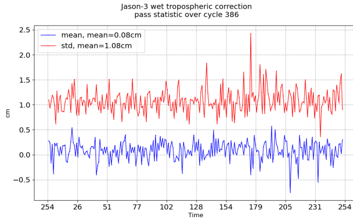
FIGURE 11 – Pass monitoring of wet troposphere differences between radiometer and ECMWF model for Jason-3 cycle 386
