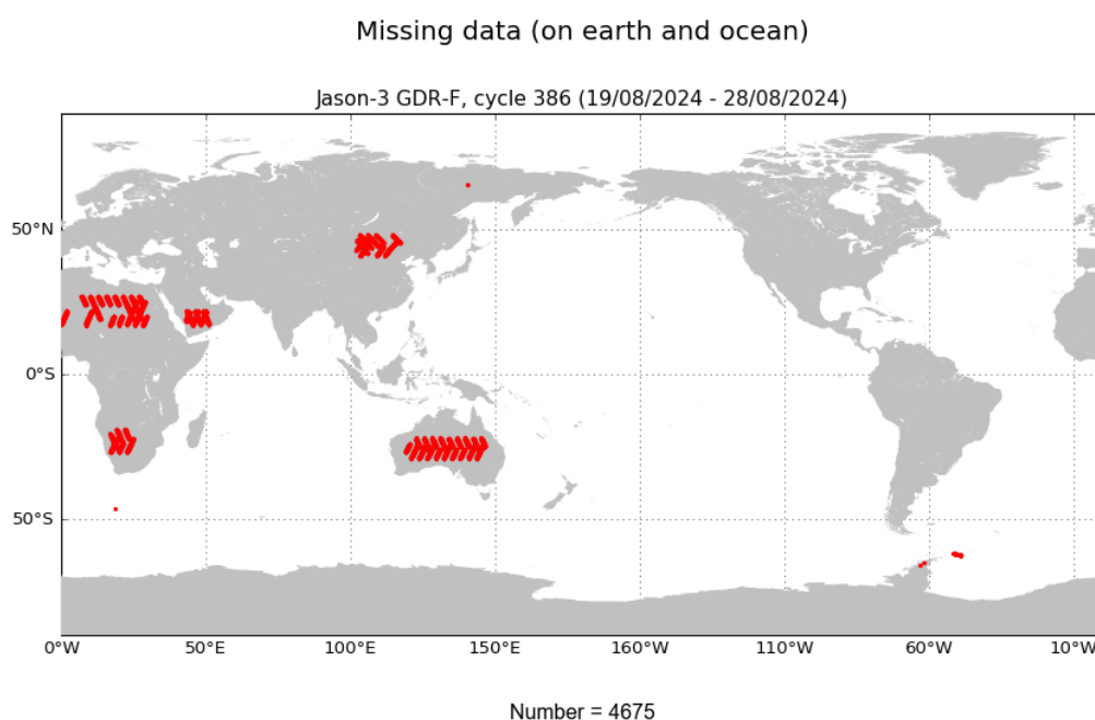
FIGURE 1 – Missing measurements for cycle 386.
