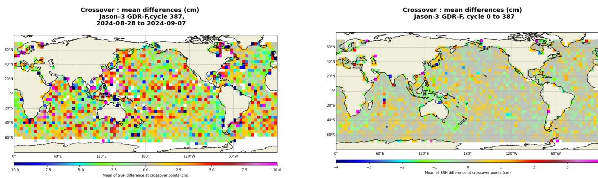
FIGURE 13 – Mean SSH at crossovers for cycle 387 (left) and over the whole Jason-3 period (right).
