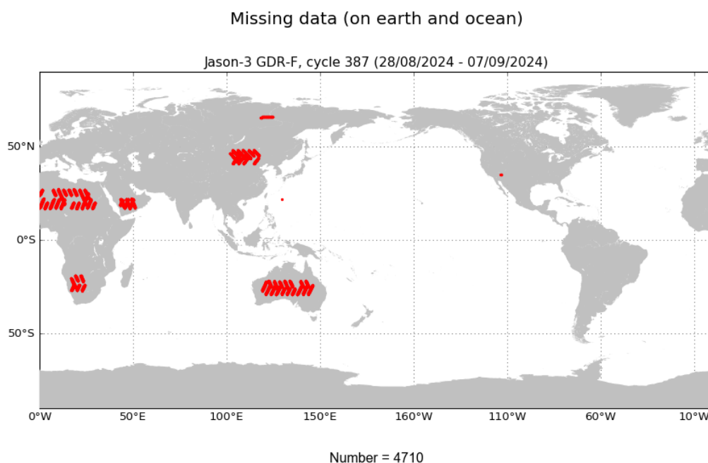
FIGURE 1 – Missing measurements for cycle 387.
