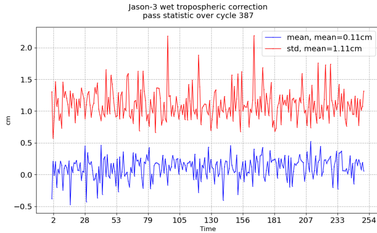
FIGURE 11 – Pass monitoring of wet troposphere differences between radiometer and ECMWF model for Jason-3 cycle 387
