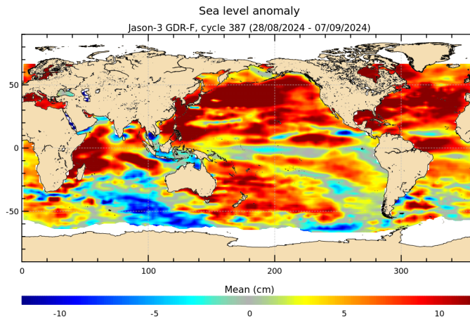
FIGURE 18 – Sea level anomaly relative to MSS for cycle 387.
