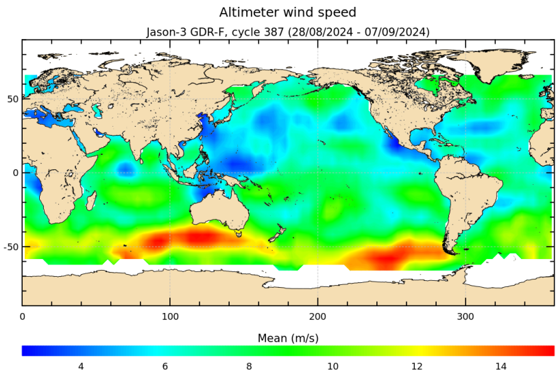
FIGURE 9 – Altimeter wind speed for cycle 387.
