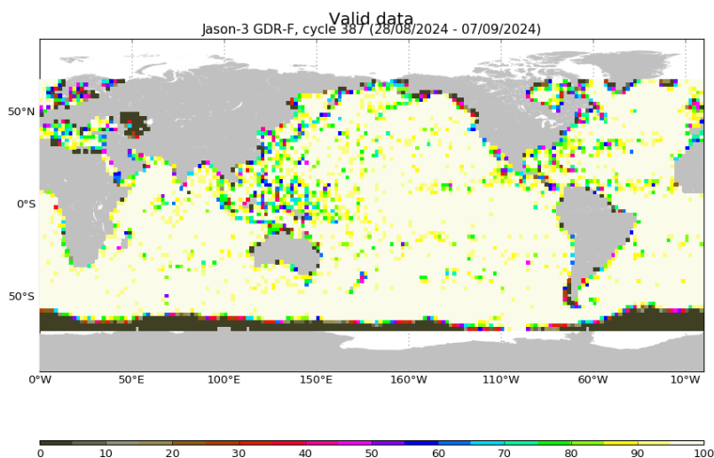
FIGURE 3 – Percentage of valid measurements for cycle 387.
