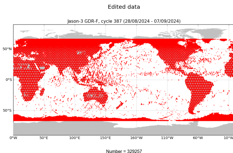
FIGURE 2 – Edited measurements for cycle 387.
