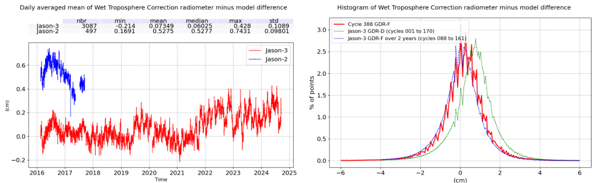
FIGURE 12 – Daily monitoring of wet troposphere differences between radiometer and ECMWF model for Jason-2 and Jason-3 (left) and histograms of Jason-3 (right).
