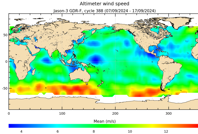
FIGURE 9 – Altimeter wind speed for cycle 388.
