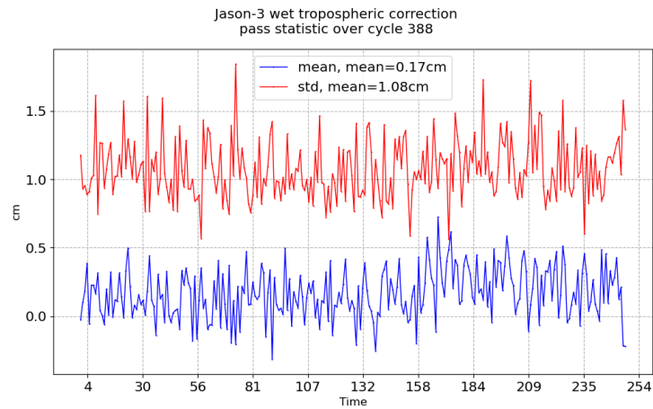
FIGURE 11 – Pass monitoring of wet troposphere differences between radiometer and ECMWF model for Jason-3 cycle 388
