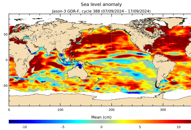
FIGURE 18 – Sea level anomaly relative to MSS for cycle 388.
