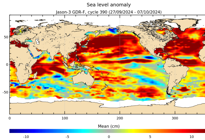
FIGURE 18 – Sea level anomaly relative to MSS for cycle 390.
