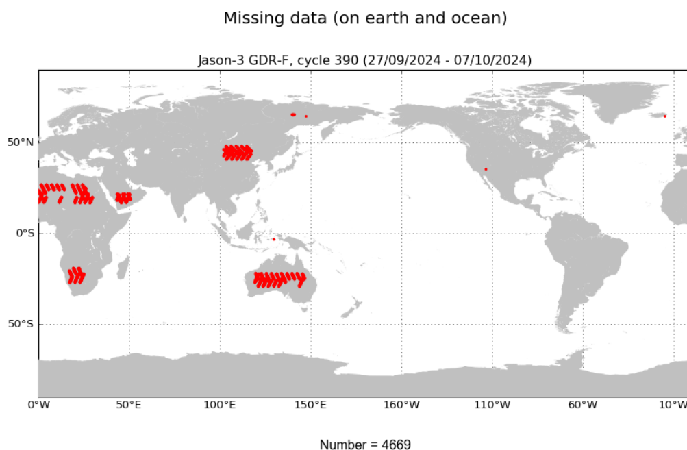
FIGURE 1 – Missing measurements for cycle 390.
