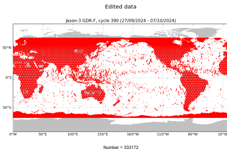
FIGURE 2 – Edited measurements for cycle 390.
