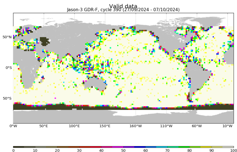
FIGURE 3 – Percentage of valid measurements for cycle 390.
