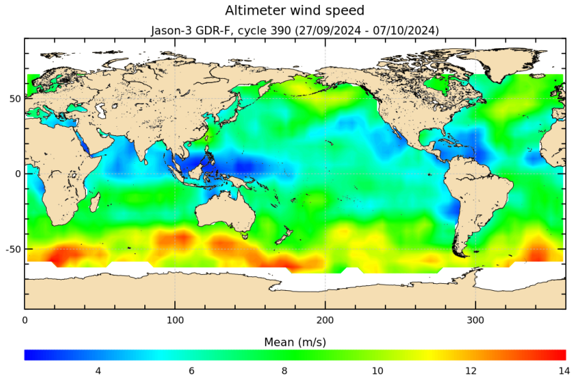
FIGURE 9 – Altimeter wind speed for cycle 390.
