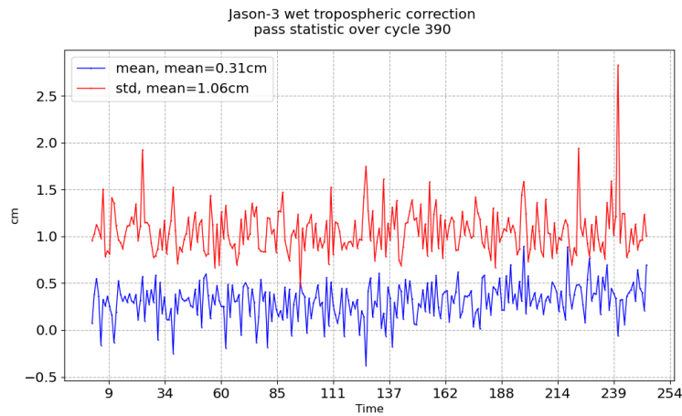
FIGURE 11 – Pass monitoring of wet troposphere differences between radiometer and ECMWF model for Jason-3 cycle 390
