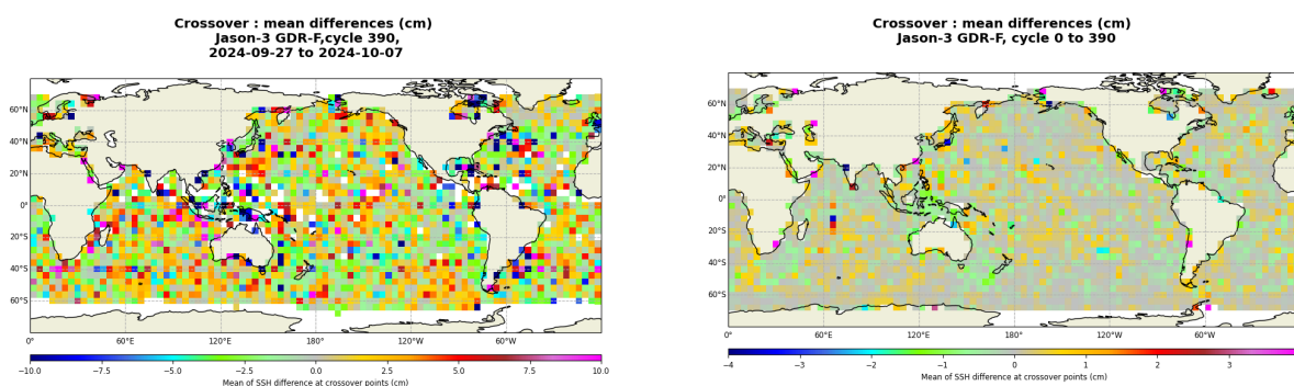
FIGURE 13 – Mean SSH at crossovers for cycle 390 (left) and over the whole Jason-3 period (right).
