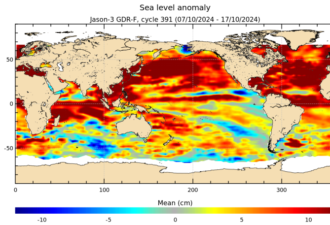
FIGURE 18 – Sea level anomaly relative to MSS for cycle 391.
