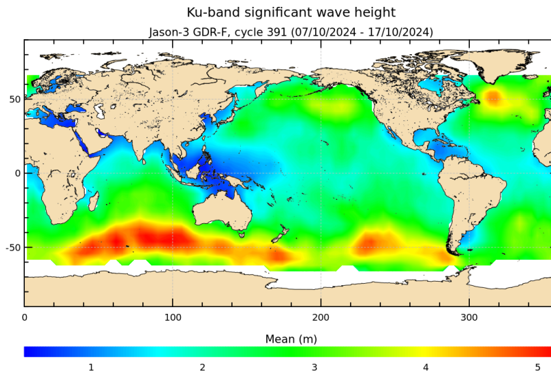
FIGURE 5 – Significant wave height for cycle 391.
