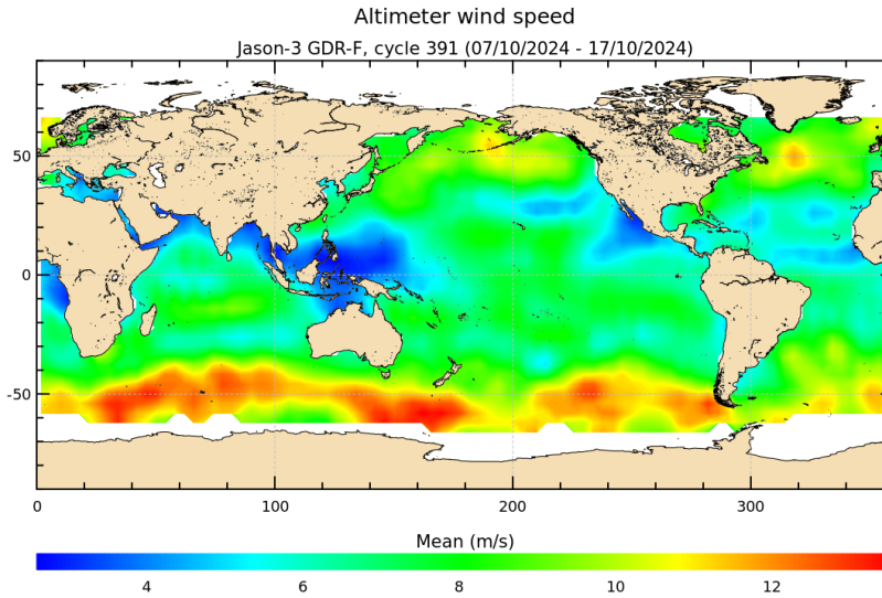
FIGURE 9 – Altimeter wind speed for cycle 391.
