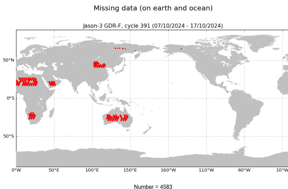
FIGURE 1 – Missing measurements for cycle 391.
