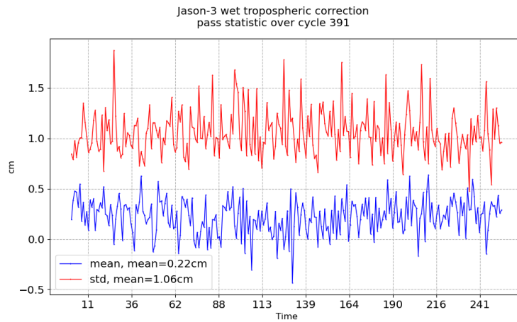
FIGURE 11 – Pass monitoring of wet troposphere differences between radiometer and ECMWF model for Jason-3 cycle 391
