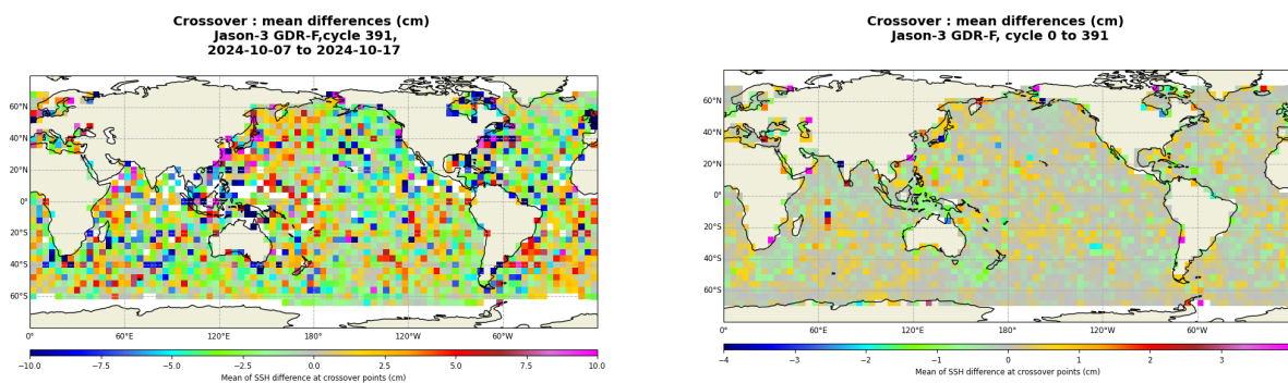
FIGURE 13 – Mean SSH at crossovers for cycle 391 (left) and over the whole Jason-3 period (right).
