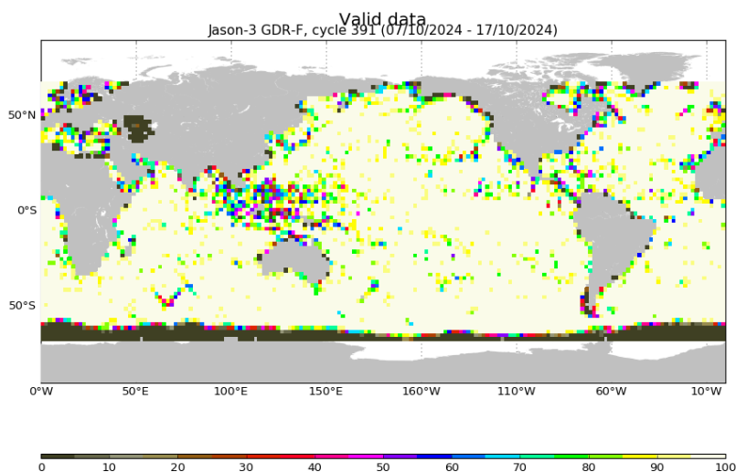
FIGURE 3 – Percentage of valid measurements for cycle 391.
