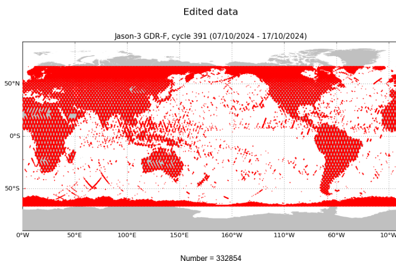
FIGURE 2 – Edited measurements for cycle 391.
