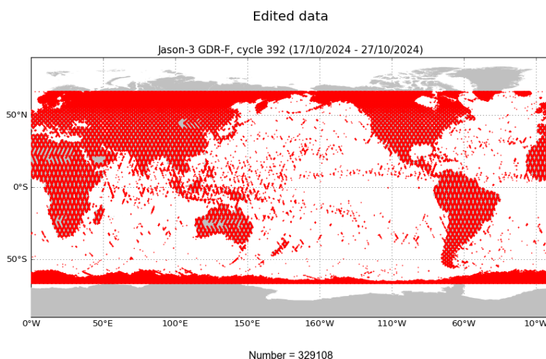
FIGURE 2 – Edited measurements for cycle 392.
