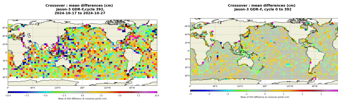
FIGURE 13 – Mean SSH at crossovers for cycle 392 (left) and over the whole Jason-3 period (right).
