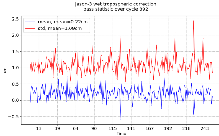
FIGURE 11 – Pass monitoring of wet troposphere differences between radiometer and ECMWF model for Jason-3 cycle 392
