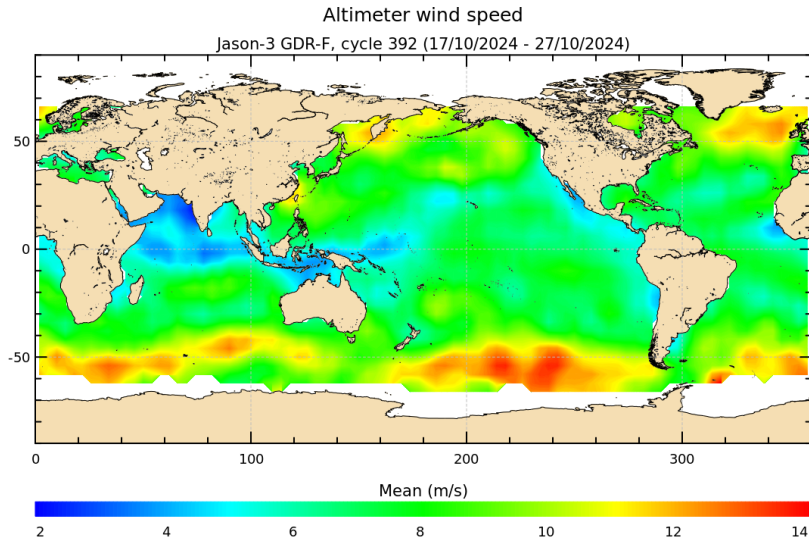
FIGURE 9 – Altimeter wind speed for cycle 392.
