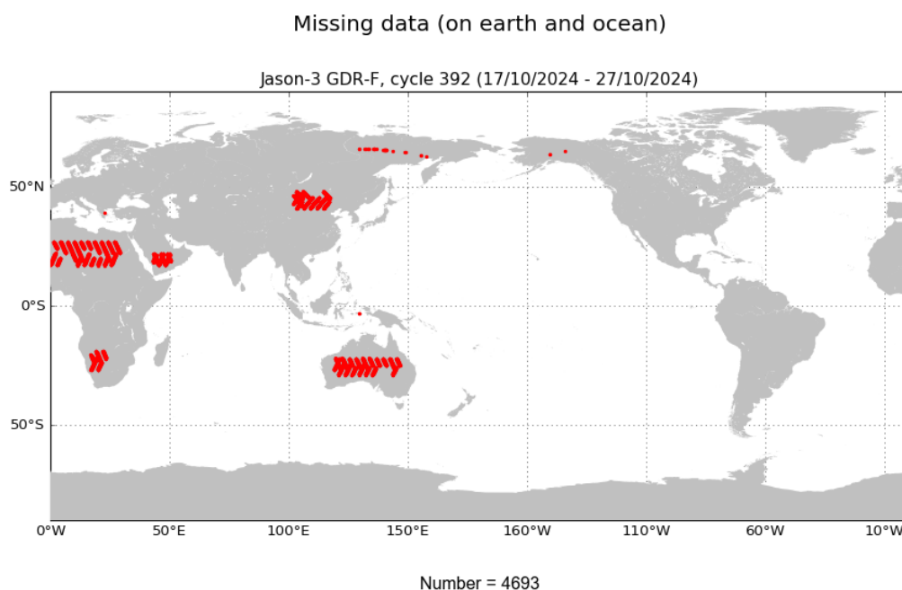
FIGURE 1 – Missing measurements for cycle 392.
