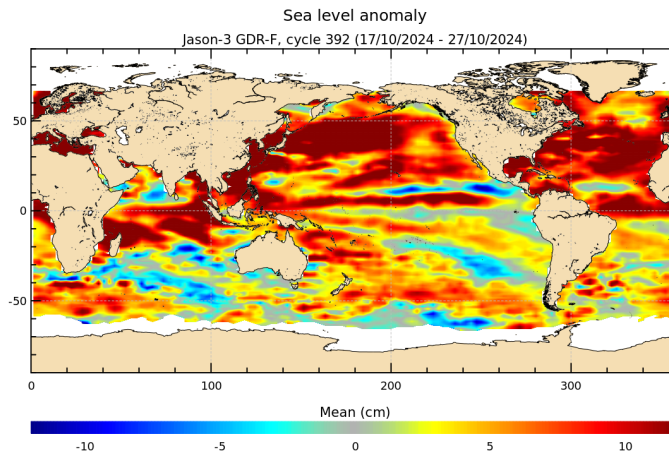
FIGURE 18 – Sea level anomaly relative to MSS for cycle 392.
