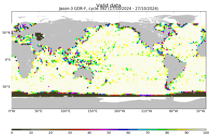
FIGURE 3 – Percentage of valid measurements for cycle 392.
