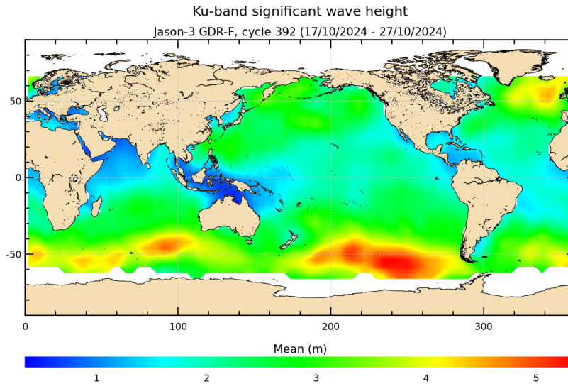
FIGURE 5 – Significant wave height for cycle 392.
