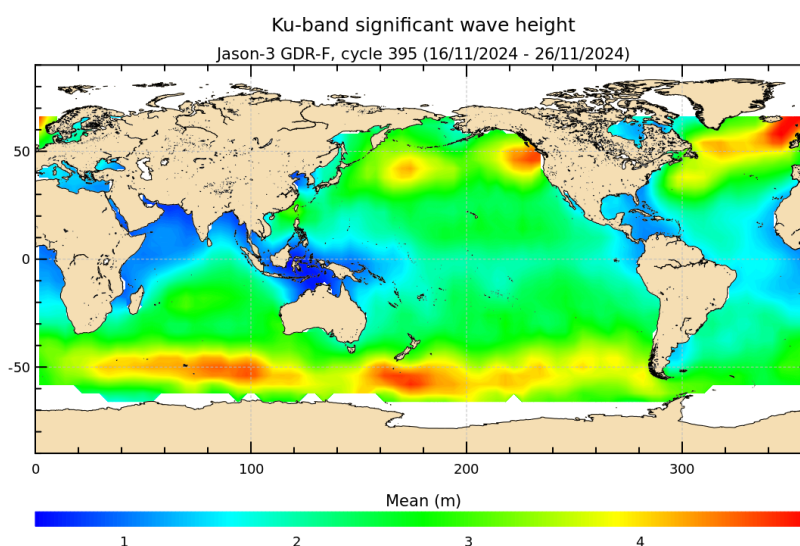
FIGURE 5 – Significant wave height for cycle 395.
