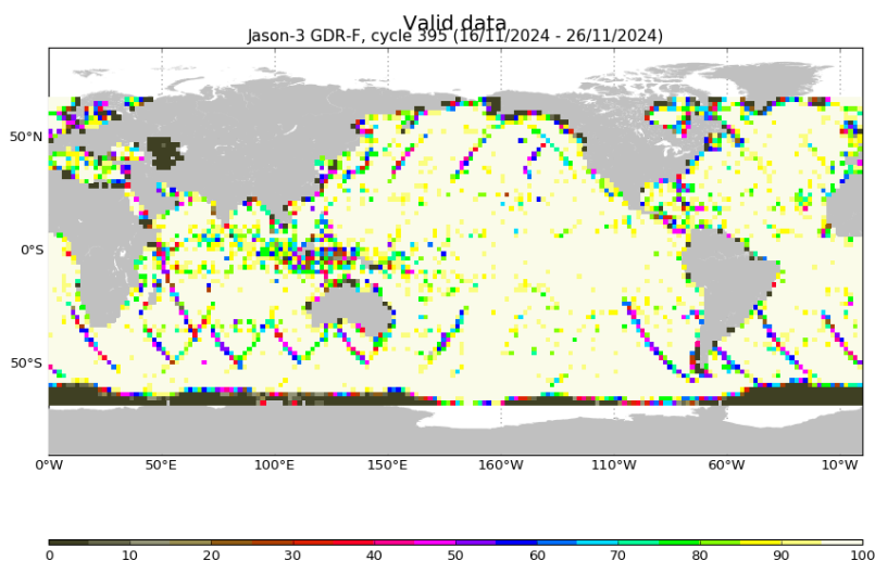
FIGURE 3 – Percentage of valid measurements for cycle 395.
