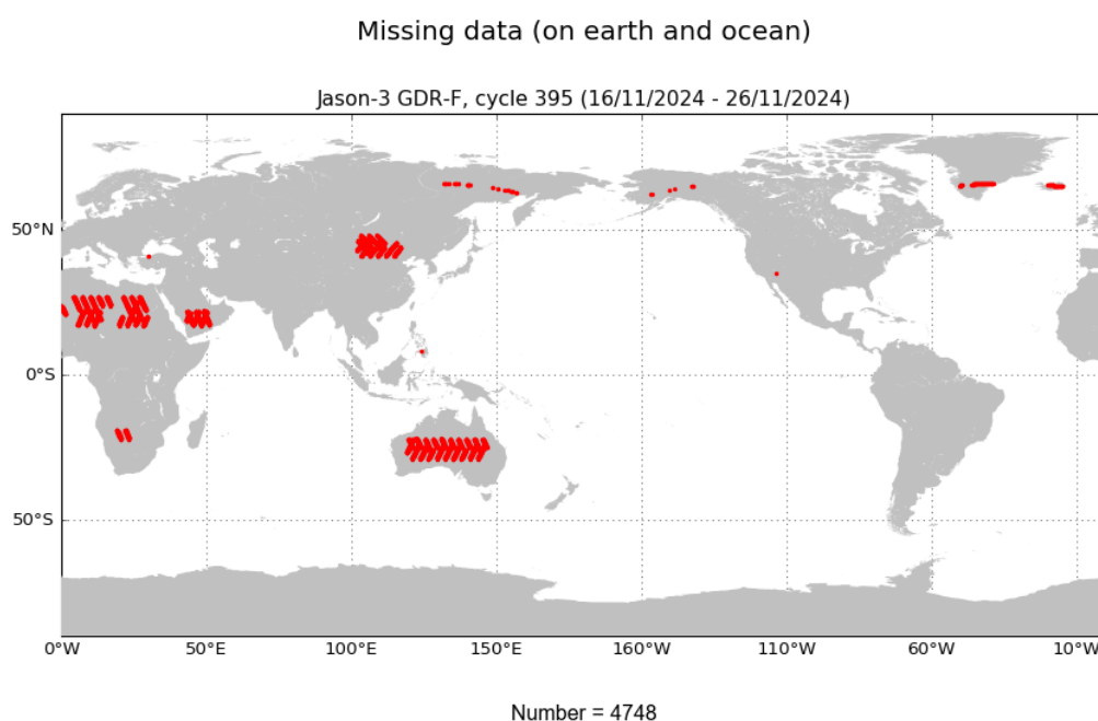
FIGURE 1 – Missing measurements for cycle 395.
