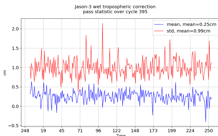
FIGURE 11 – Pass monitoring of wet troposphere differences between radiometer and ECMWF model for Jason-3 cycle 395
