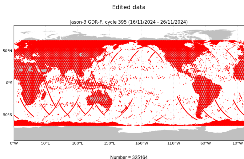
FIGURE 2 – Edited measurements for cycle 395.
