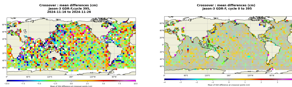
FIGURE 13 – Mean SSH at crossovers for cycle 395 (left) and over the whole Jason-3 period (right).
