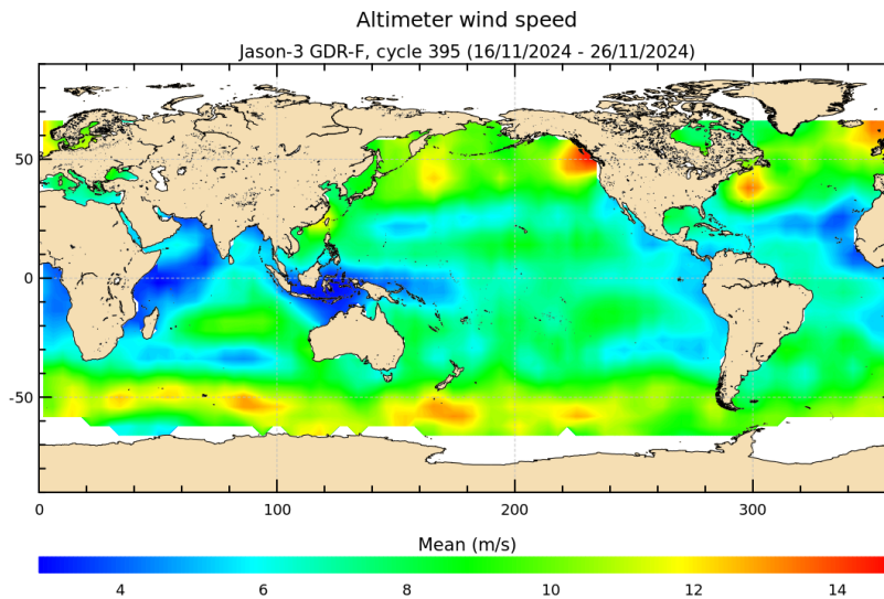
FIGURE 9 – Altimeter wind speed for cycle 395.
