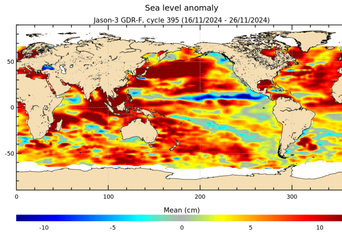
FIGURE 18 – Sea level anomaly relative to MSS for cycle 395.
