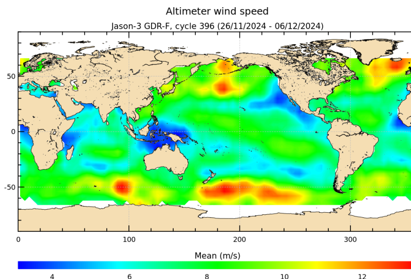
FIGURE 9 – Altimeter wind speed for cycle 396.
