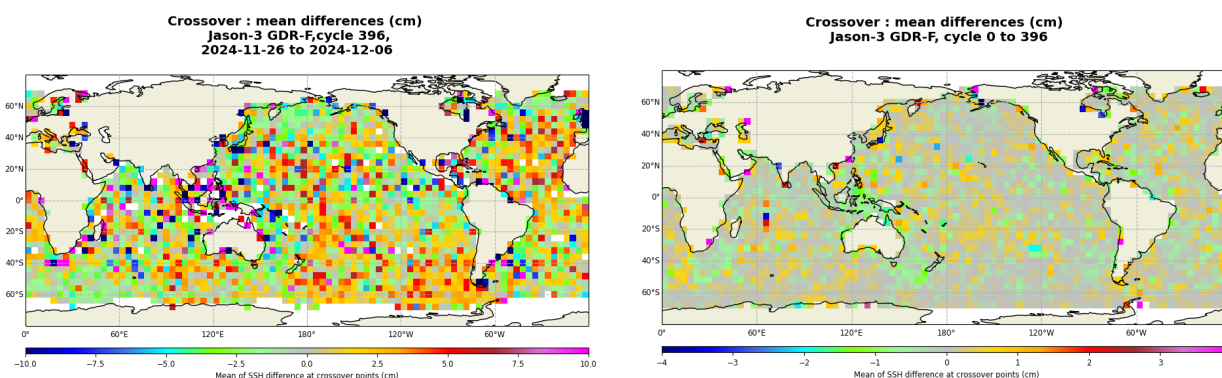
FIGURE 13 – Mean SSH at crossovers for cycle 396 (left) and over the whole Jason-3 period (right).
