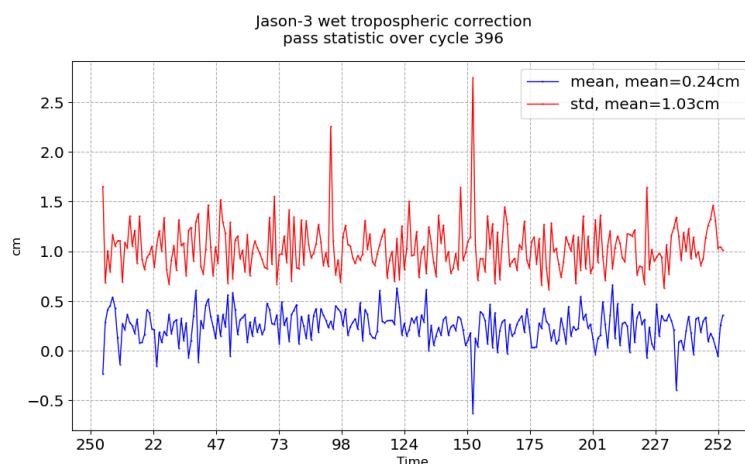
FIGURE 11 – Pass monitoring of wet troposphere differences between radiometer and ECMWF model for Jason-3 cycle 396
