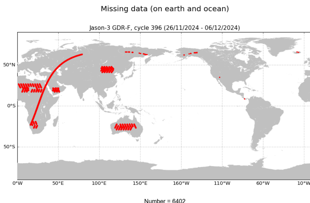
FIGURE 1 – Missing measurements for cycle 396.
