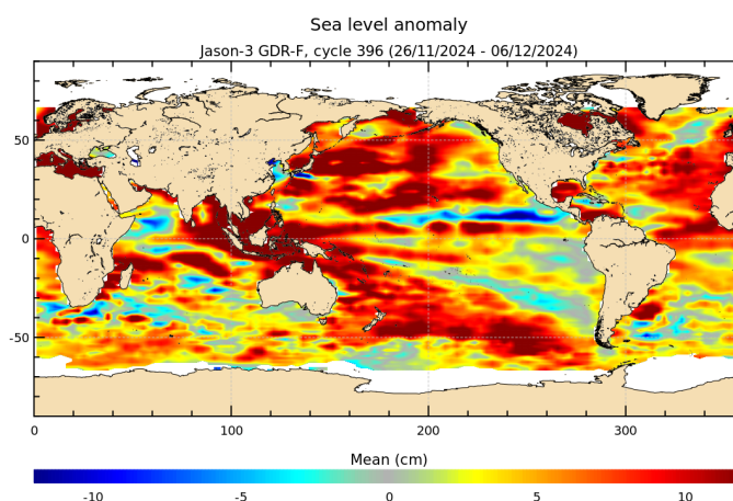
FIGURE 18 – Sea level anomaly relative to MSS for cycle 396.
