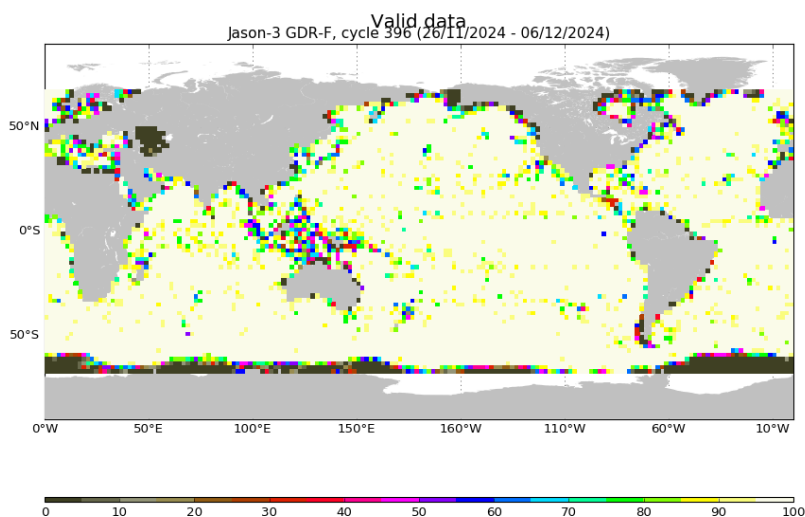
FIGURE 3 – Percentage of valid measurements for cycle 396.
