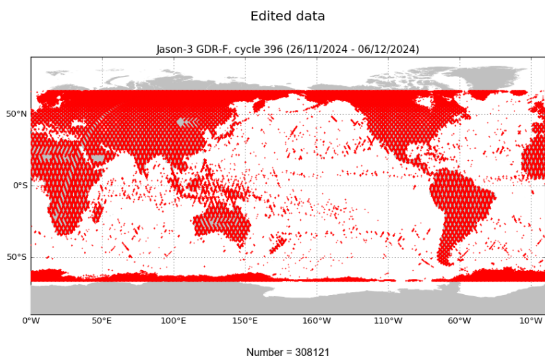
FIGURE 2 – Edited measurements for cycle 396.
