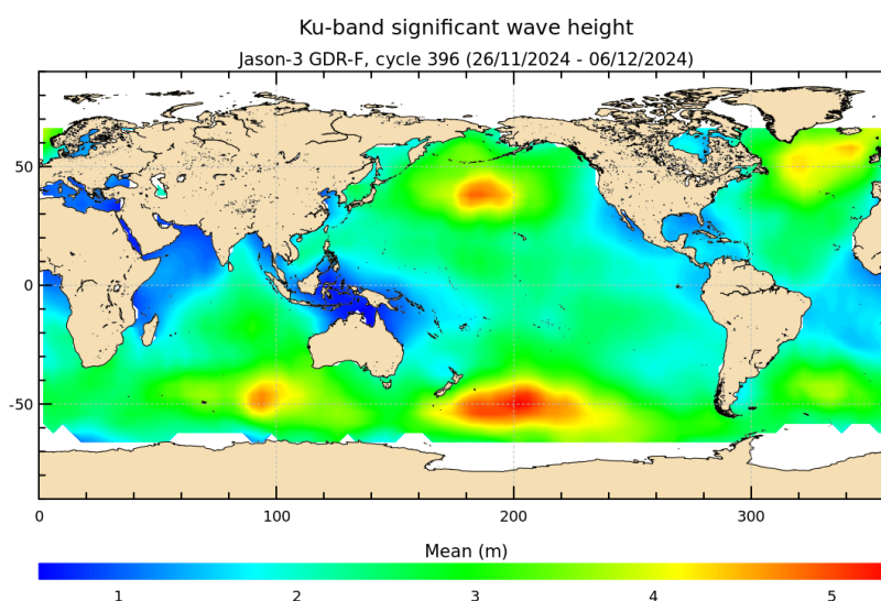
FIGURE 5 – Significant wave height for cycle 396.
