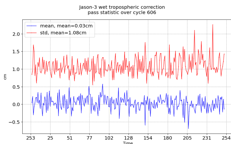
FIGURE 11 – Pass monitoring of wet troposphere differences between radiometer and ECMWF model for Jason-3 cycle 606
