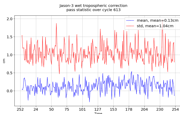
FIGURE 11 – Pass monitoring of wet troposphere differences between radiometer and ECMWF model for Jason-3 cycle 613
