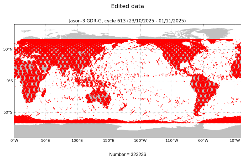
FIGURE 2 – Edited measurements for cycle 613.
