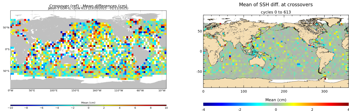
FIGURE 13 – Mean SSH at crossovers for cycle 613 (left) and over the whole Jason-3 period (right).
