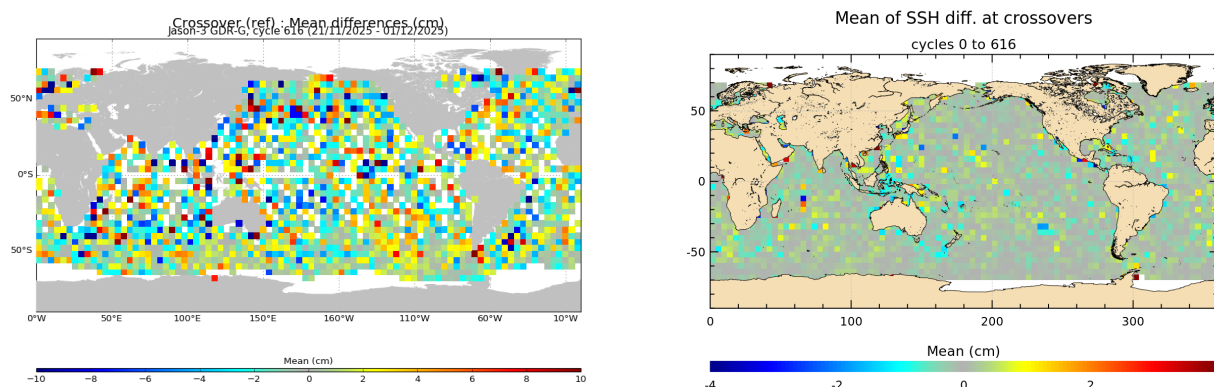
FIGURE 13 – Mean SSH at crossovers for cycle 616 (left) and over the whole Jason-3 period (right).
