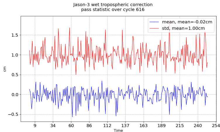
FIGURE 11 – Pass monitoring of wet troposphere differences between radiometer and ECMWF model for Jason-3 cycle 616
