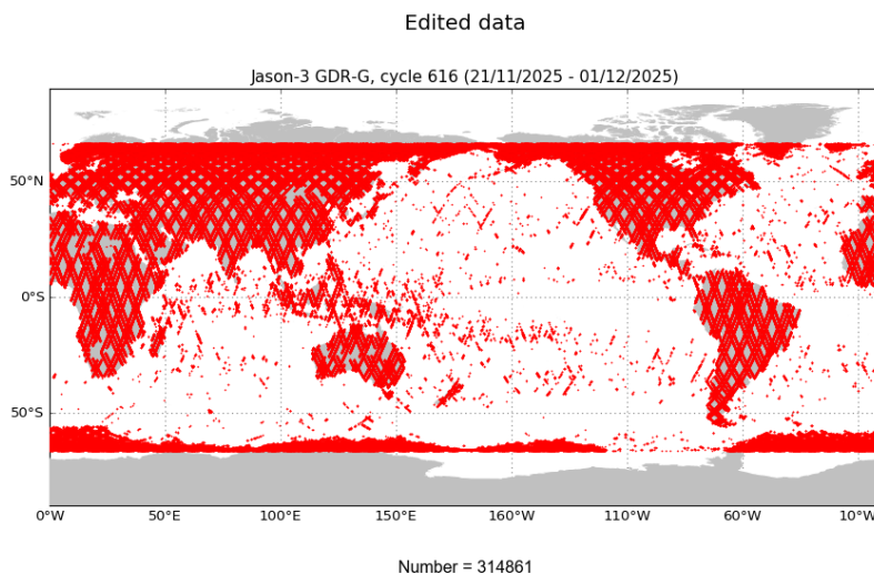
FIGURE 2 – Edited measurements for cycle 616.
