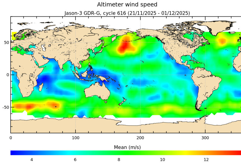
FIGURE 9 – Altimeter wind speed for cycle 616.
