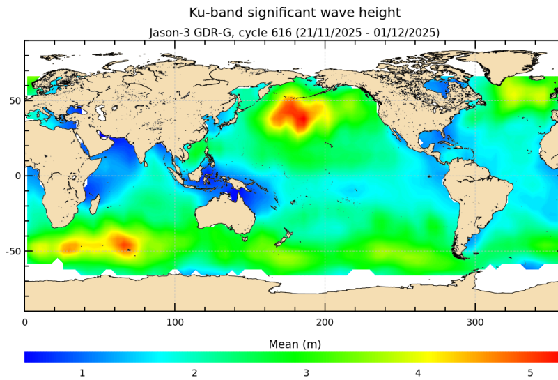
FIGURE 5 – Significant wave height for cycle 616.
