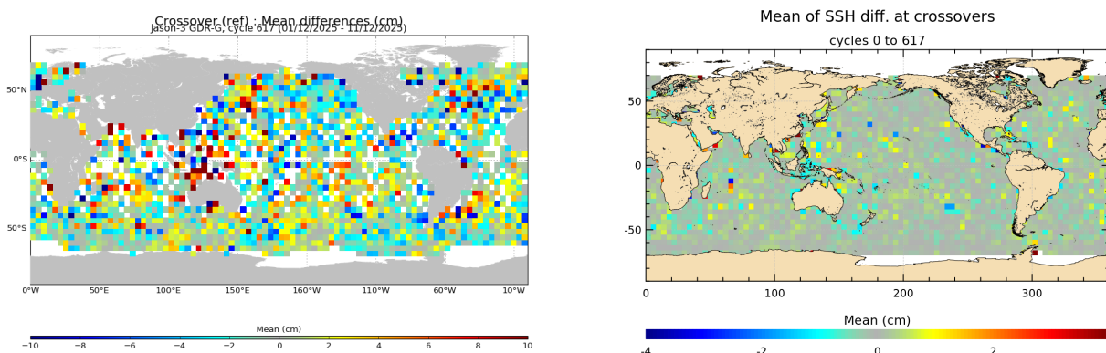
FIGURE 13 – Mean SSH at crossovers for cycle 617 (left) and over the whole Jason-3 period (right).
