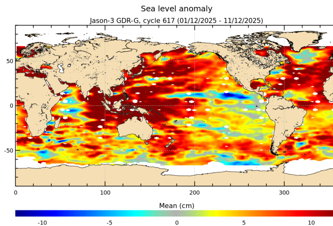
FIGURE 18 – Sea level anomaly relative to MSS for cycle 617.
