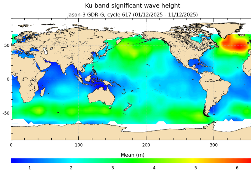
FIGURE 5 – Significant wave height for cycle 617.
