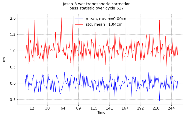
FIGURE 11 – Pass monitoring of wet troposphere differences between radiometer and ECMWF model for Jason-3 cycle 617
