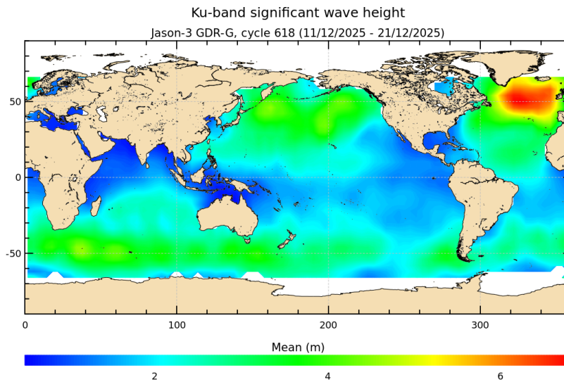
FIGURE 5 – Significant wave height for cycle 618.
