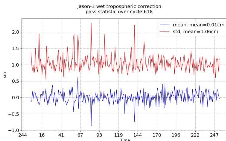
FIGURE 11 – Pass monitoring of wet troposphere differences between radiometer and ECMWF model for Jason-3 cycle 618
