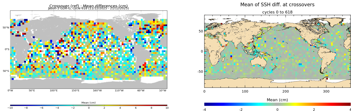
FIGURE 13 – Mean SSH at crossovers for cycle 618 (left) and over the whole Jason-3 period (right).
