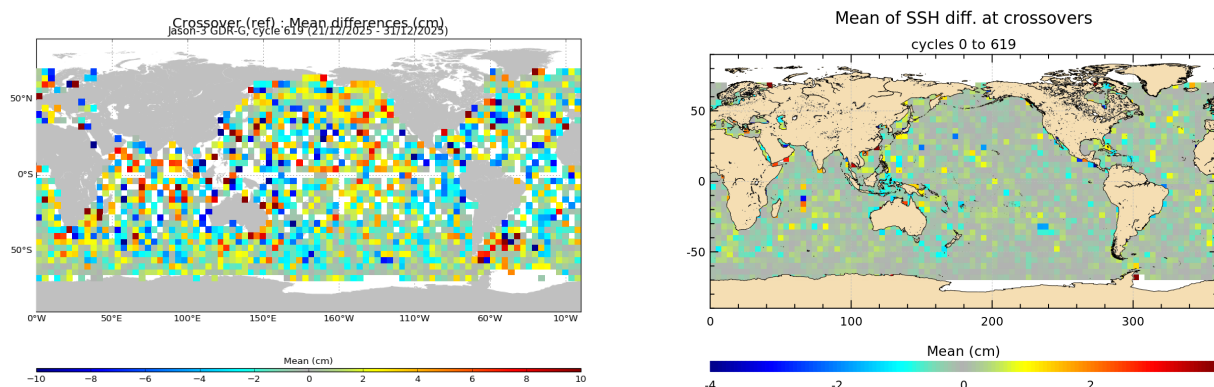
FIGURE 13 – Mean SSH at crossovers for cycle 619 (left) and over the whole Jason-3 period (right).
