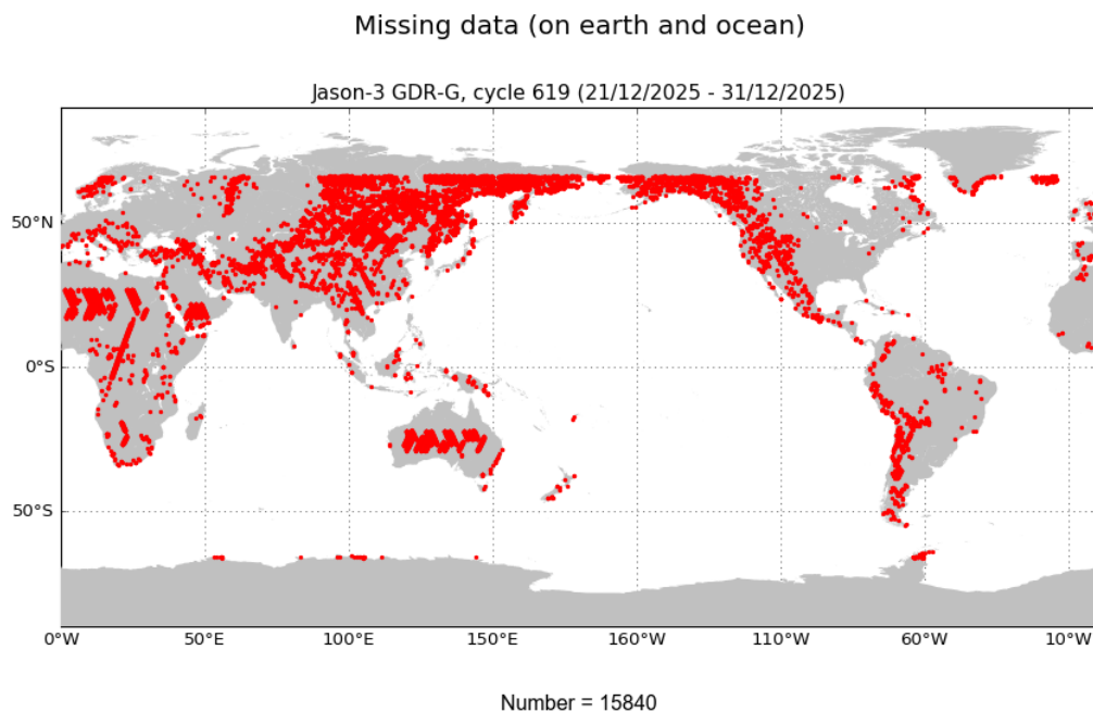
FIGURE 1 – Missing measurements for cycle 619.
