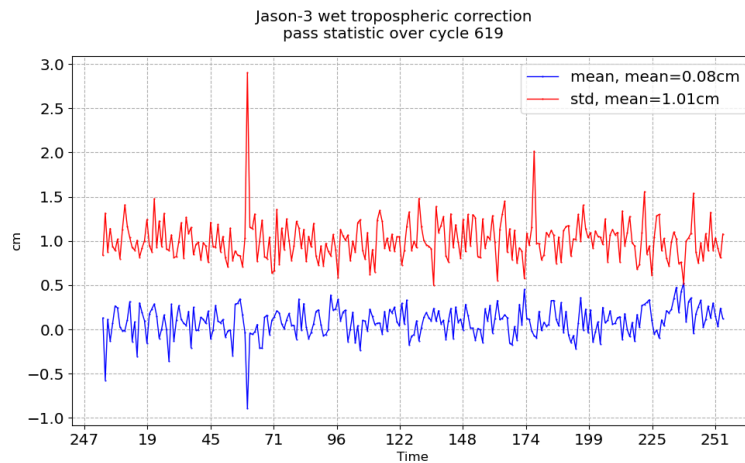
FIGURE 11 – Pass monitoring of wet troposphere differences between radiometer and ECMWF model for Jason-3 cycle 619
