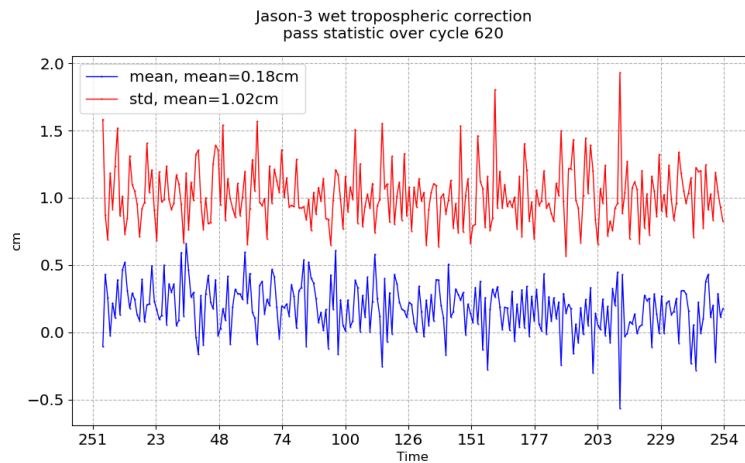
FIGURE 11 – Pass monitoring of wet troposphere differences between radiometer and ECMWF model for Jason-3 cycle 620
