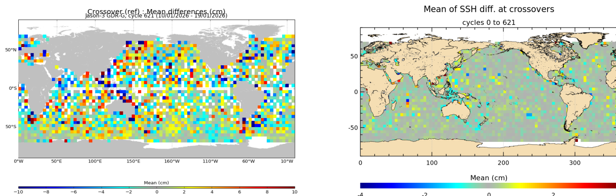
FIGURE 13 – Mean SSH at crossovers for cycle 621 (left) and over the whole Jason-3 period (right).
