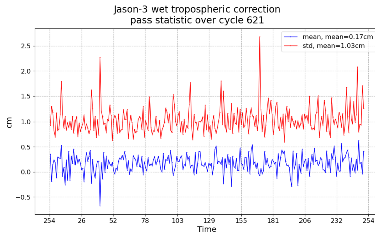
FIGURE 11 – Pass monitoring of wet troposphere differences between radiometer and ECMWF model for Jason-3 cycle 621
