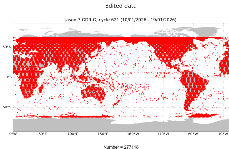
FIGURE 2 – Edited measurements for cycle 621.
