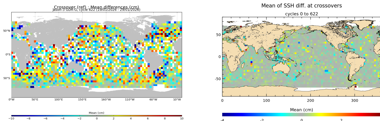
FIGURE 13 – Mean SSH at crossovers for cycle 622 (left) and over the whole Jason-3 period (right).
