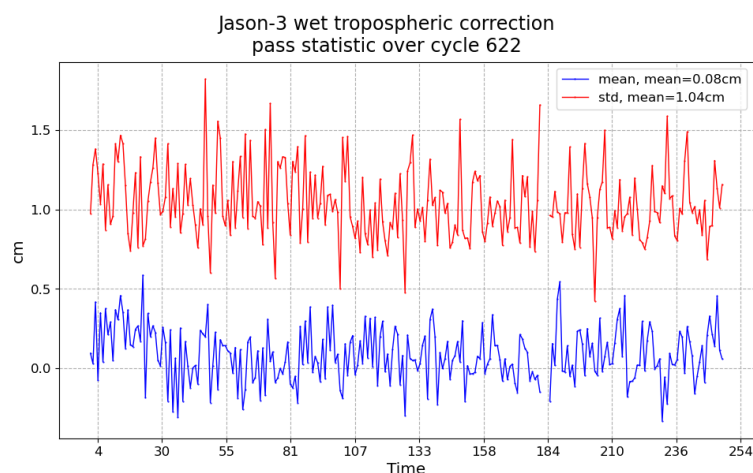
FIGURE 11 – Pass monitoring of wet troposphere differences between radiometer and ECMWF model for Jason-3 cycle 622
