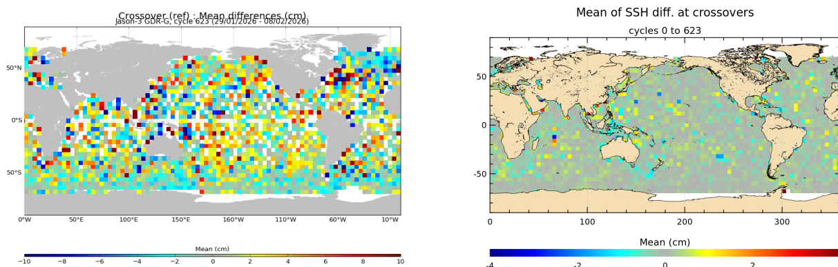
FIGURE 13 – Mean SSH at crossovers for cycle 623 (left) and over the whole Jason-3 period (right).
