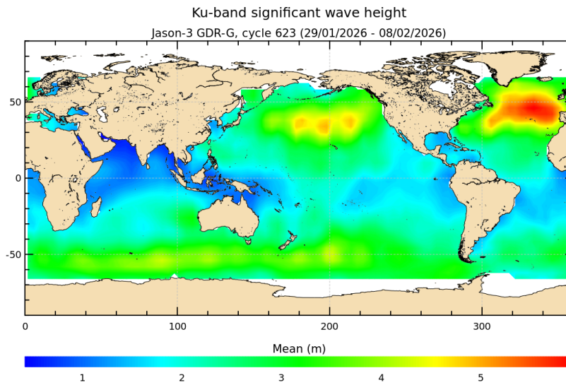
FIGURE 5 – Significant wave height for cycle 623.
