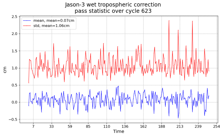
FIGURE 11 – Pass monitoring of wet troposphere differences between radiometer and ECMWF model for Jason-3 cycle 623
