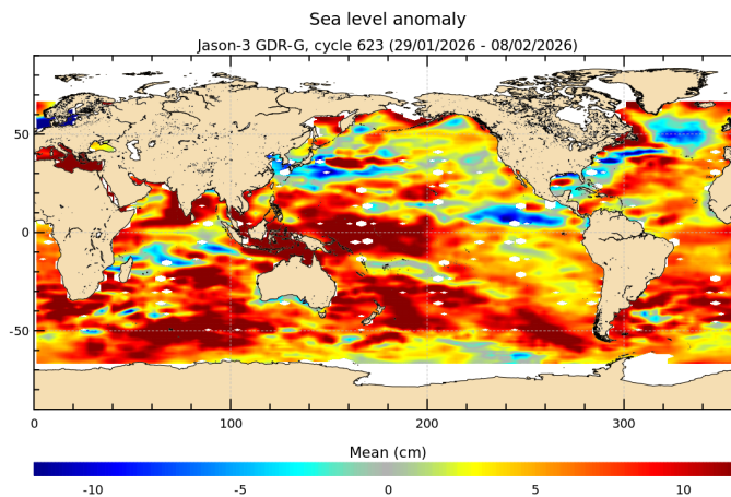
FIGURE 18 – Sea level anomaly relative to MSS for cycle 623.
