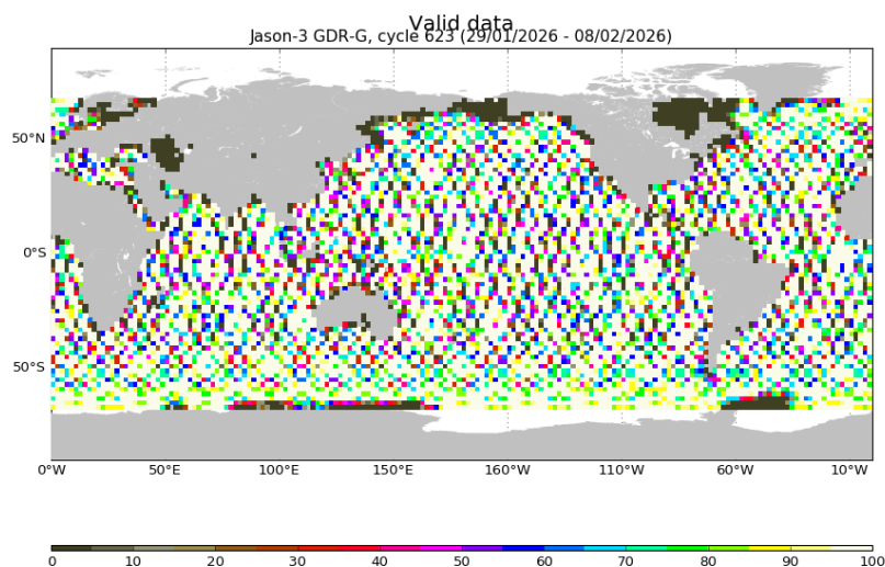
FIGURE 3 – Percentage of valid measurements for cycle 623.
