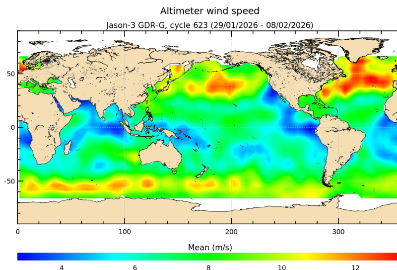
FIGURE 9 – Altimeter wind speed for cycle 623.
