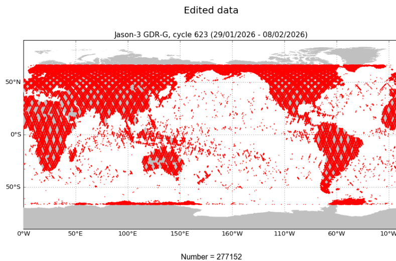
FIGURE 2 – Edited measurements for cycle 623.
