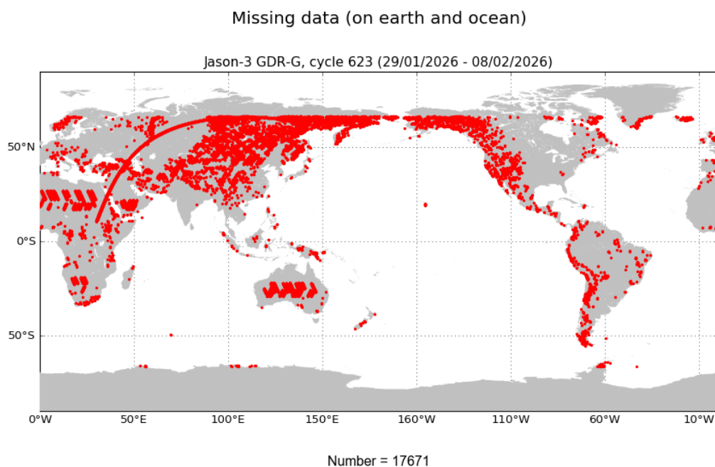
FIGURE 1 – Missing measurements for cycle 623.
