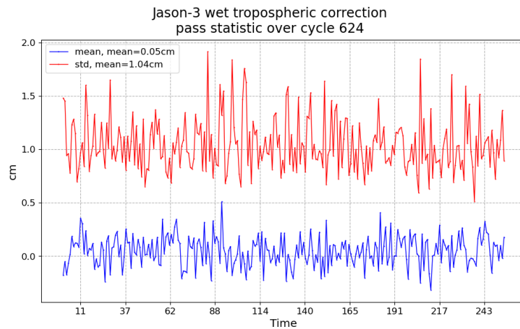
FIGURE 11 – Pass monitoring of wet troposphere differences between radiometer and ECMWF model for Jason-3 cycle 624
