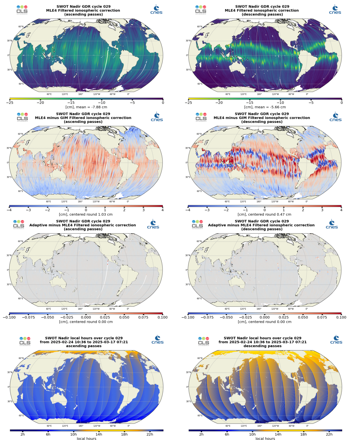
Figure 14: Along-track maps of filtered ionosphere correction over cycle 029 for SWOT Nadir MLE4 (top), MLE4 minus GIM (middle top) or Adaptive minus MLE4 (middle bottom), and local hours (bottom), for ascending passes (left) and descending passes (right)
