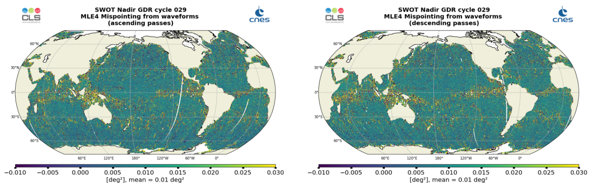
Figure 17: Along-track maps of mispointing over cycle 029 for SWOT Nadir MLE4, ascending passes (left) and descending passes (right)
