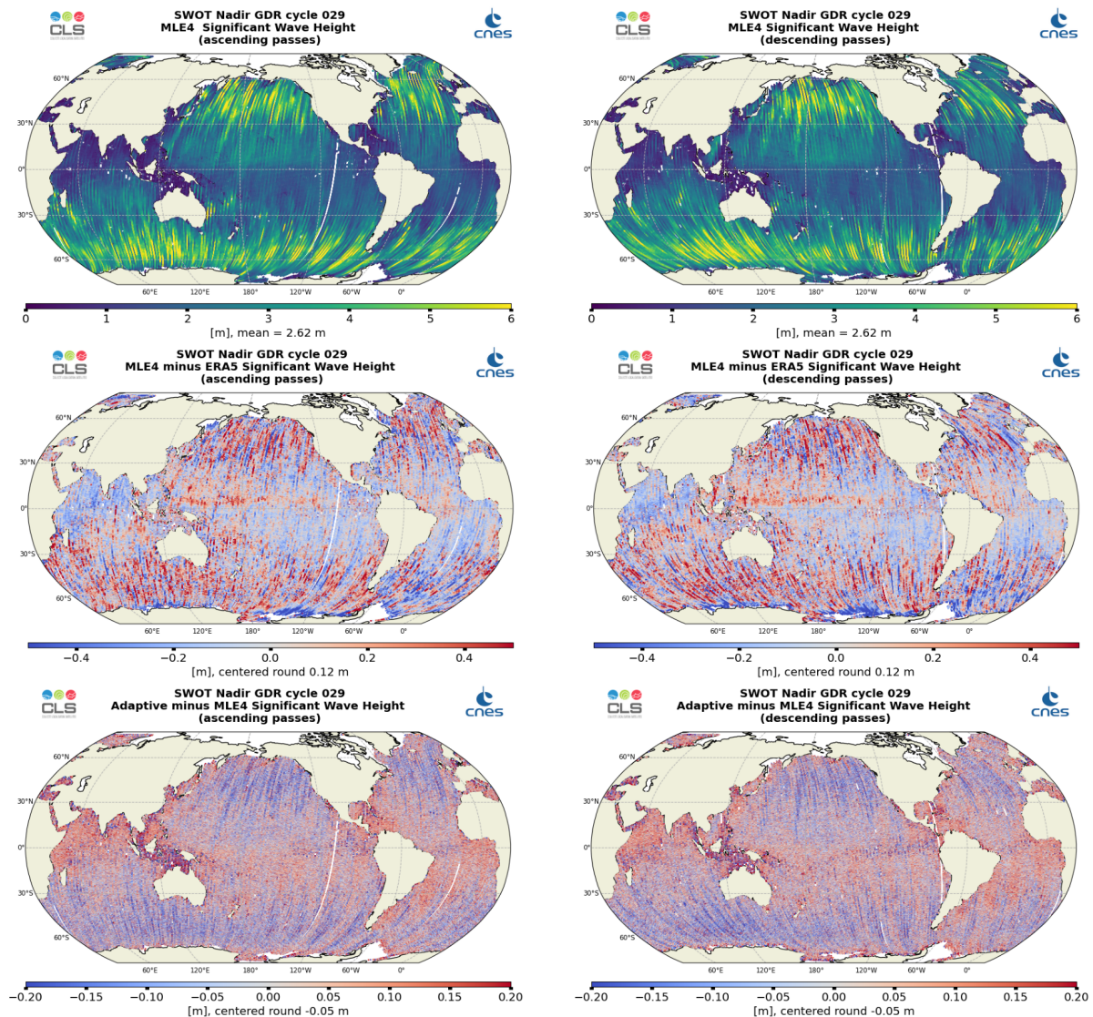
Figure 5: Along-track maps of Ku-band Significant Wave Height over cycle 029 for SWOT Nadir MLE4 (top), MLE4 minus model (middle) or Adaptive minus MLE4 (bottom), ascending passes (left) and descending passes (right)
