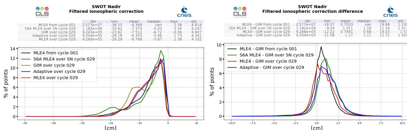
Figure 13: GIM model (dark green) and altimeter filtered ionosphere correction histogram computed over cycle 029 (red line for SWOT Nadir MLE4 and blue line for SWOT Nadir Adaptive, green for Sentinel-6A-MF (LR MLE4)) and from cycle 001 (SWOT Nadir, MLE4 only, black line) (left). Difference between filtered altimeter and GIM model (right).
