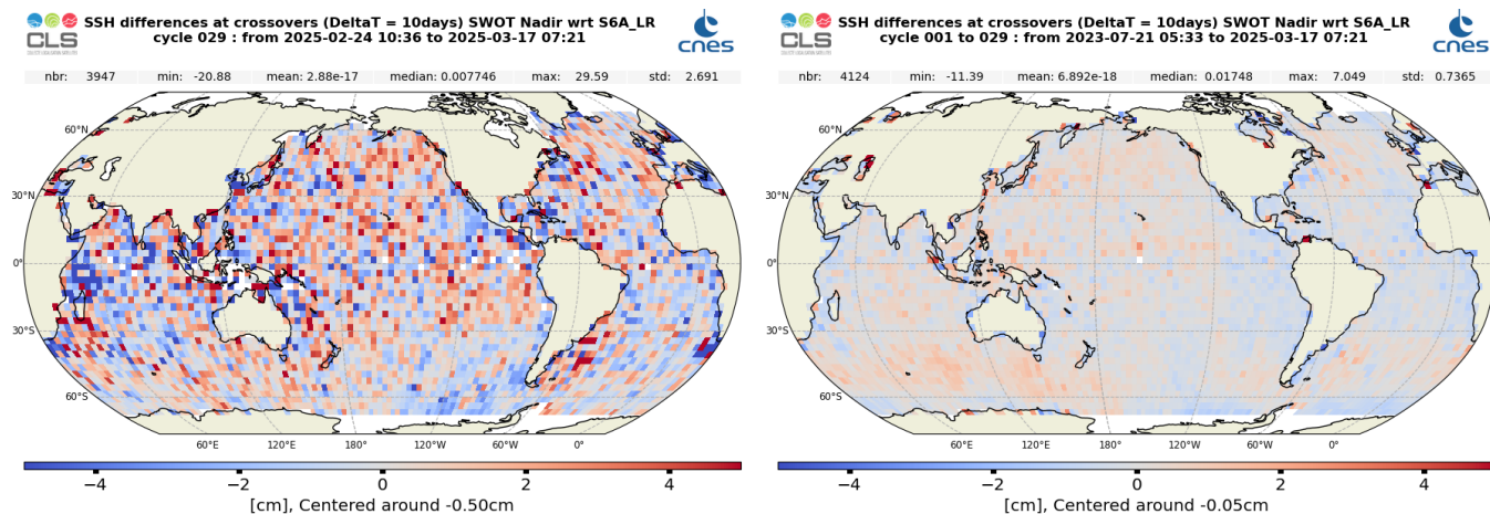
Figure 30: Mean SSH difference at crossovers between SWOT Nadir MLE4 and Sentinel-6 MF LR MLE4 over cycle 029 (left) and from cycle 001 onwards (right)
