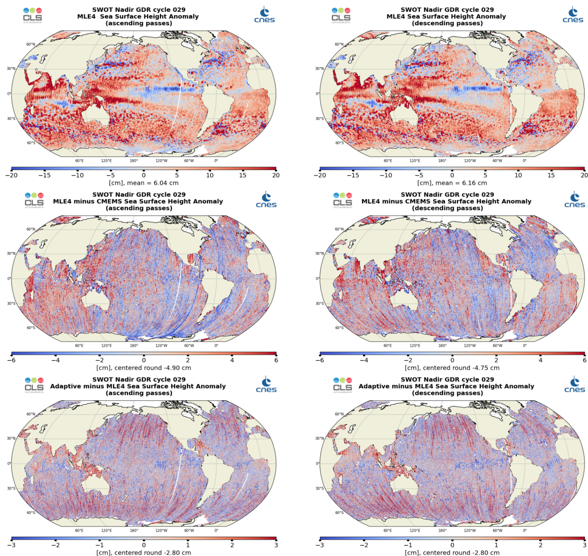
Figure 26: Along-track maps of SSHA over cycle 029 for SWOT Nadir MLE4 (top), MLE4 minus CMEMS (middle) or Adaptive minus MLE4 (bottom), ascending passes (left) and descending passes (right)
