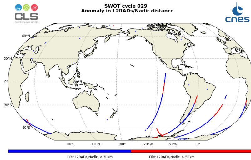
Figure 24: Map of the anomalies detected in the L2RADs/Nadir distance over the cycle 029
