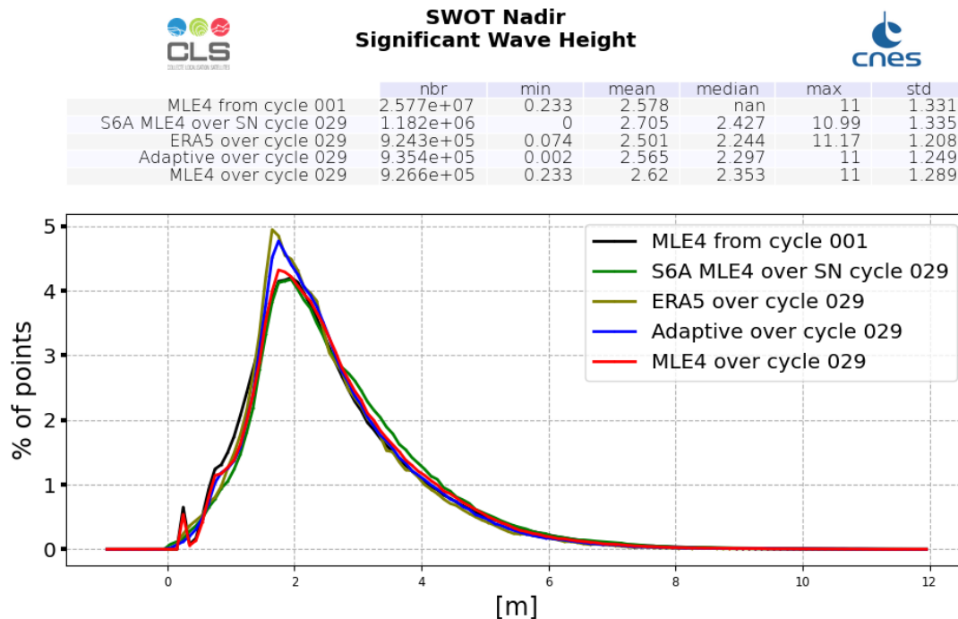
Figure 4: Ku-band Significant Wave Height histogram computed over cycle 029 (red line for SWOT Nadir MLE4 and blue line for SWOT Nadir Adaptive, green for Sentinel-6A-MF (LR MLE4) and dark green for ERA5) and from cycle 001 (SWOT Nadir, MLE4 only, black line)
