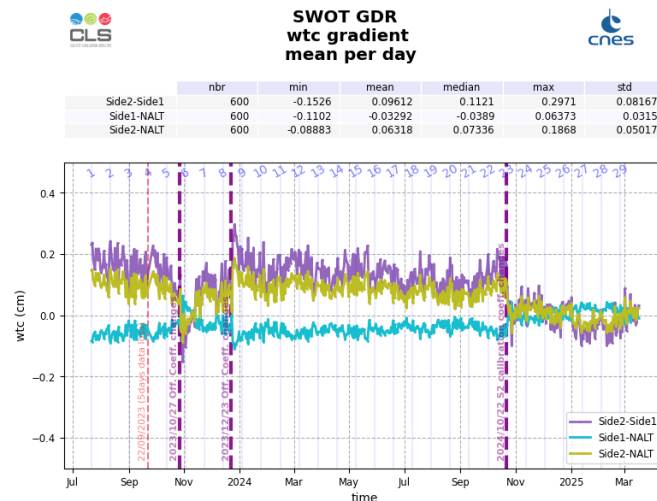
Figure 20: Daily monitoring of the wet tropospheric correction gradient between AMR Side 1 and AMR Side 2 (purple), AMR Side 1 and Nadir (cyan), and AMR Side 2 and Nadir (yellow), from Cycle 001 to 029
