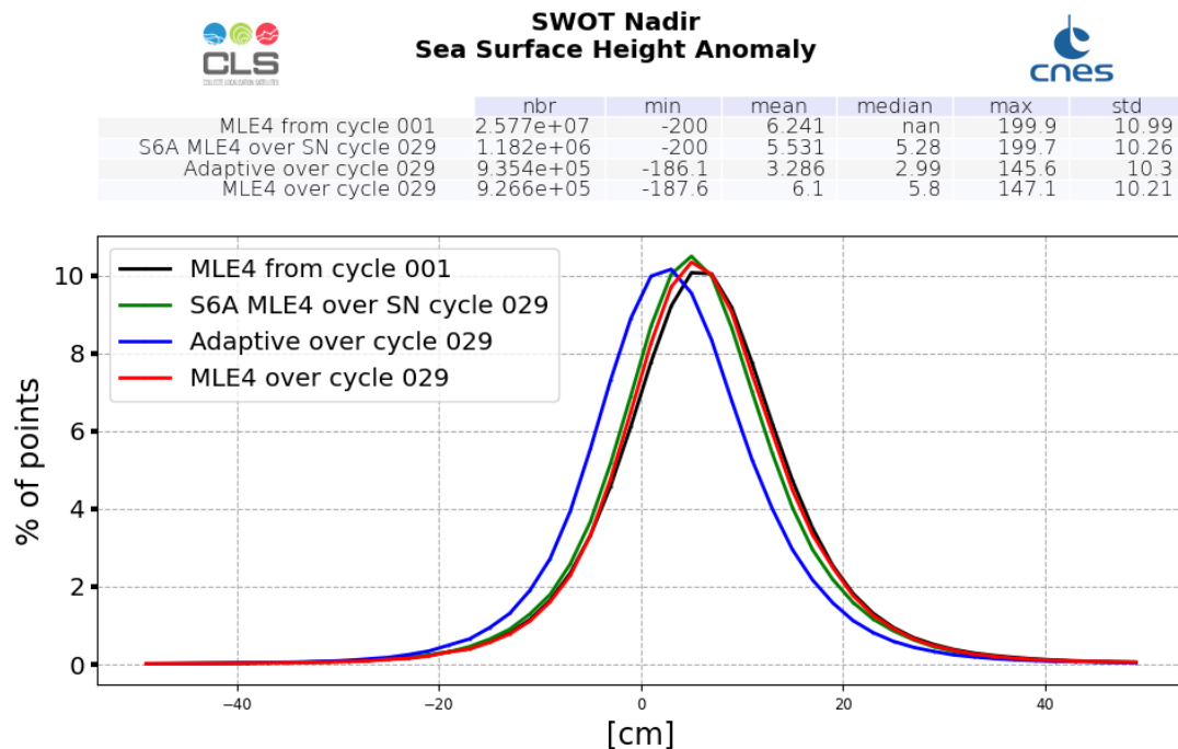
Figure 25: SSHA histogram computed over cycle 029 (red line for SWOT Nadir MLE4 and blue line for SWOT Nadir Adaptive, green for Sentinel-6A-MF (LR MLE4)) and from cycle 001 (SWOT Nadir, MLE4 only, black line)
