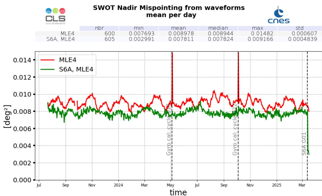
Figure 18: Mispointing daily monitoring from SWOT cycle 001 to 029 for SWOT Nadir GDR (red) and Sentinel-6A-MF (green)
