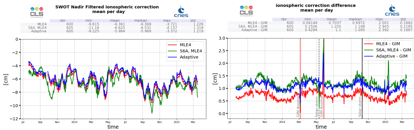
Figure 15: SWOT Nadir MLE4 (red), Adaptive (blue) and Sentinel-6A-MF (LR MLE4) (green) filtered ionosphere correction daily monitoring from cycle 001 to 029 (left) and difference with GIM model (right)
