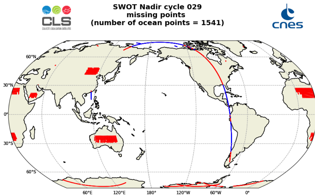
Figure 1: Map of missing measurements for SWOT Nadir GDR cycle 029
