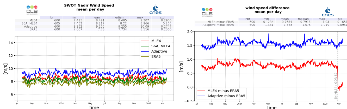
Figure 12: Wind Speed daily monitoring from cycle 001 to 029 for SWOT Nadir GDR, ERA5 model, and Sentinel-6A-MF (LR MLE4) (left), and daily mean difference with ERA5 (right)
