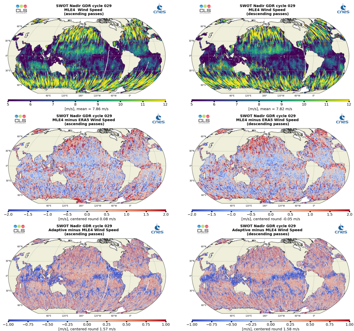
Figure 11: Along-track maps of Altimeter Wind Speed over cycle 029 for SWOT Nadir MLE4 (top), MLE4 minus ERA5 (middle) or Adaptive minus MLE4 (bottom), ascending passes (left) and descending passes (right)
