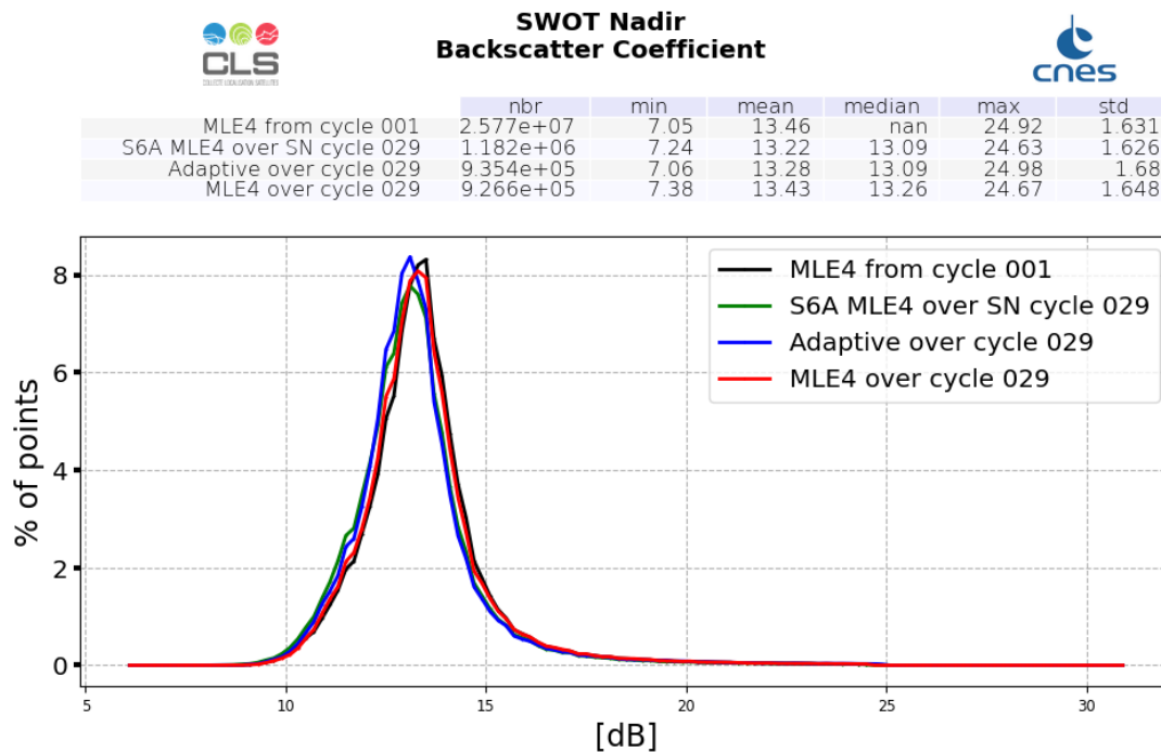
Figure 7: Ku-band Backscattering coefficient histogram computed over cycle 029 (red line for SWOT Nadir MLE4 and blue line for SWOT Nadir Adaptive, green for Sentinel-6A-MF (LR MLE4)) and from cycle 001 (SWOT Nadir, MLE4 only, black line)
