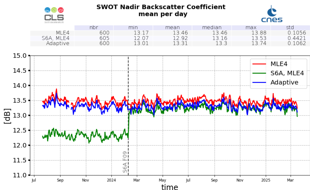
Figure 9: Ku-band Backscattering coefficient daily monitoring from cycle 001 to 029, for SWOT Nadir and Sentinel-6A-MF
