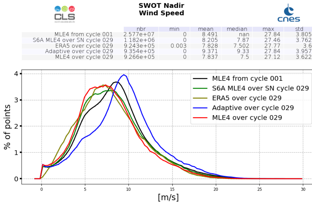
Figure 10: Altimeter Wind Speed histogram computed over cycle 029 (red line for SWOT Nadir MLE4 and blue line for SWOT Nadir Adaptive, green for Sentinel-6A-MF (LR MLE4)) and from cycle 001 (SWOT Nadir, MLE4 only, black line)
