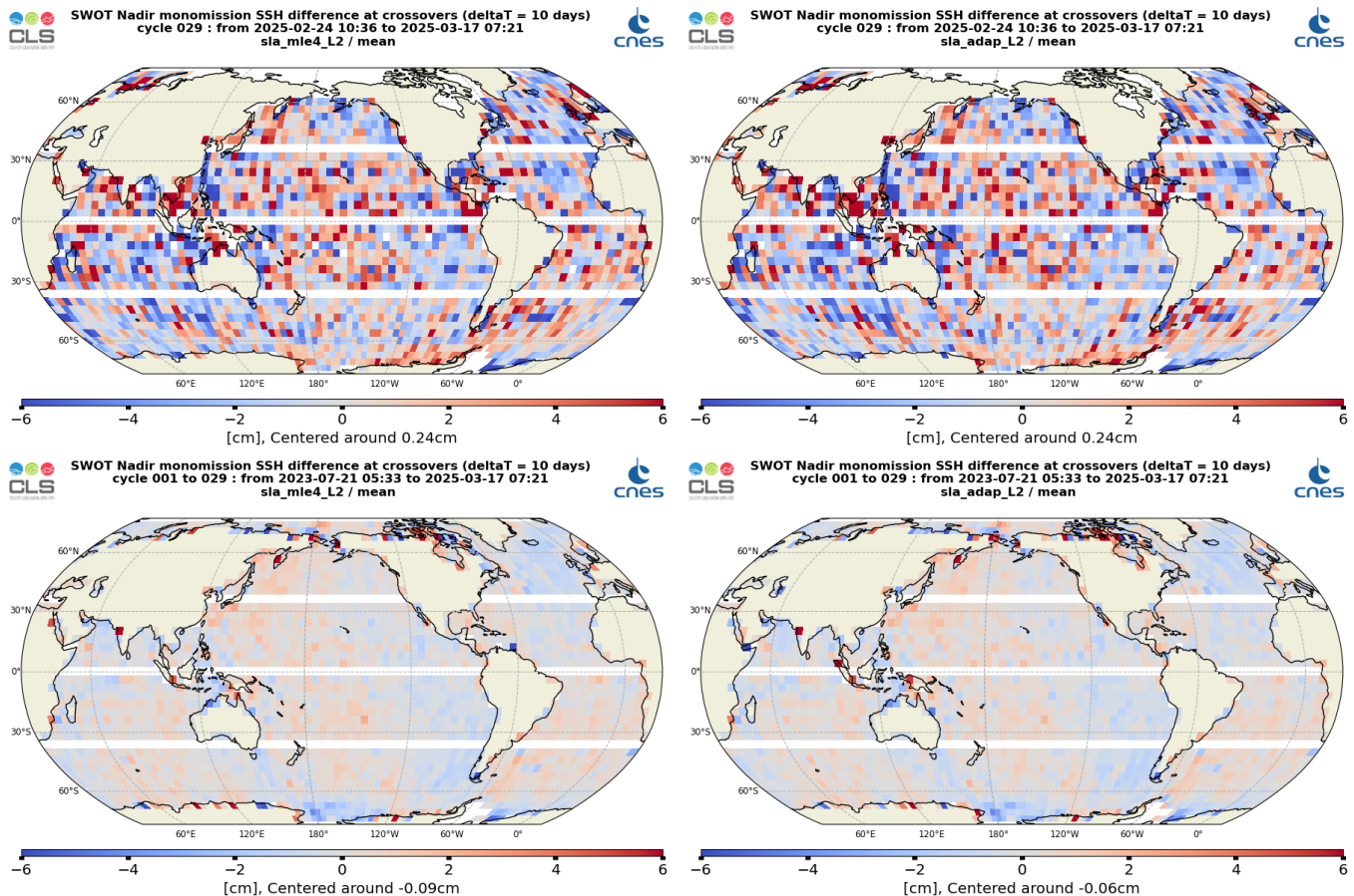
Figure 28: Mean SSH difference at crossovers for SWOT Nadir MLE4 (left) and Adaptive (right) cycle 029(top) and from cycle 001 to cycle 029 (bottom)
