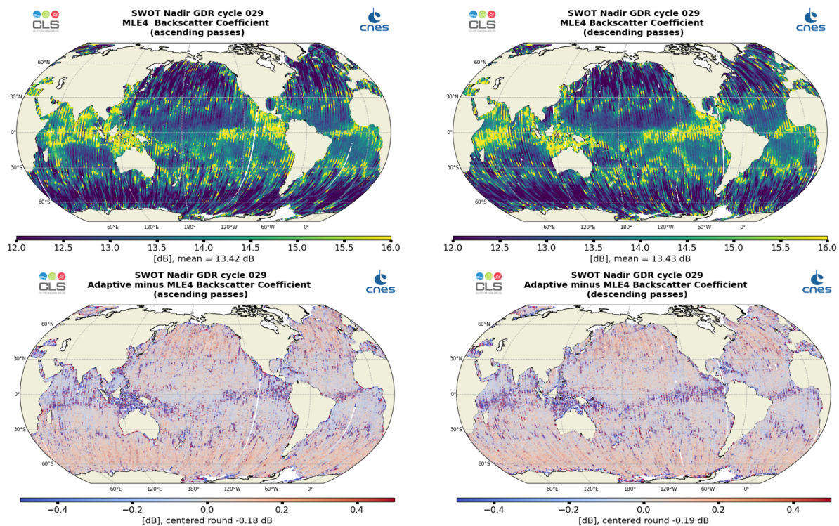
Figure 8: Along-track maps of Ku-band backscatter coefficient \sigma_0 over cycle 029 for SWOT Nadir MLE4 (top) or Adaptive minus MLE4 difference (bottom), ascending passes (left) and descending passes (right)
