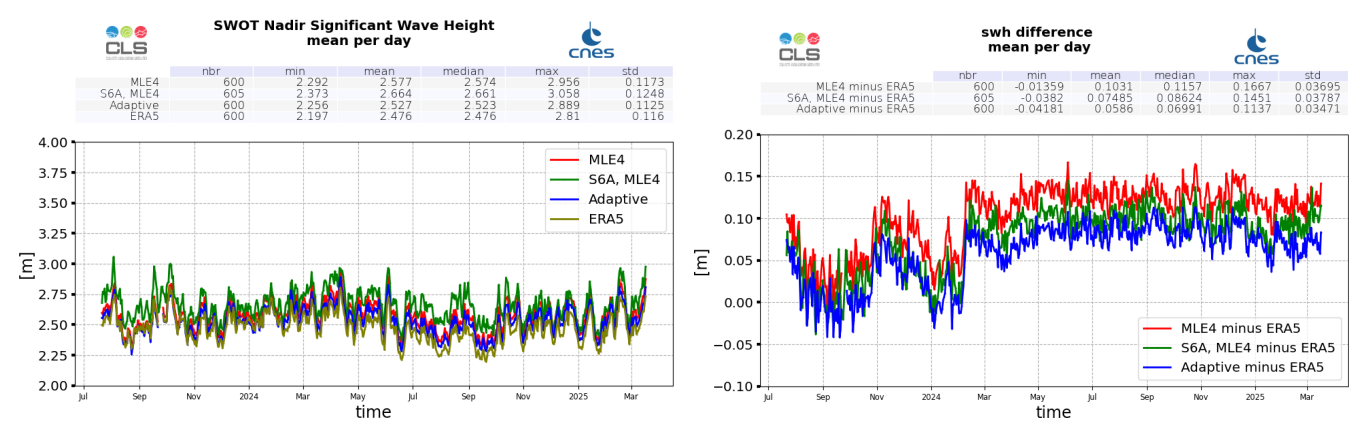
Figure 6: Ku-band Significant Wave Height daily monitoring from cycle 001 to 029, for SWOT Nadir, ERA5 model estimated at SWOT locations, and Sentinel-6A-MF (LR MLE4) (left), and difference with ERA5 model (right)
