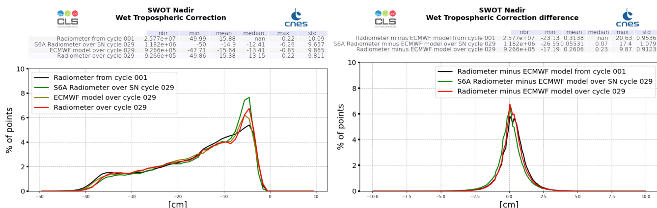
Figure 21: Histogram of wet troposphere corrections : SWOT Nadir radiometer (left) and difference with ECMWF model (right), computed over cycle 029 and from cycle 001 (black line)
