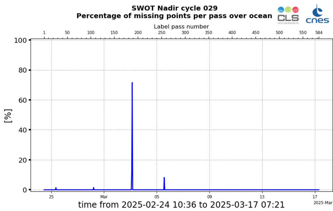
Figure 2: Monitoring of the percentage per pass of missing data over ocean, for SWOT Nadir GDR cycle 029
