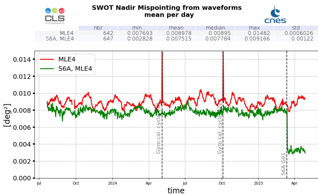
Figure 18: Mispointing daily monitoring from SWOT cycle 001 to 031 for SWOT Nadir GDR (red) and Sentinel-6A-MF (green)
