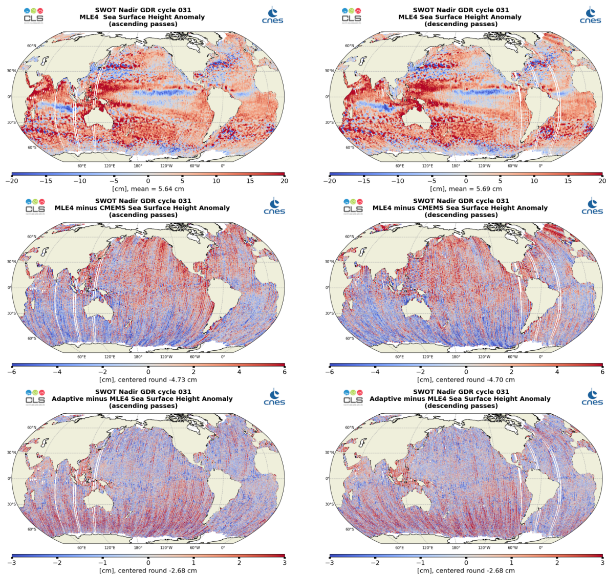
Figure 26: Along-track maps of SSHA over cycle 031 for SWOT Nadir MLE4 (top), MLE4 minus CMEMS (middle) or Adaptive minus MLE4 (bottom), ascending passes (left) and descending passes (right)
