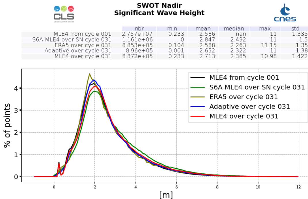
Figure 4: Ku-band Significant Wave Height histogram computed over cycle 031 (red line for SWOT Nadir MLE4 and blue line for SWOT Nadir Adaptive, green for Sentinel-6A-MF (LR MLE4) and dark green for ERA5) and from cycle 001 (SWOT Nadir, MLE4 only, black line)
