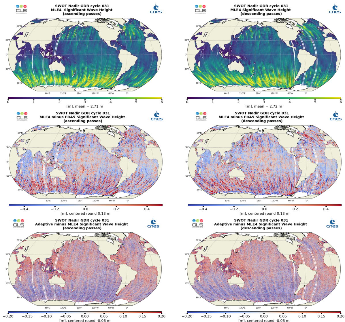
Figure 5: Along-track maps of Ku-band Significant Wave Height over cycle 031 for SWOT Nadir MLE4 (top), MLE4 minus model (middle) or Adaptive minus MLE4 (bottom), ascending passes (left) and descending passes (right)
