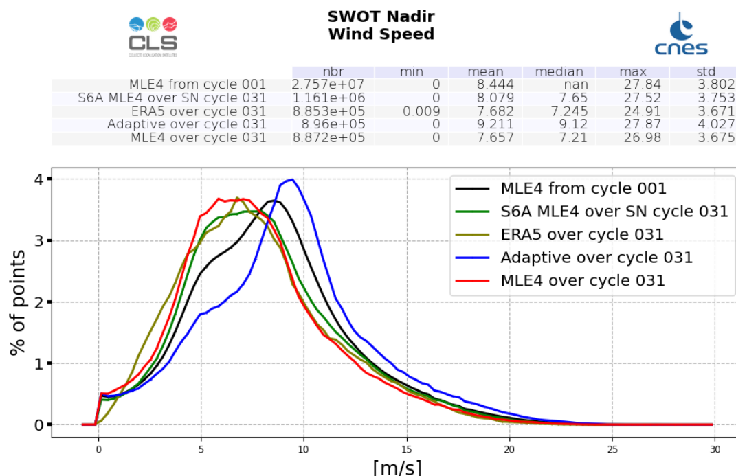
Figure 10: Altimeter Wind Speed histogram computed over cycle 031 (red line for SWOT Nadir MLE4 and blue line for SWOT Nadir Adaptive, green for Sentinel-6A-MF (LR MLE4)) and from cycle 001 (SWOT Nadir, MLE4 only, black line)
