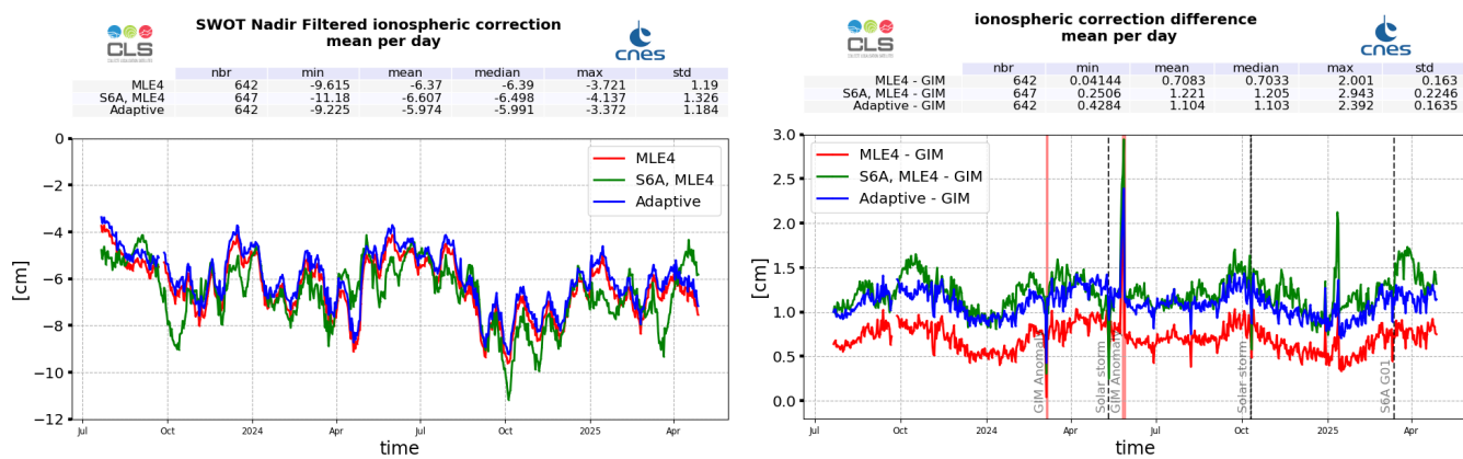
Figure 15: SWOT Nadir MLE4 (red), Adaptive (blue) and Sentinel-6A-MF (LR MLE4) (green) filtered ionosphere correction daily monitoring from cycle 001 to 031 (left) and difference with GIM model (right)
