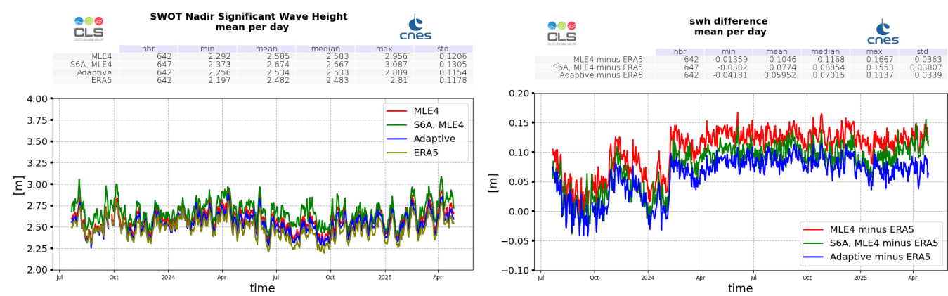
Figure 6: Ku-band Significant Wave Height daily monitoring from cycle 001 to 031, for SWOT Nadir, ERA5 model estimated at SWOT locations, and Sentinel-6A-MF (LR MLE4) (left), and difference with ERA5 model (right)
