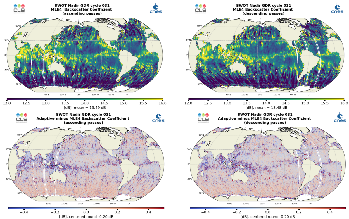
Figure 8: Along-track maps of Ku-band backscatter coefficient \sigma_0 over cycle 031 for SWOT Nadir MLE4 (top) or Adaptive minus MLE4 difference (bottom), ascending passes (left) and descending passes (right)
