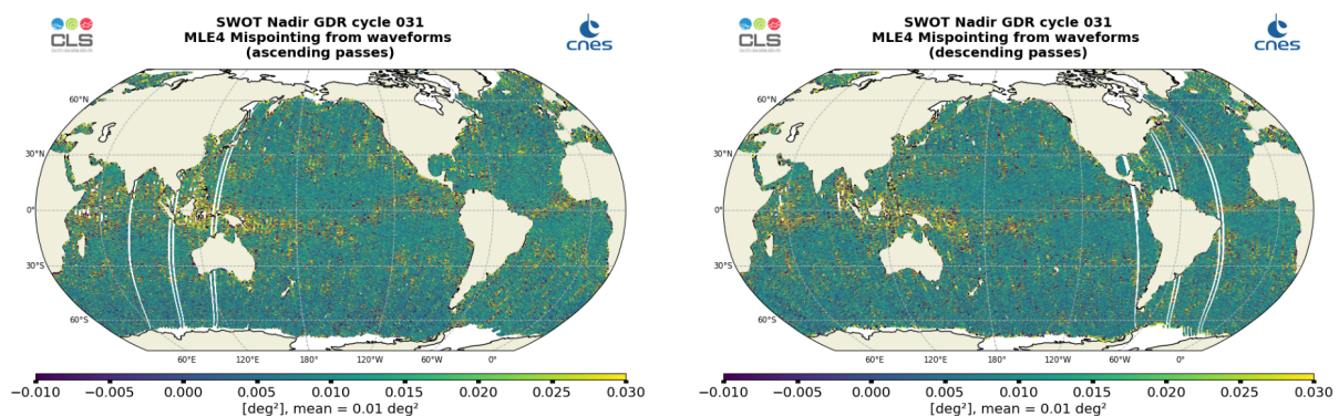
Figure 17: Along-track maps of mispointing over cycle 031 for SWOT Nadir MLE4, ascending passes (left) and descending passes (right)
