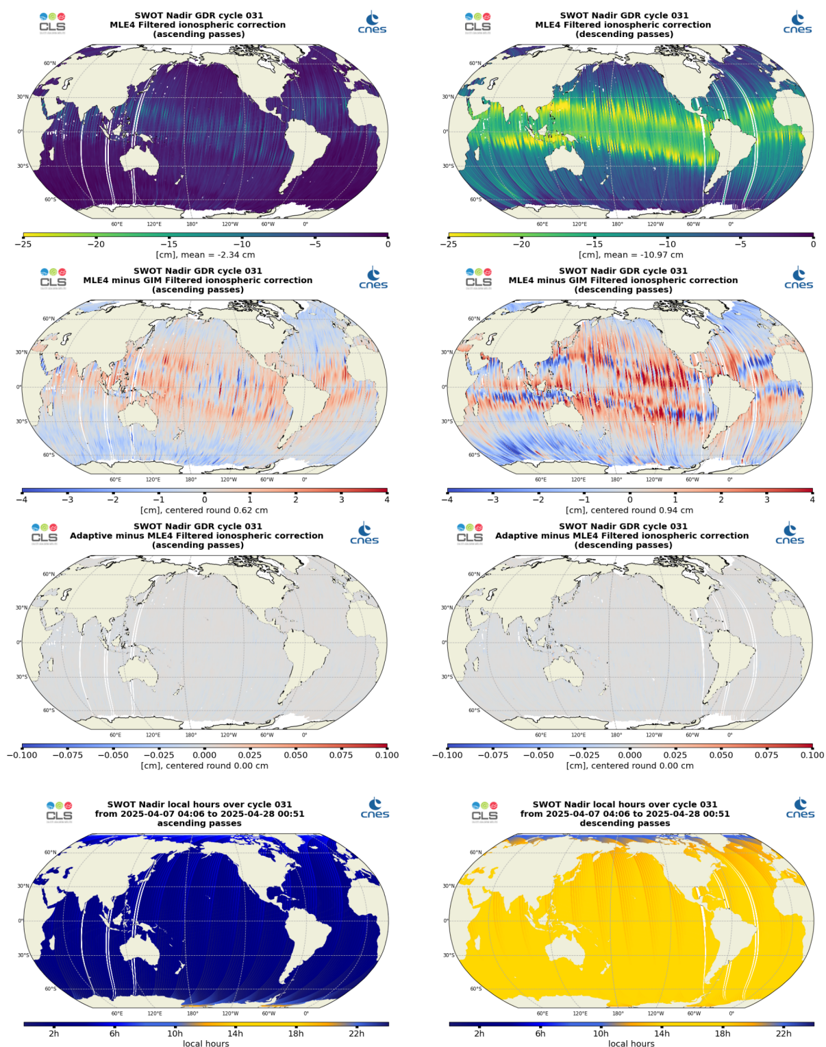
Figure 14: Along-track maps of filtered ionosphere correction over cycle 031 for SWOT Nadir MLE4 (top), MLE4 minus GIM (middle top) or Adaptive minus MLE4 (middle bottom), and local hours (bottom), for ascending passes (left) and descending passes (right)
