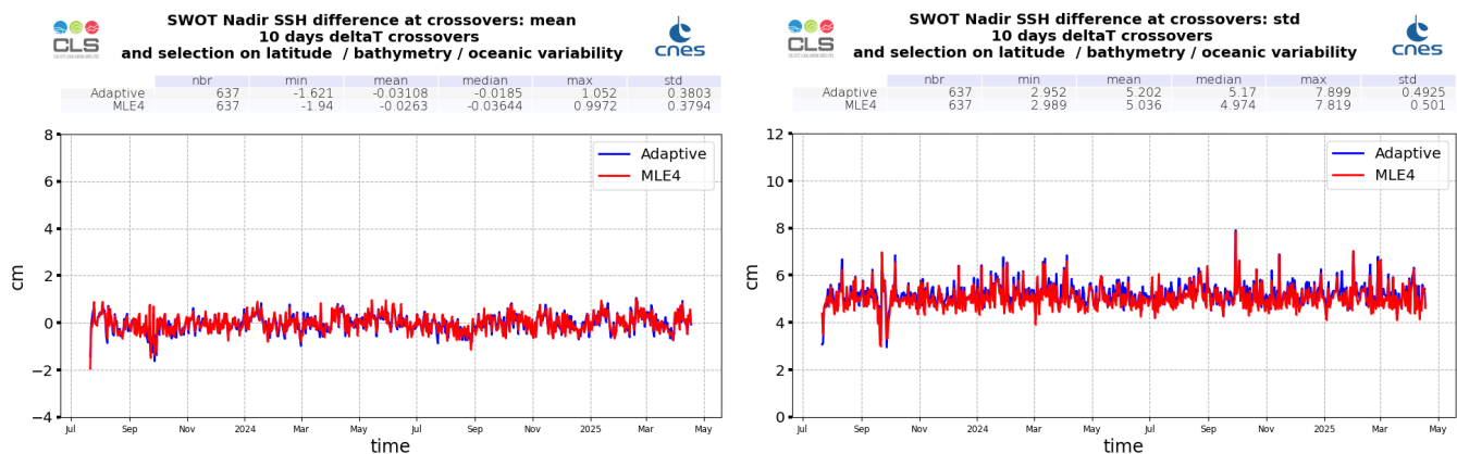
Figure 29: Monitoring of SSH difference at crossovers for SWOT Nadir MLE4 (red) and Adaptive (blue) : mean (left) and standard deviation (right), from cycle 001 to 031
