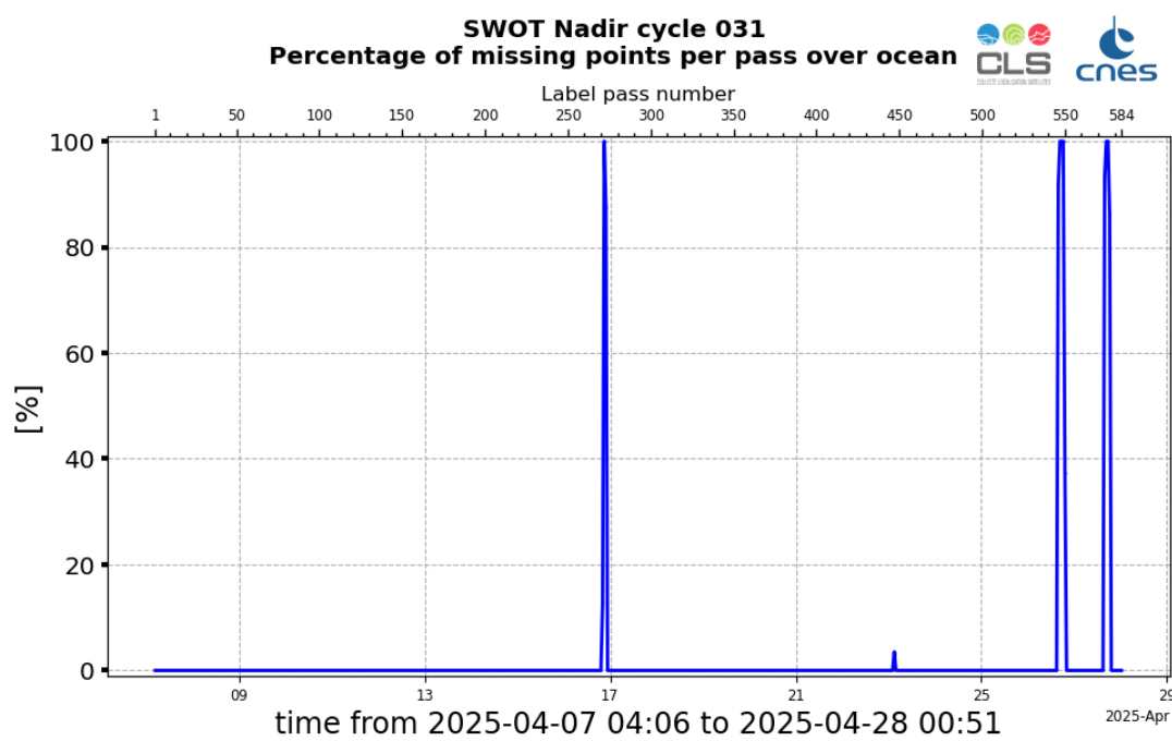
Figure 2: Monitoring of the percentage per pass of missing data over ocean, for SWOT Nadir GDR cycle 031
