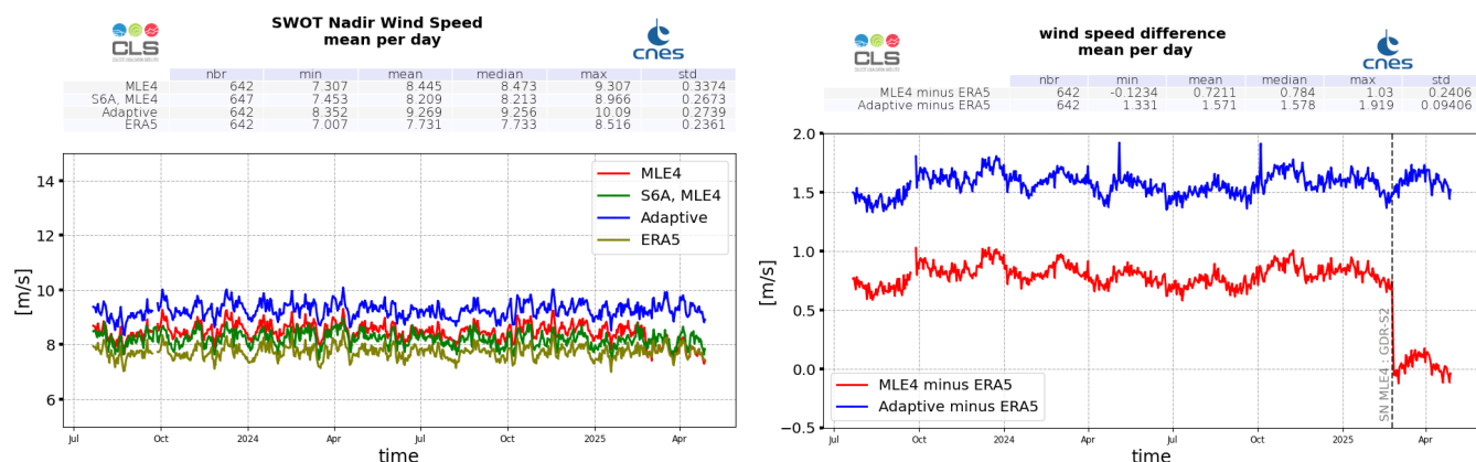
Figure 12: Wind Speed daily monitoring from cycle 001 to 031 for SWOT Nadir GDR, ERA5 model, and Sentinel-6A-MF (LR MLE4) (left), and daily mean difference with ERA5 (right)
