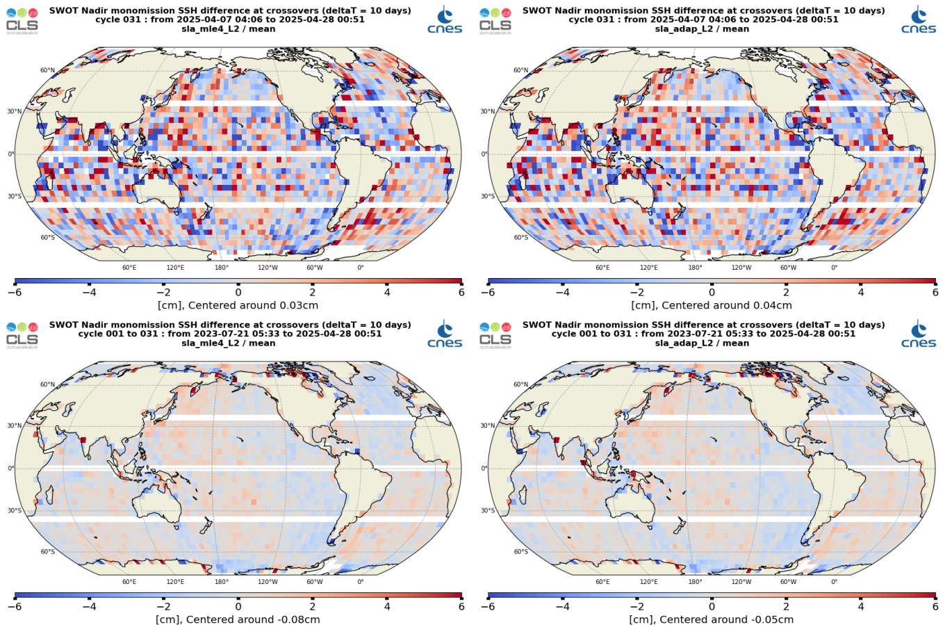
Figure 28: Mean SSH difference at crossovers for SWOT Nadir MLE4 (left) and Adaptive (right) cycle 031(top) and from cycle 001 to cycle 031 (bottom)
