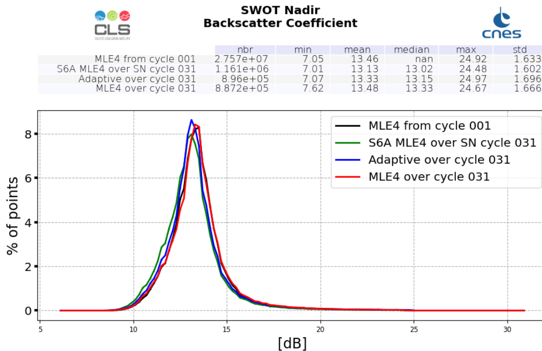
Figure 7: Ku-band Backscattering coefficient histogram computed over cycle 031 (red line for SWOT Nadir MLE4 and blue line for SWOT Nadir Adaptive, green for Sentinel-6A-MF (LR MLE4)) and from cycle 001 (SWOT Nadir, MLE4 only, black line)
