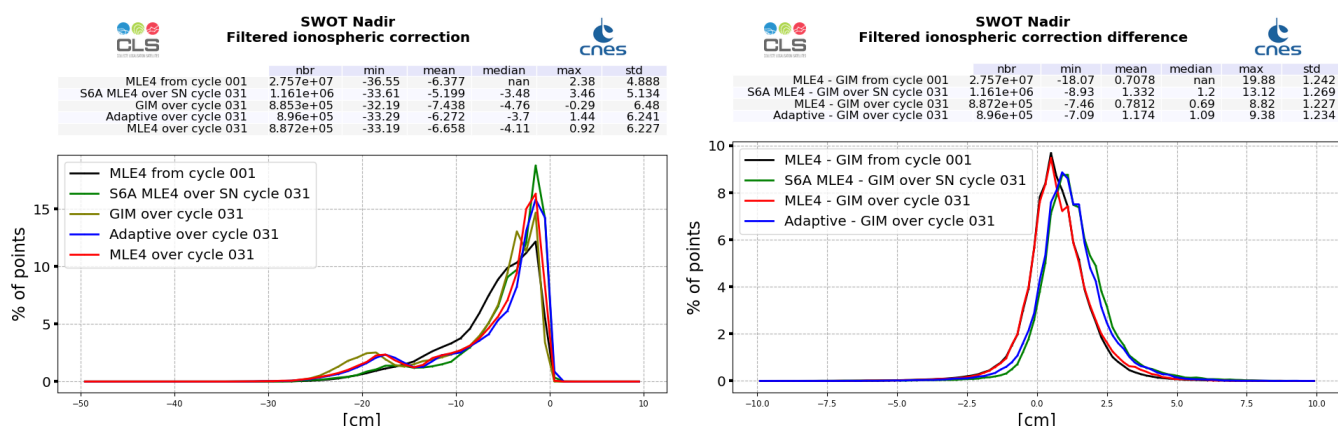
Figure 13: GIM model (dark green) and altimeter filtered ionosphere correction histogram computed over cycle 031 (red line for SWOT Nadir MLE4 and blue line for SWOT Nadir Adaptive, green for Sentinel-6A-MF (LR MLE4)) and from cycle 001 (SWOT Nadir, MLE4 only, black line) (left). Difference between filtered altimeter and GIM model (right).
