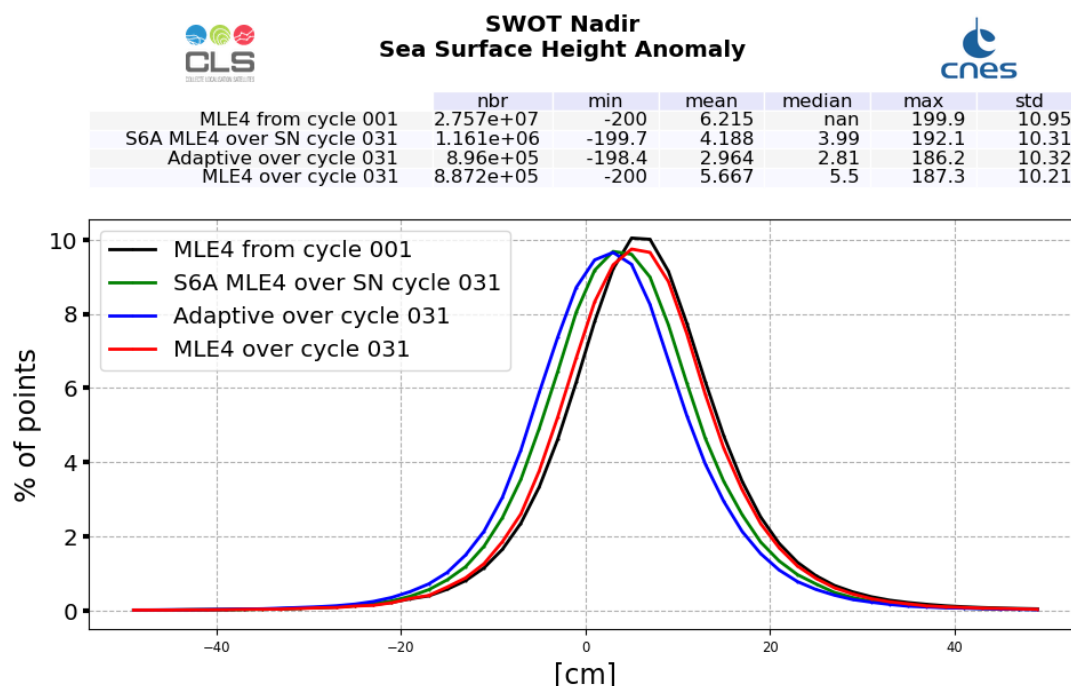
Figure 25: SSHA histogram computed over cycle 031 (red line for SWOT Nadir MLE4 and blue line for SWOT Nadir Adaptive, green for Sentinel-6A-MF (LR MLE4)) and from cycle 001 (SWOT Nadir, MLE4 only, black line)
