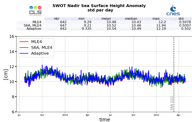
Figure 27: SSHA daily monitoring from cycle 001 to 031, for SWOT Nadir GDR
