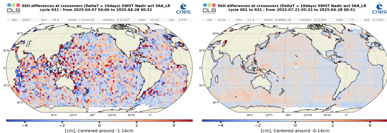
Figure 30: Mean SSH difference at crossovers between SWOT Nadir MLE4 and Sentinel-6 MF LR MLE4 over cycle 031 (left) and from cycle 001 onwards (right)
