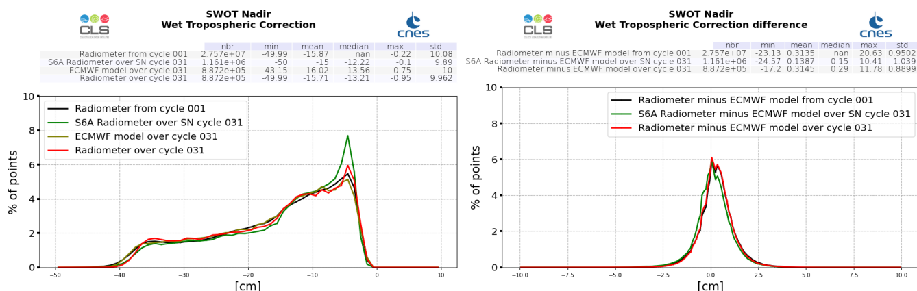
Figure 21: Histogram of wet troposphere corrections : SWOT Nadir radiometer (left) and difference with ECMWF model (right), computed over cycle 031 and from cycle 001 (black line)
