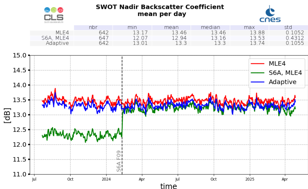
Figure 9: Ku-band Backscattering coefficient daily monitoring from cycle 001 to 031, for SWOT Nadir and Sentinel-6A-MF
