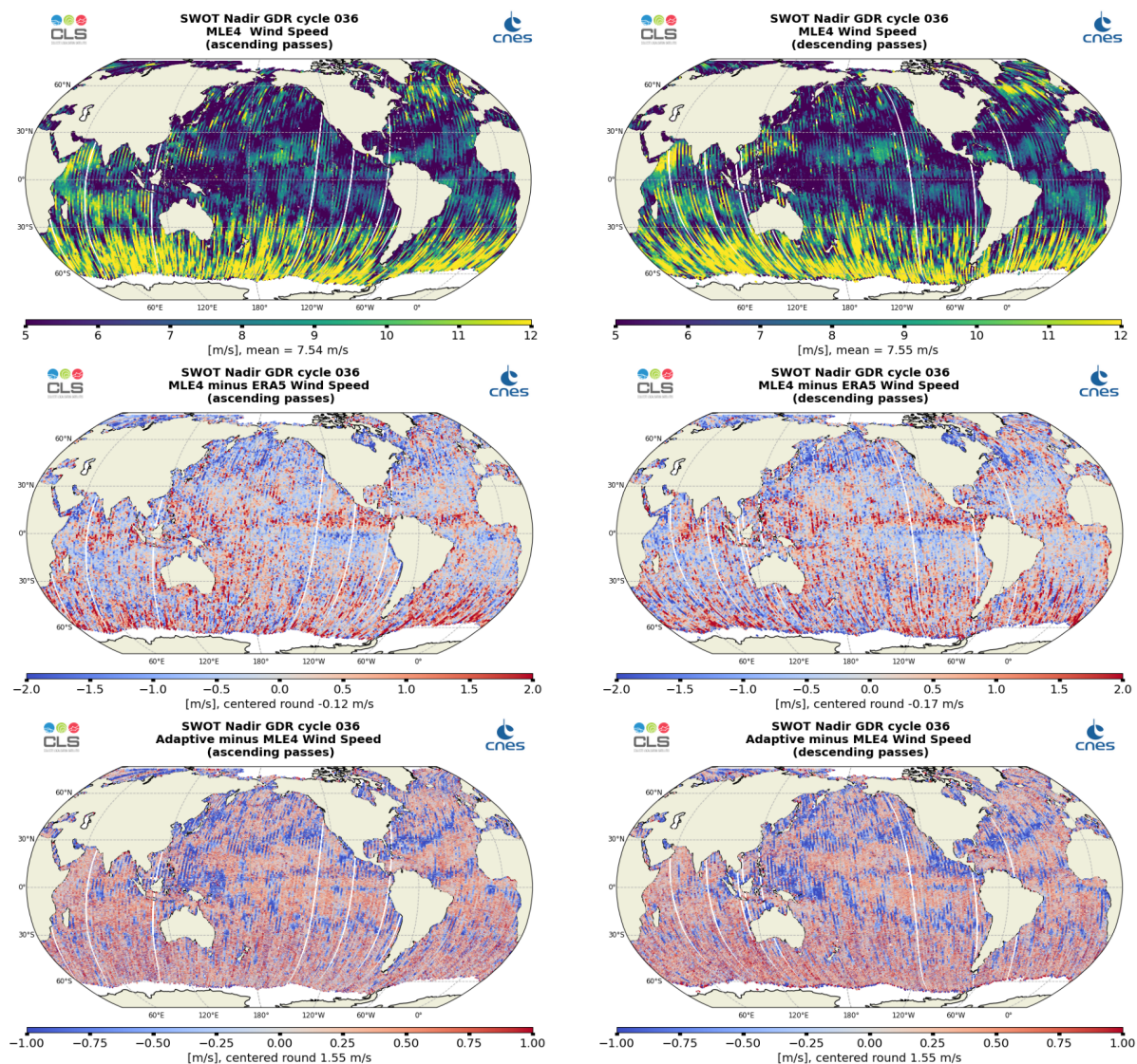
Figure 11: Along-track maps of Altimeter Wind Speed over cycle 036 for SWOT Nadir MLE4 (top), MLE4 minus ERA5 (middle) or Adaptive minus MLE4 (bottom), ascending passes (left) and descending passes (right)
