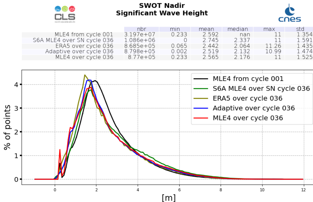
Figure 4: Ku-band Significant Wave Height histogram computed over cycle 036 (red line for SWOT Nadir MLE4 and blue line for SWOT Nadir Adaptive, green for Sentinel-6A-MF (LR MLE4) and dark green for ERA5) and from cycle 001 (SWOT Nadir, MLE4 only, black line)
