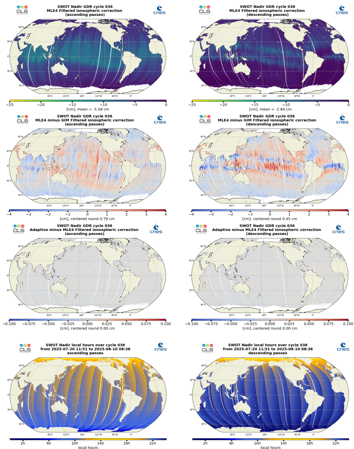
Figure 14: Along-track maps of filtered ionosphere correction over cycle 036 for SWOT Nadir MLE4 (top), MLE4 minus GIM (middle top) or Adaptive minus MLE4 (middle bottom), and local hours (bottom), for ascending passes (left) and descending passes (right)
