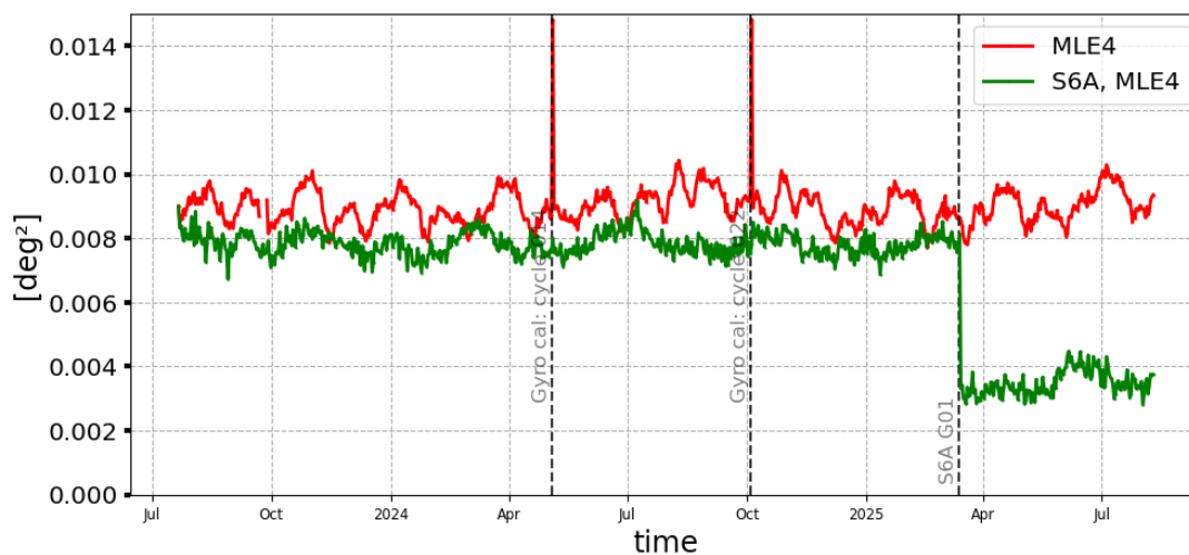
Figure 18: Mispointing daily monitoring from SWOT cycle 001 to 036 for SWOT Nadir GDR (red) and Sentinel-6A-MF (green)
