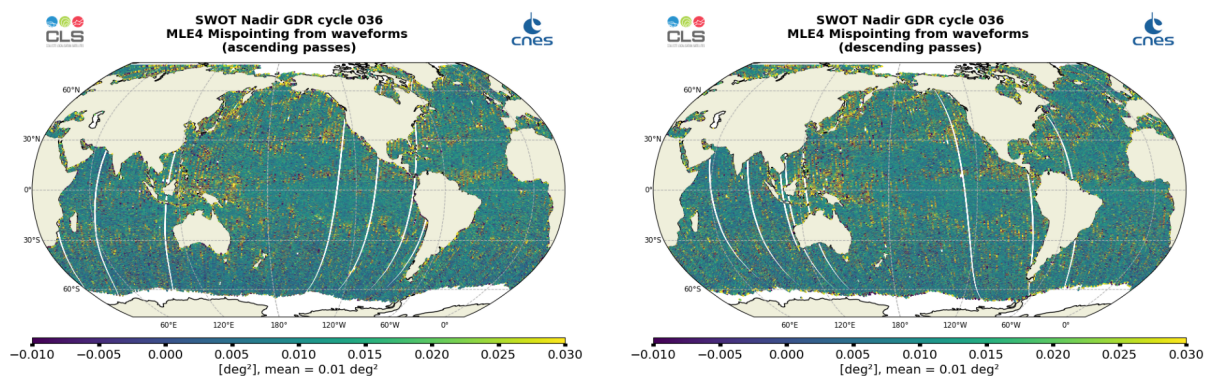
Figure 17: Along-track maps of mispointing over cycle 036 for SWOT Nadir MLE4, ascending passes (left) and descending passes (right)
