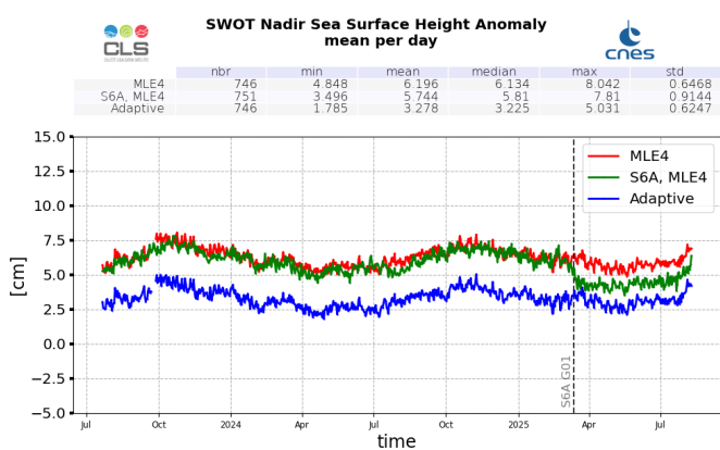
Figure 27: SSHA daily monitoring from cycle 001 to 036, for SWOT Nadir GDR
