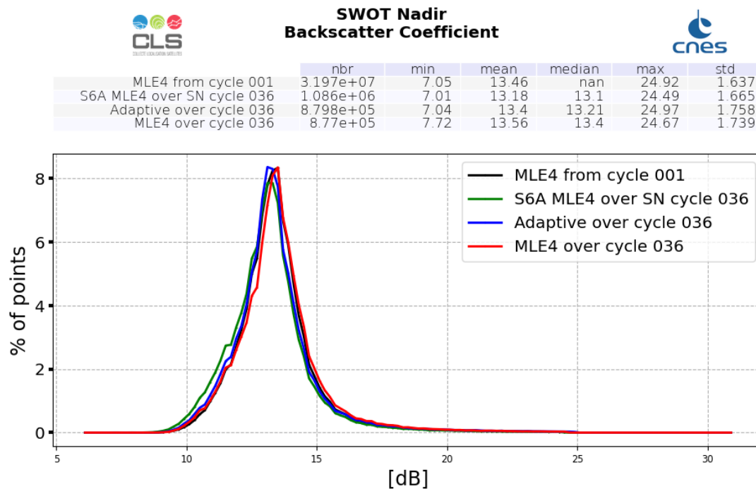
Figure 7: Ku-band Backscattering coefficient histogram computed over cycle 036 (red line for SWOT Nadir MLE4 and blue line for SWOT Nadir Adaptive, green for Sentinel-6A-MF (LR MLE4)) and from cycle 001 (SWOT Nadir, MLE4 only, black line)
