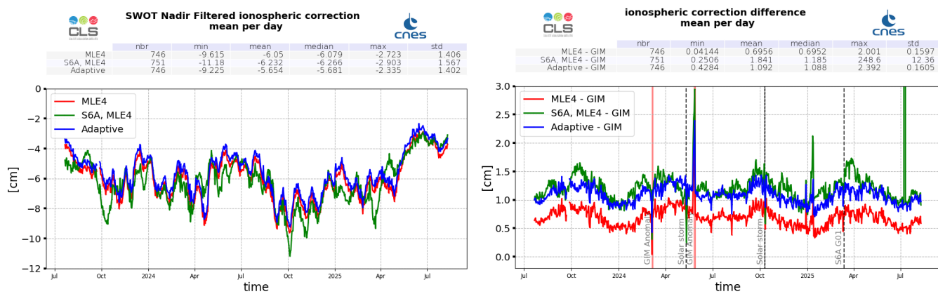
Figure 15: SWOT Nadir MLE4 (red), Adaptive (blue) and Sentinel-6A-MF (LR MLE4) (green) filtered ionosphere correction daily monitoring from cycle 001 to 036 (left) and difference with GIM model (right)
