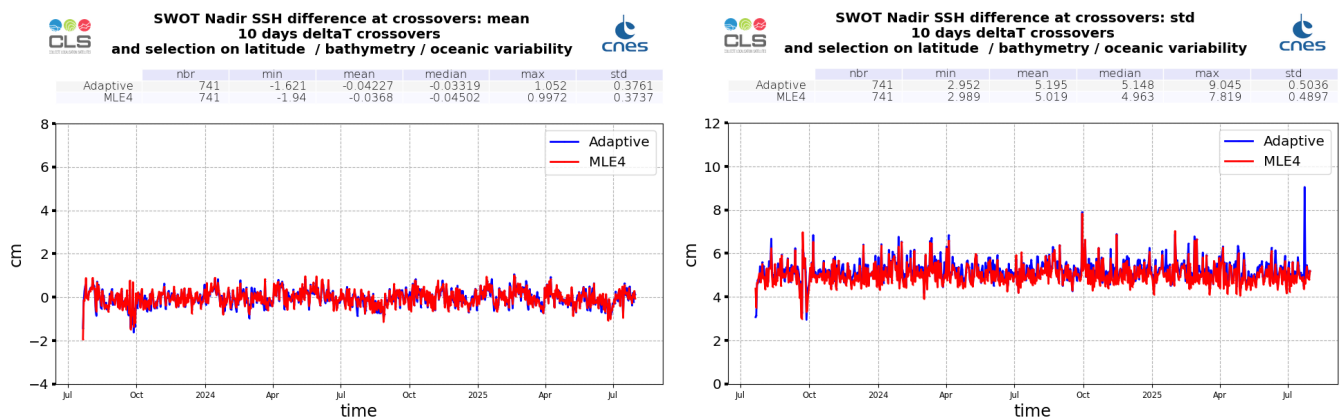
Figure 29: Monitoring of SSH difference at crossovers for SWOT Nadir MLE4 (red) and Adaptive (blue) : mean (left) and standard deviation (right), from cycle 001 to 036
