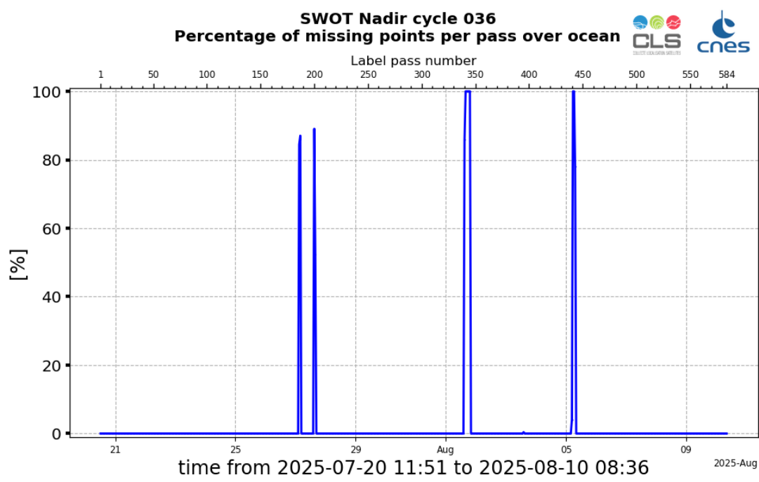
Figure 2: Monitoring of the percentage per pass of missing data over ocean, for SWOT Nadir GDR cycle 036
