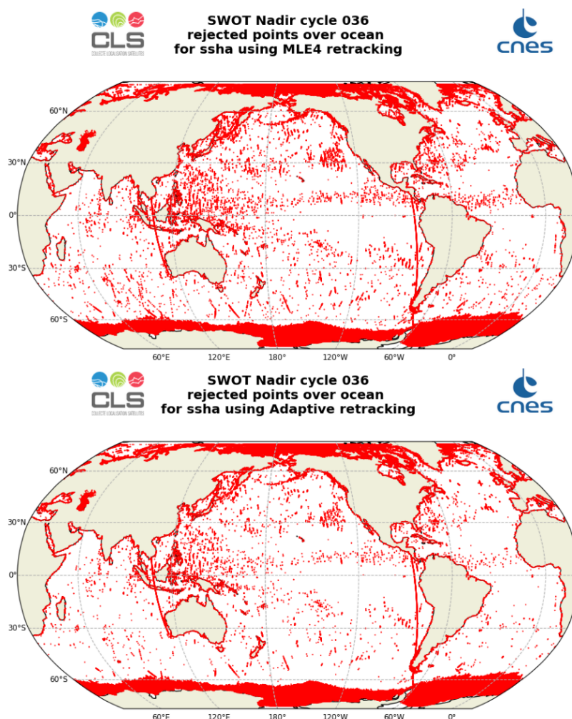
Figure 3: Edited measurements for SWOT Nadir over cycle 036
