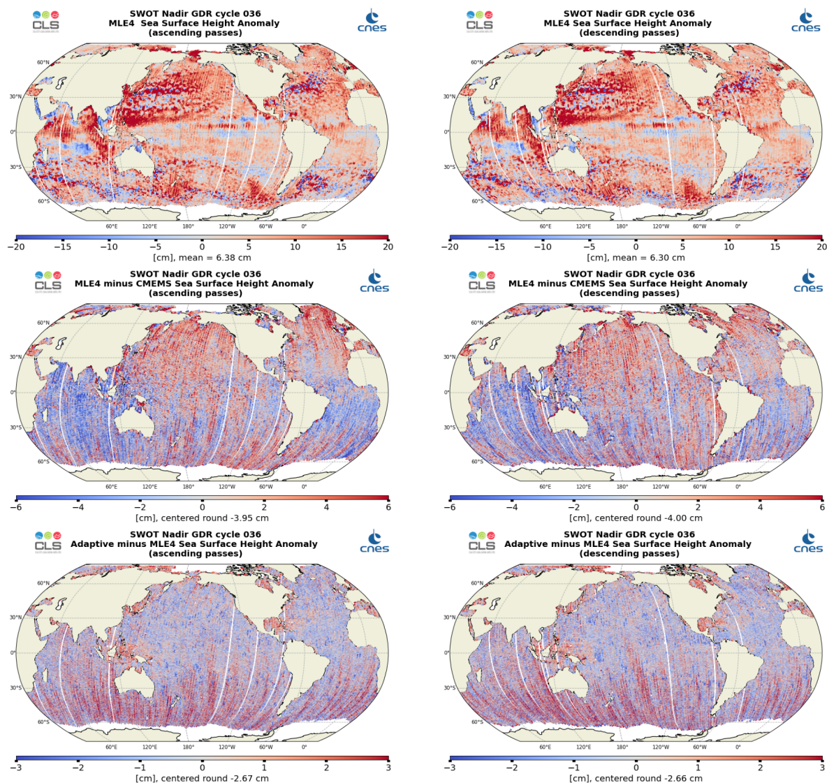
Figure 26: Along-track maps of SSHA over cycle 036 for SWOT Nadir MLE4 (top), MLE4 minus CMEMS (middle) or Adaptive minus MLE4 (bottom), ascending passes (left) and descending passes (right)
