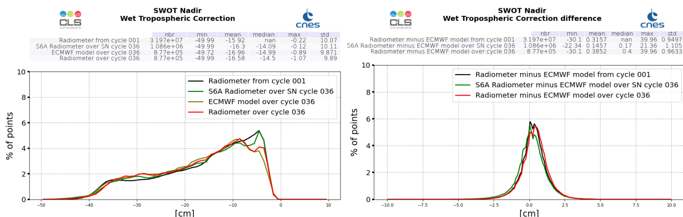
Figure 21: Histogram of wet troposphere corrections : SWOT Nadir radiometer (left) and difference with ECMWF model (right), computed over cycle 036 and from cycle 001 (black line)
