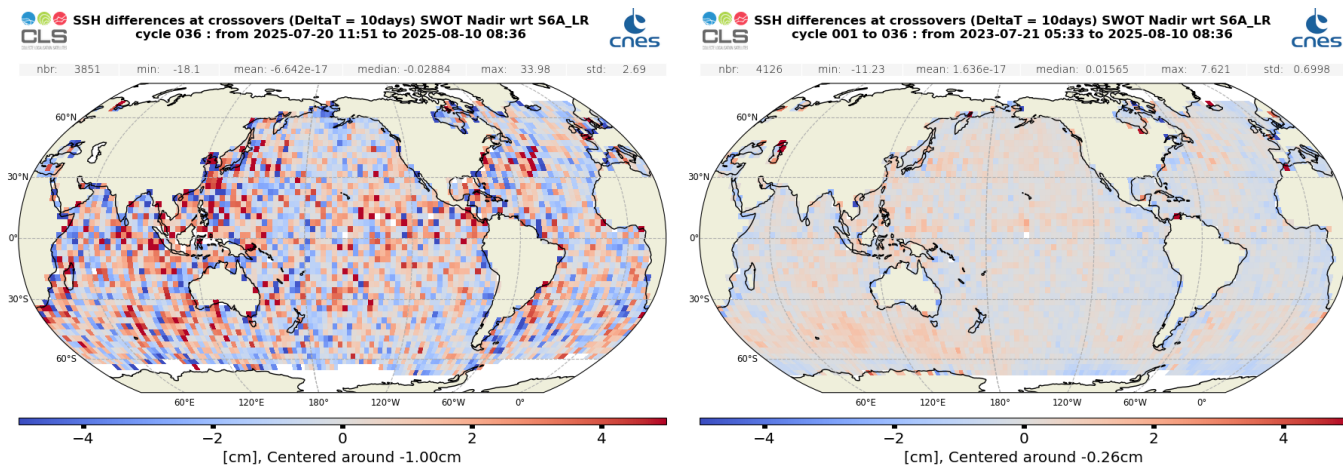
Figure 30: Mean SSH difference at crossovers between SWOT Nadir MLE4 and Sentinel-6 MF LR MLE4 over cycle 036 (left) and from cycle 001 onwards (right)
