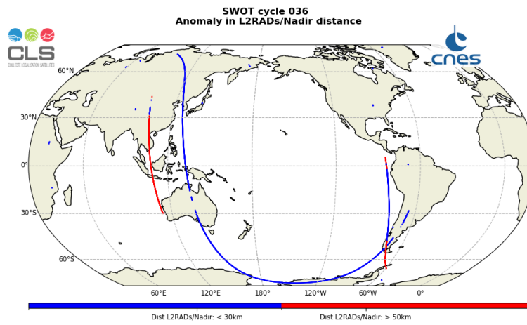
Figure 24: Map of the anomalies detected in the L2RADs/Nadir distance over the cycle 036
