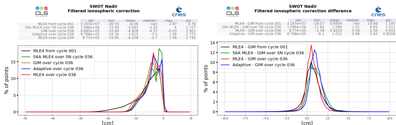
Figure 13: GIM model (dark green) and altimeter filtered ionosphere correction histogram computed over cycle 036 (red line for SWOT Nadir MLE4 and blue line for SWOT Nadir Adaptive, green for Sentinel-6A-MF (LR MLE4)) and from cycle 001 (SWOT Nadir, MLE4 only, black line) (left). Difference between filtered altimeter and GIM model (right).
