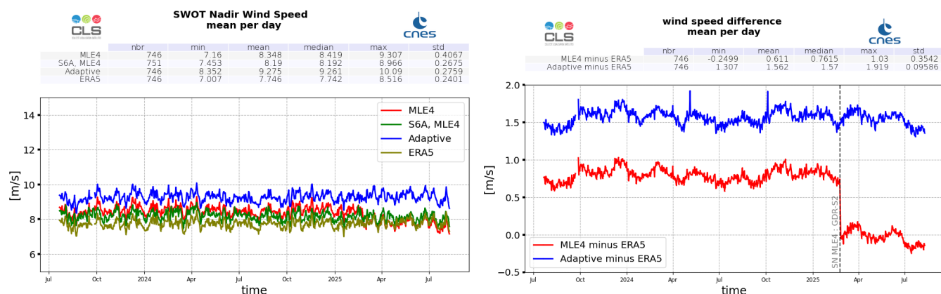
Figure 12: Wind Speed daily monitoring from cycle 001 to 036 for SWOT Nadir GDR, ERA5 model, and Sentinel-6A-MF (LR MLE4) (left), and daily mean difference with ERA5 (right)
