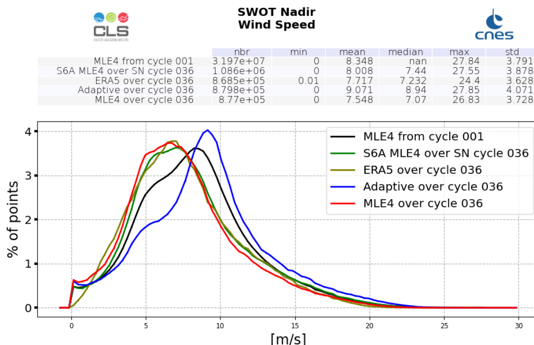
Figure 10: Altimeter Wind Speed histogram computed over cycle 036 (red line for SWOT Nadir MLE4 and blue line for SWOT Nadir Adaptive, green for Sentinel-6A-MF (LR MLE4)) and from cycle 001 (SWOT Nadir, MLE4 only, black line)
