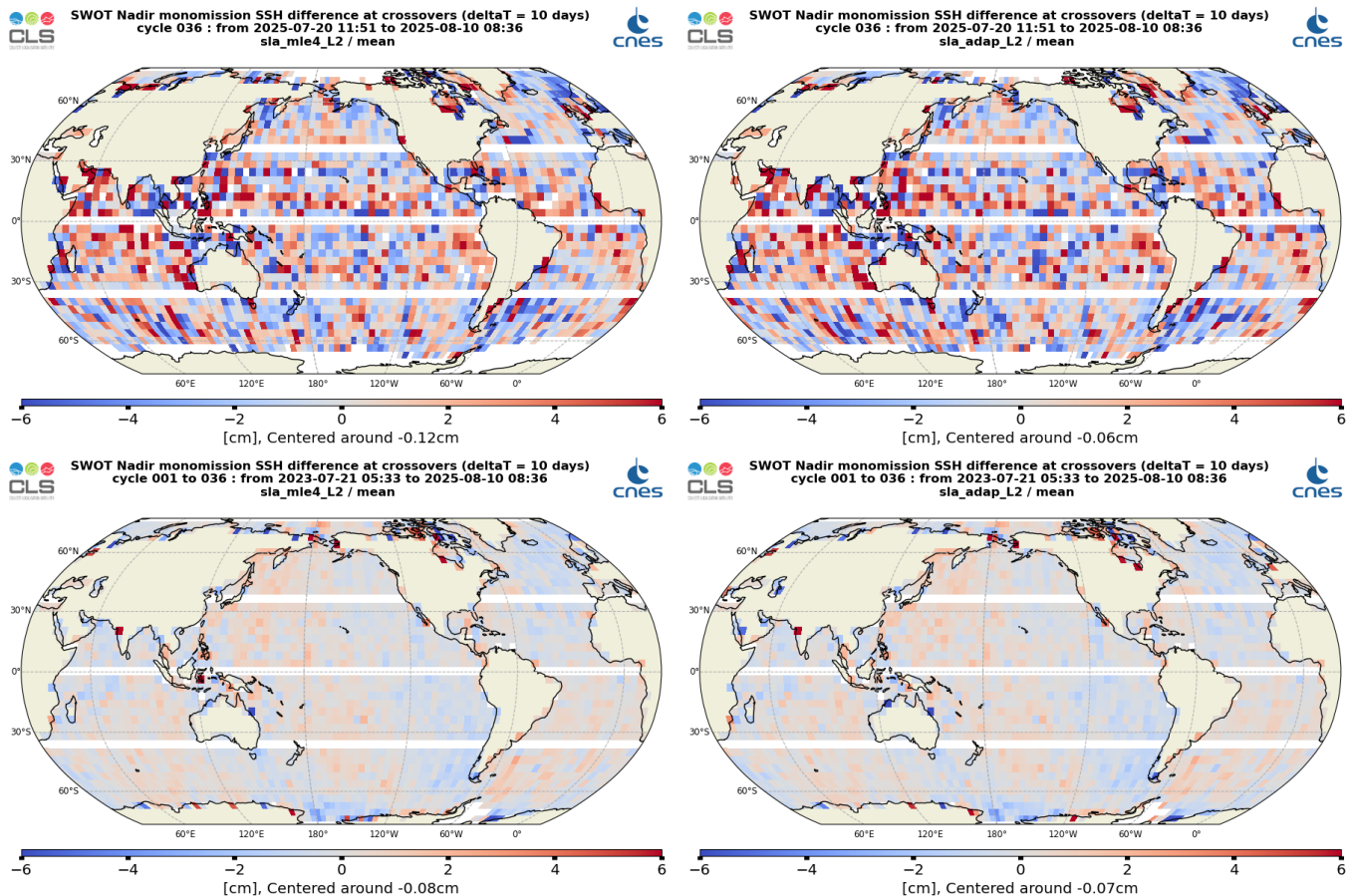
Figure 28: Mean SSH difference at crossovers for SWOT Nadir MLE4 (left) and Adaptive (right) cycle 036(top) and from cycle 001 to cycle 036 (bottom)
