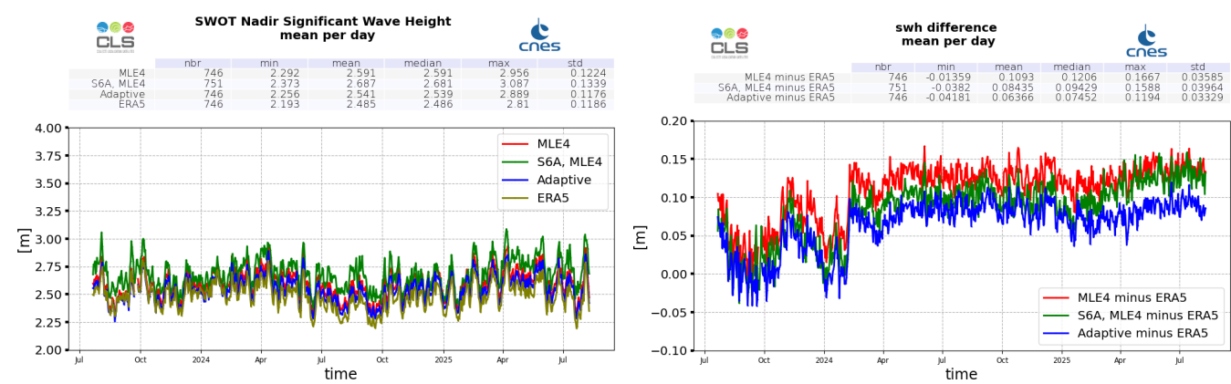
Figure 6: Ku-band Significant Wave Height daily monitoring from cycle 001 to 036, for SWOT Nadir, ERA5 model estimated at SWOT locations, and Sentinel-6A-MF (LR MLE4) (left), and difference with ERA5 model (right)
