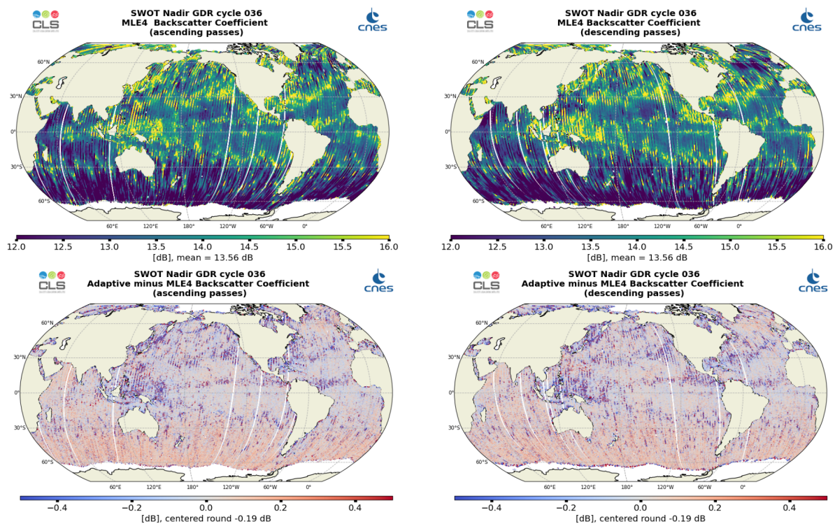
Figure 8: Along-track maps of Ku-band backscatter coefficient \sigma_0 over cycle 036 for SWOT Nadir MLE4 (top) or Adaptive minus MLE4 difference (bottom), ascending passes (left) and descending passes (right)
