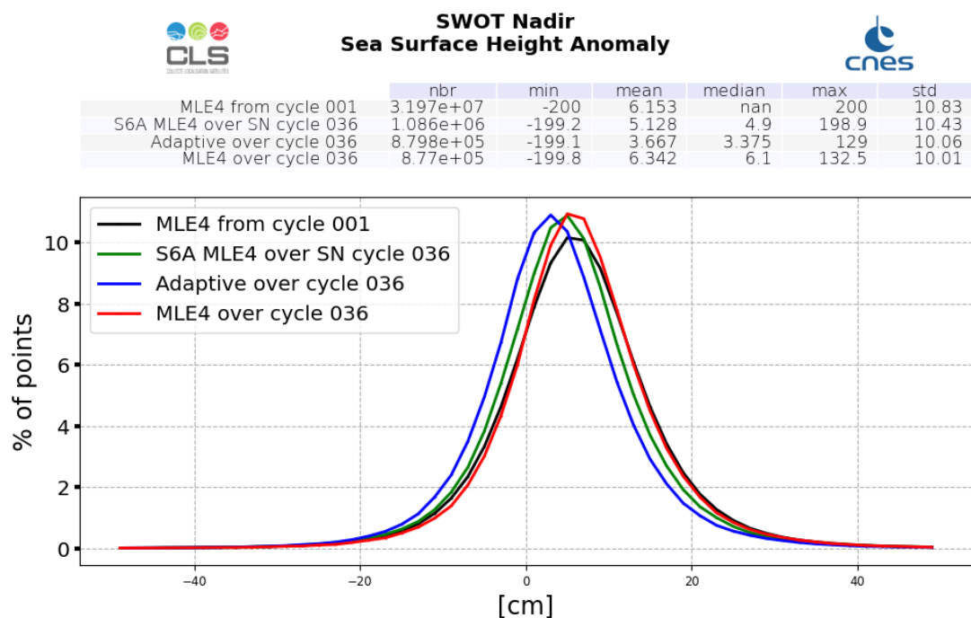
Figure 25: SSHA histogram computed over cycle 036 (red line for SWOT Nadir MLE4 and blue line for SWOT Nadir Adaptive, green for Sentinel-6A-MF (LR MLE4)) and from cycle 001 (SWOT Nadir, MLE4 only, black line)
