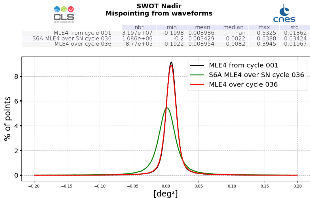
Figure 16: Mispointing histogram computed over cycle 036 (solid line) and from cycle 4 (dashed line)
