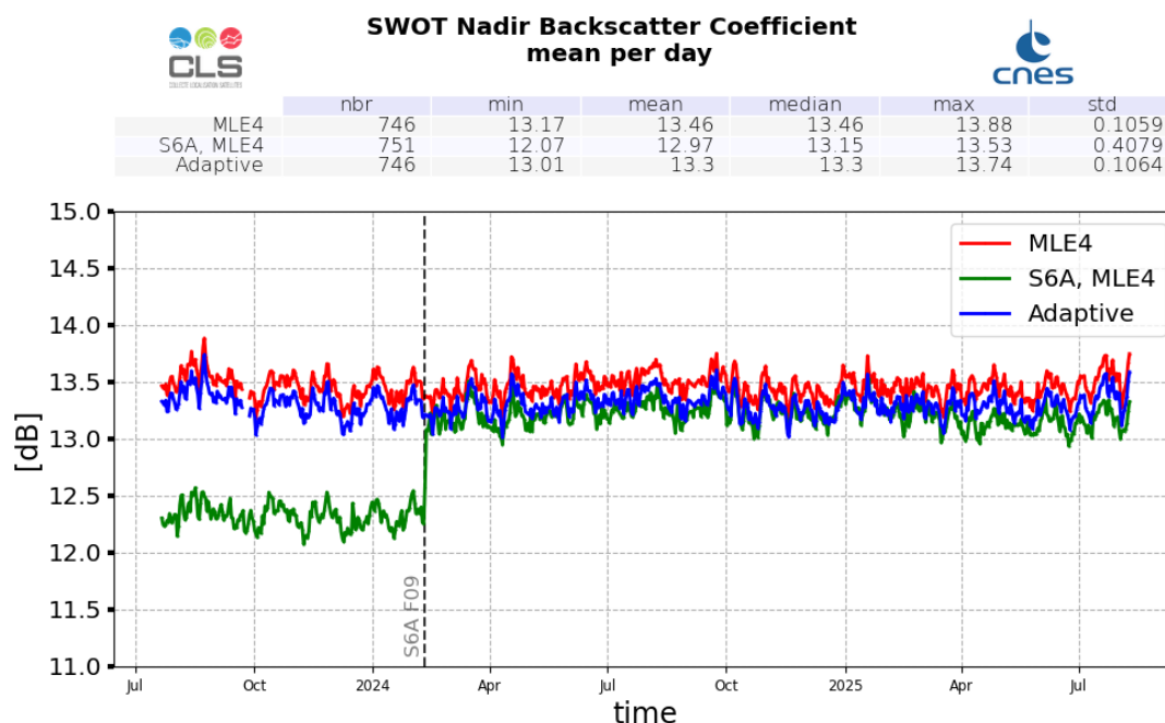
Figure 9: Ku-band Backscattering coefficient daily monitoring from cycle 001 to 036, for SWOT Nadir and Sentinel-6A-MF
