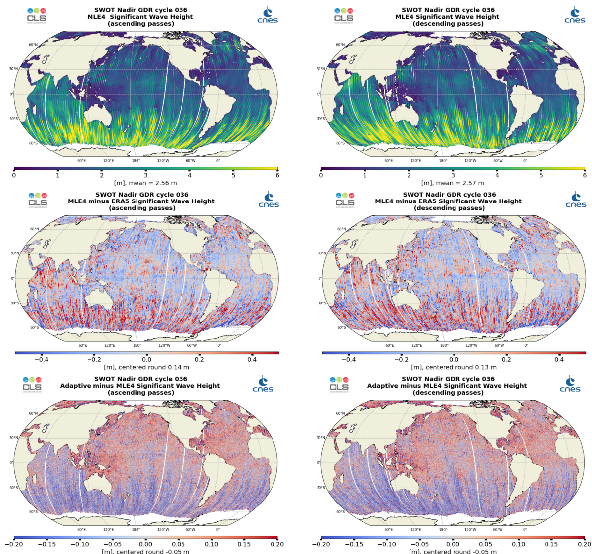
Figure 5: Along-track maps of Ku-band Significant Wave Height over cycle 036 for SWOT Nadir MLE4 (top), MLE4 minus model (middle) or Adaptive minus MLE4 (bottom), ascending passes (left) and descending passes (right)
