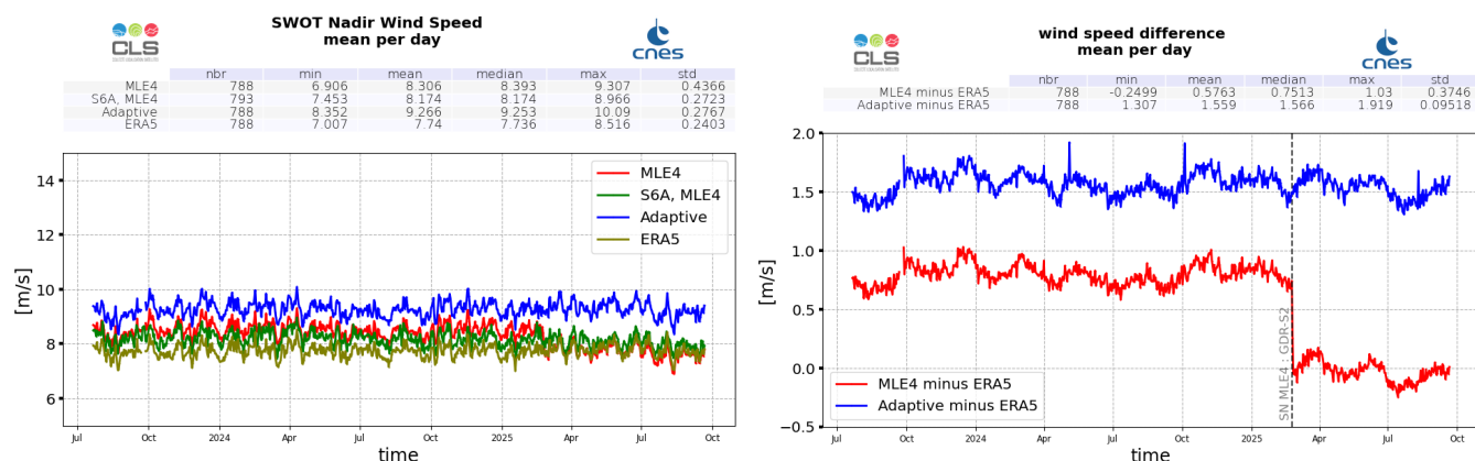
Figure 12: Wind Speed daily monitoring from cycle 001 to 038 for SWOT Nadir GDR, ERA5 model, and Sentinel-6A-MF (LR MLE4) (left), and daily mean difference with ERA5 (right)
