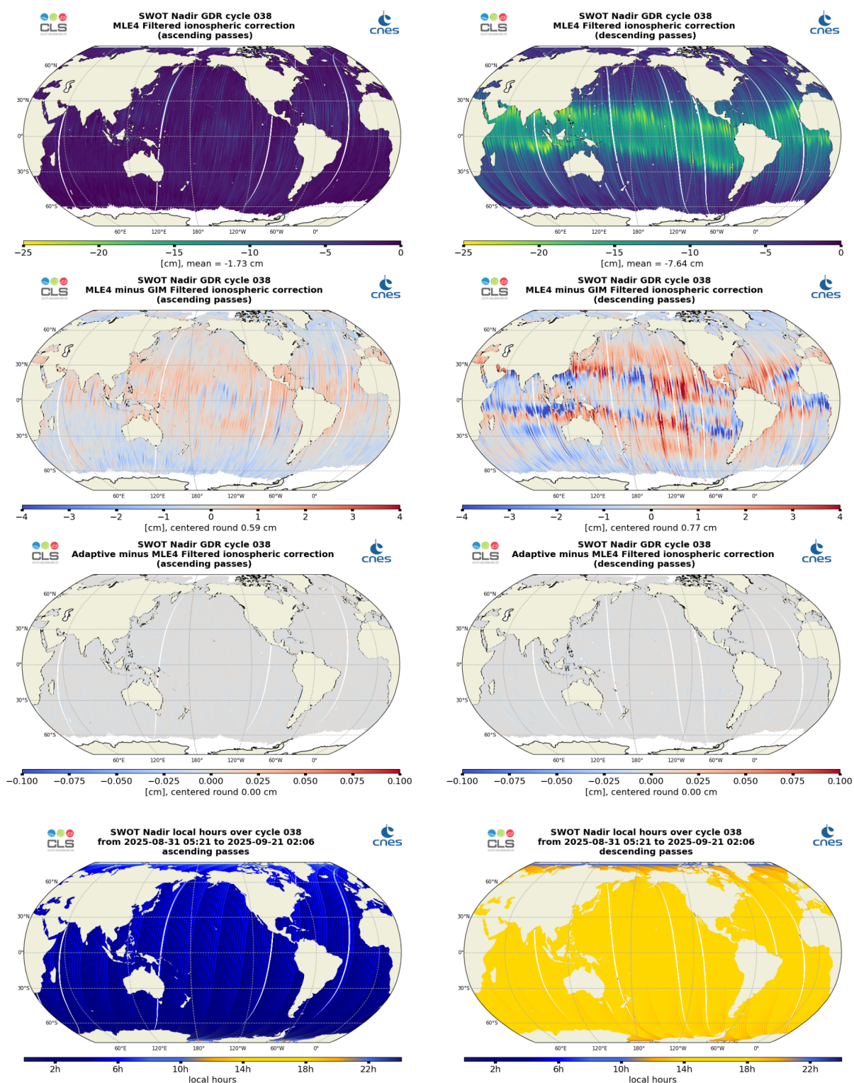
Figure 14: Along-track maps of filtered ionosphere correction over cycle 038 for SWOT Nadir MLE4 (top), MLE4 minus GIM (middle top) or Adaptive minus MLE4 (middle bottom), and local hours (bottom), for ascending passes (left) and descending passes (right)
