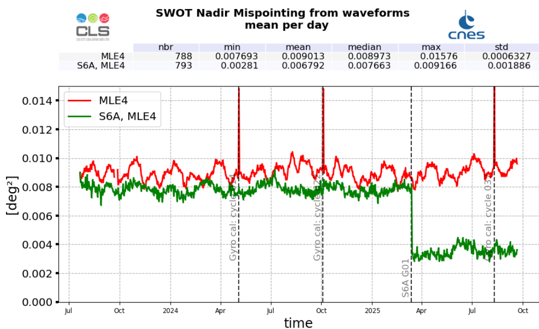
Figure 18: Mispointing daily monitoring from SWOT cycle 001 to 038 for SWOT Nadir GDR (red) and Sentinel-6A-MF (green)
