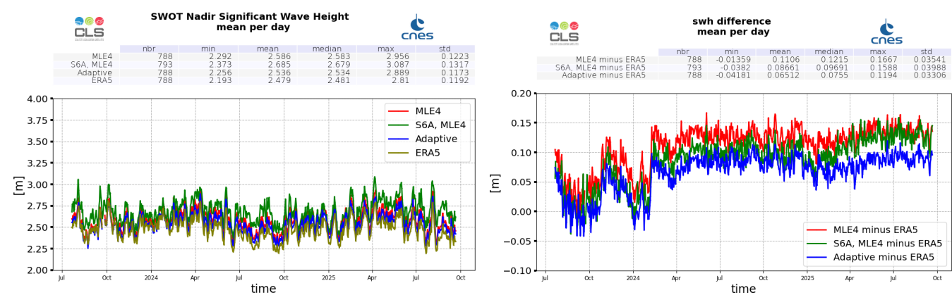
Figure 6: Ku-band Significant Wave Height daily monitoring from cycle 001 to 038, for SWOT Nadir, ERA5 model estimated at SWOT locations, and Sentinel-6A-MF (LR MLE4) (left), and difference with ERA5 model (right)
