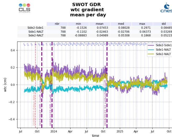
Figure 20: Daily monitoring of the wet tropospheric correction gradient between AMR Side 1 and AMR Side 2 (purple), AMR Side 1 and Nadir (cyan), and AMR Side 2 and Nadir (yellow), from Cycle 001 to 038
