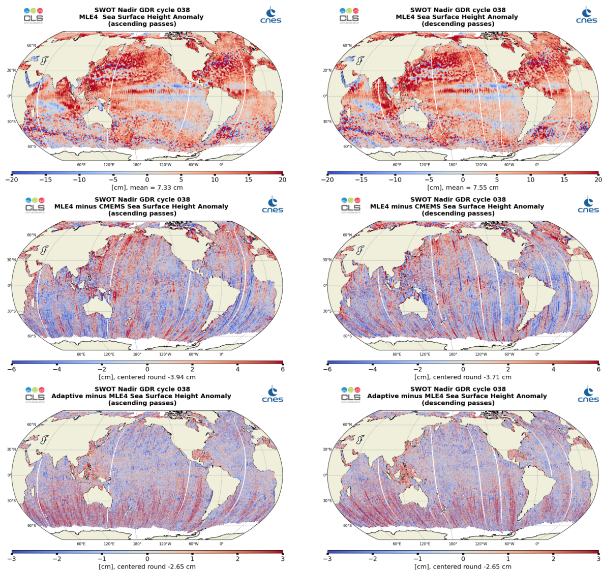
Figure 26: Along-track maps of SSHA over cycle 038 for SWOT Nadir MLE4 (top), MLE4 minus CMEMS (middle) or Adaptive minus MLE4 (bottom), ascending passes (left) and descending passes (right)
