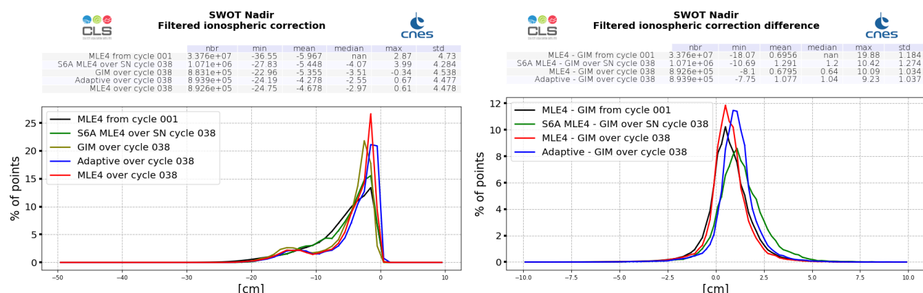
Figure 13: GIM model (dark green) and altimeter filtered ionosphere correction histogram computed over cycle 038 (red line for SWOT Nadir MLE4 and blue line for SWOT Nadir Adaptive, green for Sentinel-6A-MF (LR MLE4)) and from cycle 001 (SWOT Nadir, MLE4 only, black line) (left). Difference between filtered altimeter and GIM model (right).
