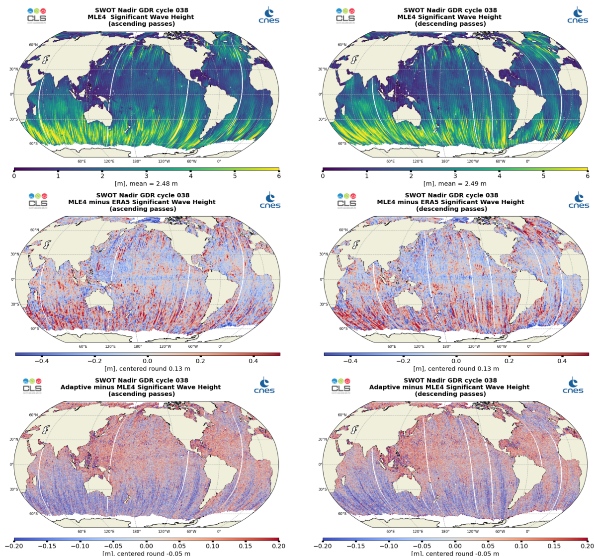
Figure 5: Along-track maps of Ku-band Significant Wave Height over cycle 038 for SWOT Nadir MLE4 (top), MLE4 minus model (middle) or Adaptive minus MLE4 (bottom), ascending passes (left) and descending passes (right)
