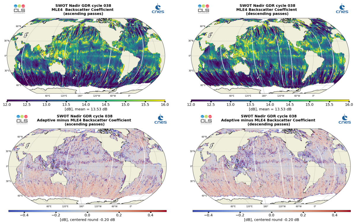
Figure 8: Along-track maps of Ku-band backscatter coefficient \sigma_0 over cycle 038 for SWOT Nadir MLE4 (top) or Adaptive minus MLE4 difference (bottom), ascending passes (left) and descending passes (right)
