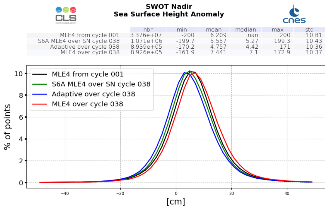
Figure 25: SSHA histogram computed over cycle 038 (red line for SWOT Nadir MLE4 and blue line for SWOT Nadir Adaptive, green for Sentinel-6A-MF (LR MLE4)) and from cycle 001 (SWOT Nadir, MLE4 only, black line)
