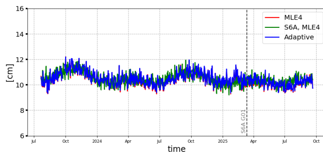
Figure 27: SSHA daily monitoring from cycle 001 to 038, for SWOT Nadir GDR
