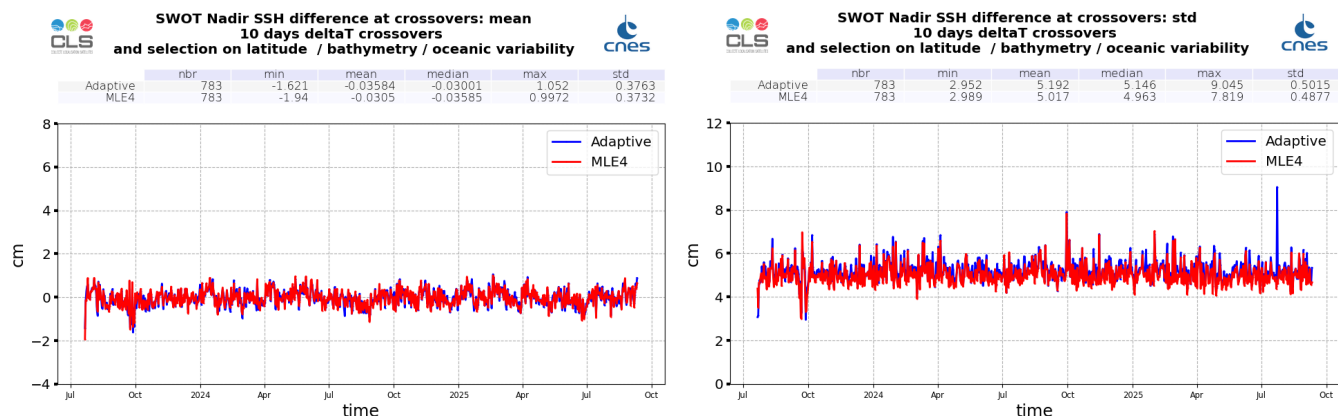
Figure 29: Monitoring of SSH difference at crossovers for SWOT Nadir MLE4 (red) and Adaptive (blue) : mean (left) and standard deviation (right), from cycle 001 to 038
