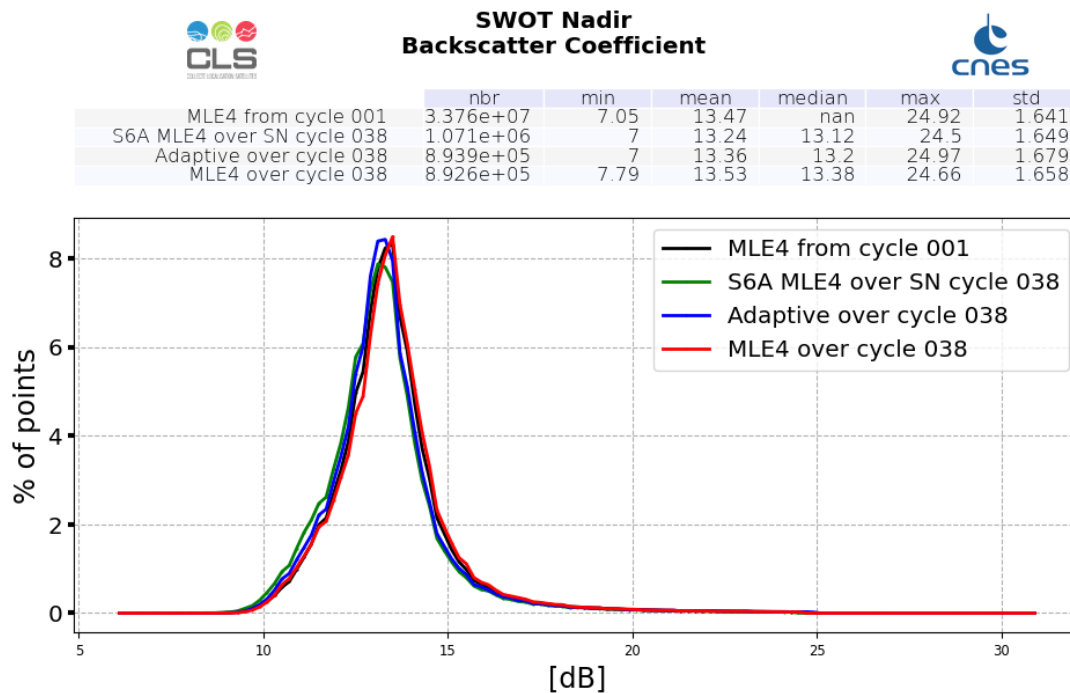
Figure 7: Ku-band Backscattering coefficient histogram computed over cycle 038 (red line for SWOT Nadir MLE4 and blue line for SWOT Nadir Adaptive, green for Sentinel-6A-MF (LR MLE4)) and from cycle 001 (SWOT Nadir, MLE4 only, black line)
