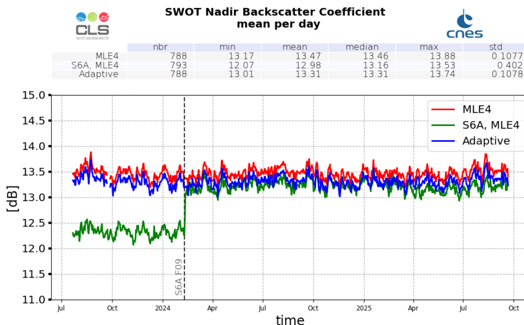
Figure 9: Ku-band Backscattering coefficient daily monitoring from cycle 001 to 038, for SWOT Nadir and Sentinel-6A-MF
