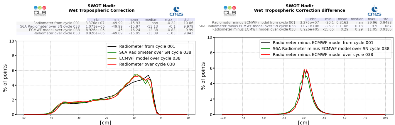
Figure 21: Histogram of wet troposphere corrections : SWOT Nadir radiometer (left) and difference with ECMWF model (right), computed over cycle 038 and from cycle 001 (black line)
