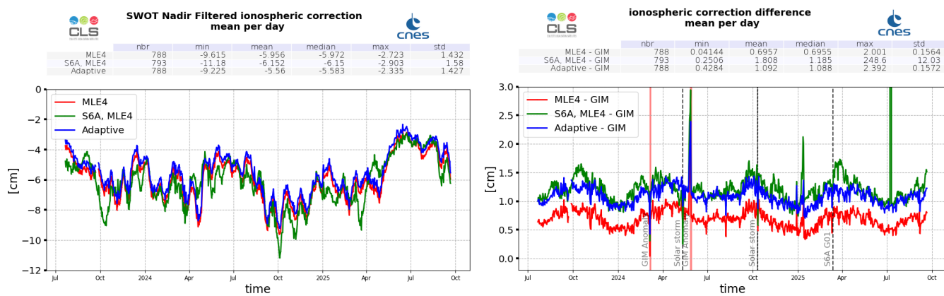
Figure 15: SWOT Nadir MLE4 (red), Adaptive (blue) and Sentinel-6A-MF (LR MLE4) (green) filtered ionosphere correction daily monitoring from cycle 001 to 038 (left) and difference with GIM model (right)
