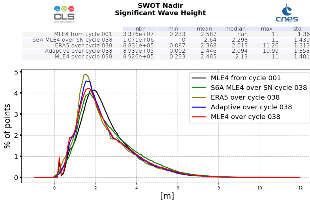
Figure 4: Ku-band Significant Wave Height histogram computed over cycle 038 (red line for SWOT Nadir MLE4 and blue line for SWOT Nadir Adaptive, green for Sentinel-6A-MF (LR MLE4) and dark green for ERA5) and from cycle 001 (SWOT Nadir, MLE4 only, black line)
