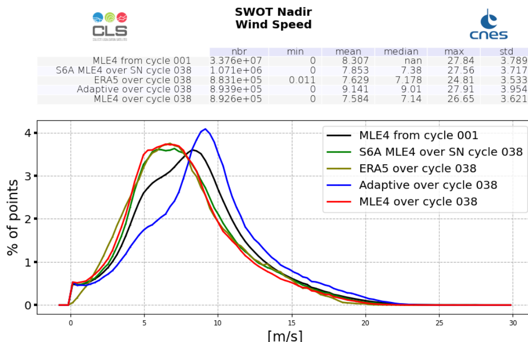
Figure 10: Altimeter Wind Speed histogram computed over cycle 038 (red line for SWOT Nadir MLE4 and blue line for SWOT Nadir Adaptive, green for Sentinel-6A-MF (LR MLE4)) and from cycle 001 (SWOT Nadir, MLE4 only, black line)
