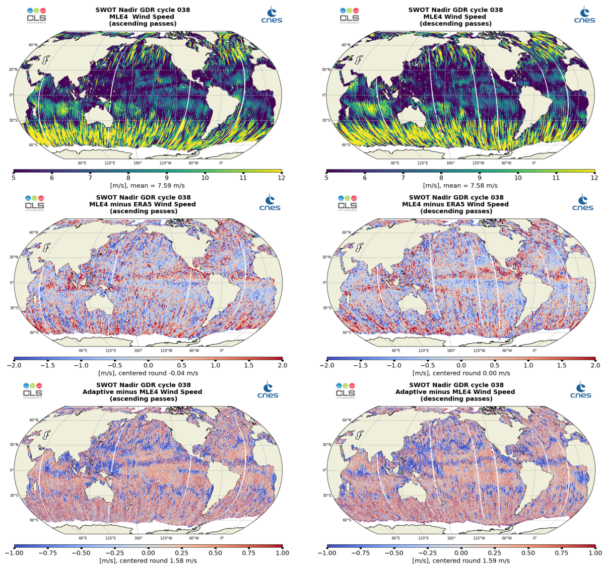
Figure 11: Along-track maps of Altimeter Wind Speed over cycle 038 for SWOT Nadir MLE4 (top), MLE4 minus ERA5 (middle) or Adaptive minus MLE4 (bottom), ascending passes (left) and descending passes (right)
