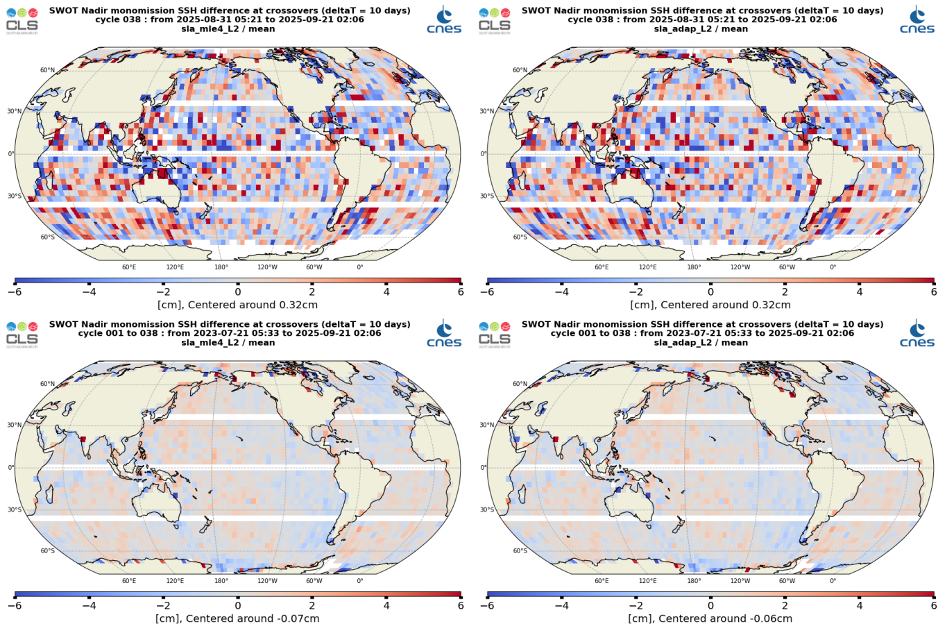
Figure 28: Mean SSH difference at crossovers for SWOT Nadir MLE4 (left) and Adaptive (right) cycle 038(top) and from cycle 001 to cycle 038 (bottom)
