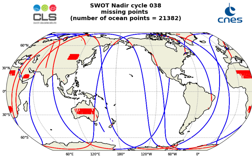
Figure 1: Map of missing measurements for SWOT Nadir GDR cycle 038
