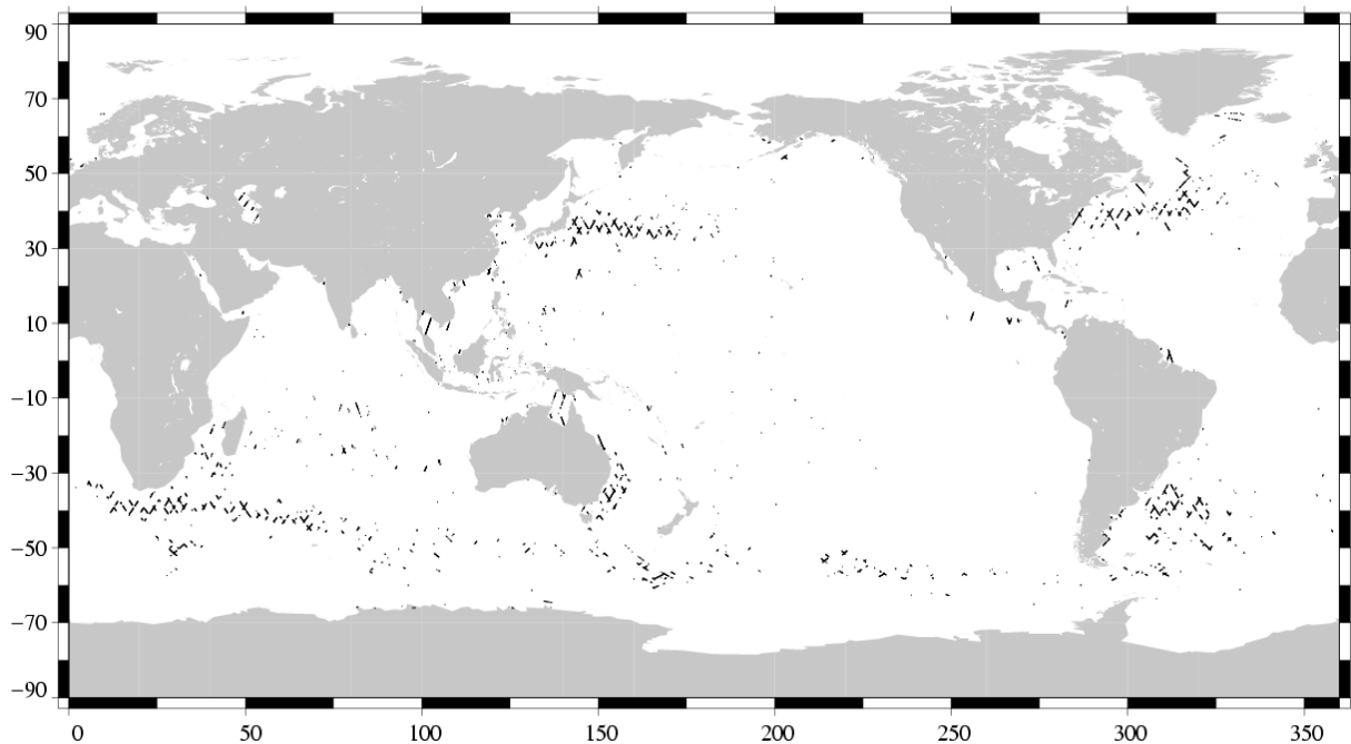
(SSH – MSS) differences greater than 0.3 m TOPEX/Poseidon Cycle 383 (05/02/2003 / 15/02/2003)
