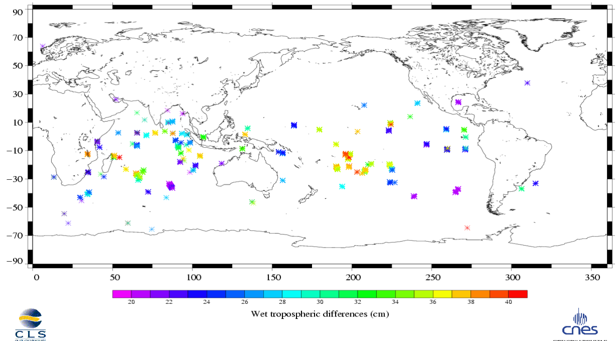
Edited parameter : Radiometer and ECMWF wet tropospheric differences T/P Cycle 383 (05/02/2003 / 15/02/2003)
