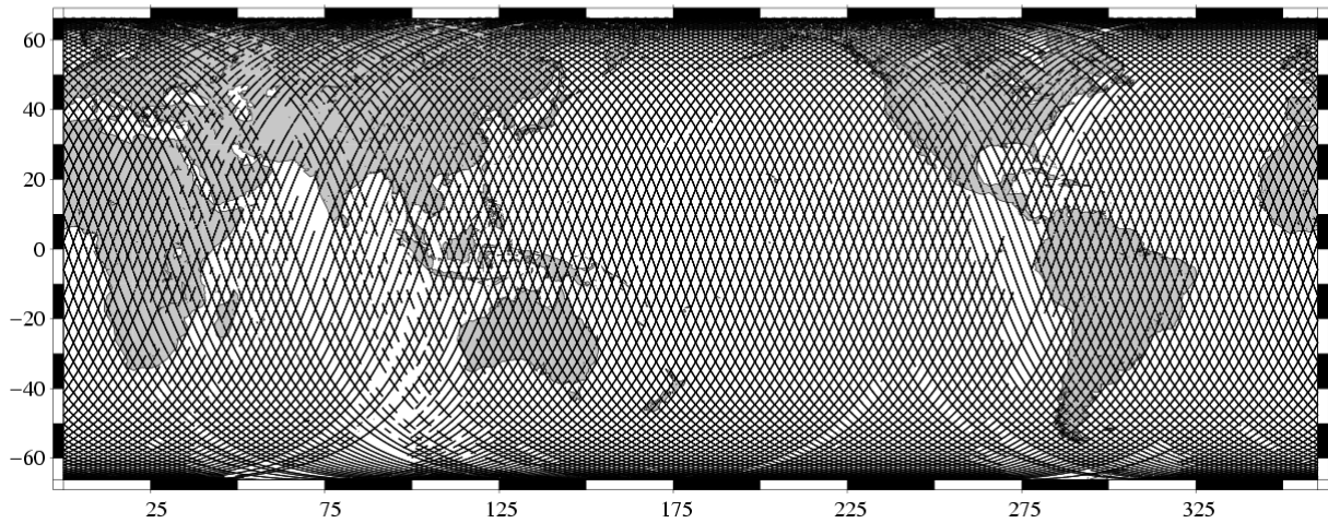
Missing measurements TOPEX/Poseidon Cycle 407 (01/10/2003 / 11/10/2003)
