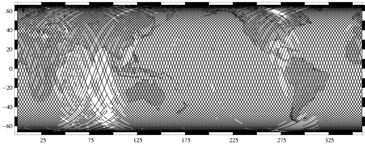
Missing measurements TOPEX/Poseidon Cycle 408 (11/10/2003 / 21/10/2003)
