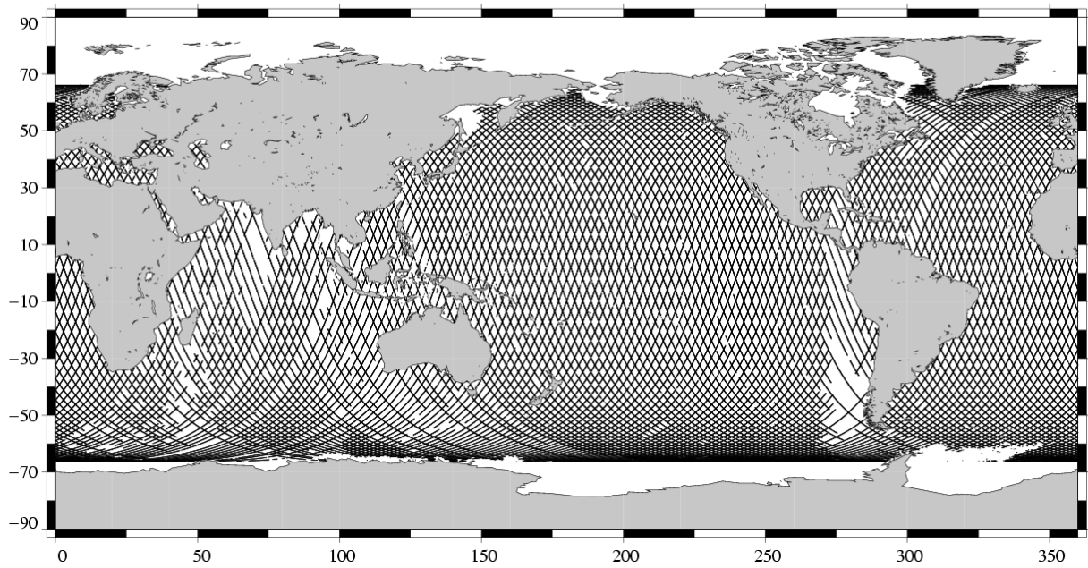
Edited measurements TOPEX Cycle 418 (19/01/2004 / 28/01/2004)
