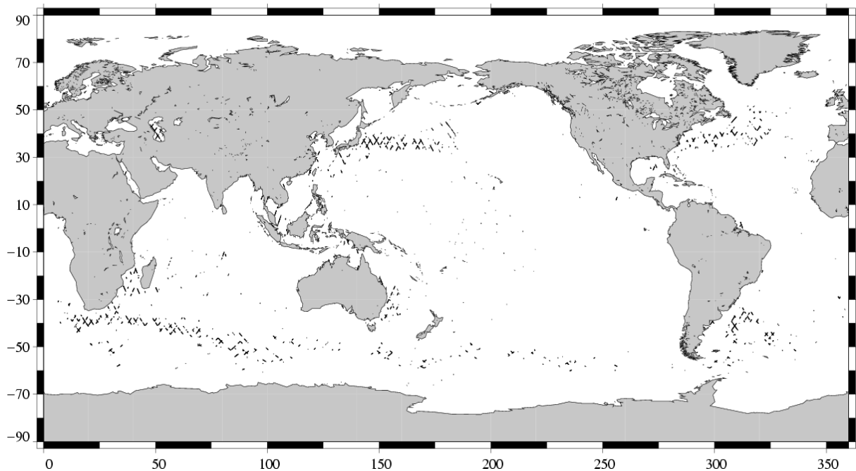
(SSH - MSS) differences greater than 0.3 m TOPEX/Poseidon Cycle 418 (19/01/2004 / 28/01/2004)
