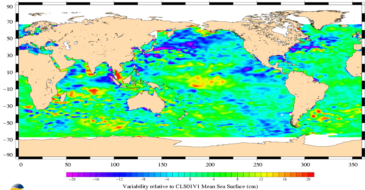
(SSH - MSS) differences greater than 0.3 m TOPEX/Poseidon Cycle 418 (19/01/2004 / 28/01/2004)
