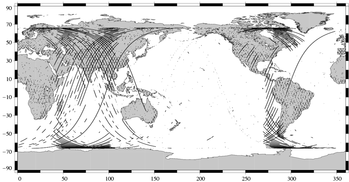
Missing measurements TOPEX/Poseidon Cycle 418 (19/01/2004 / 28/01/2004)
