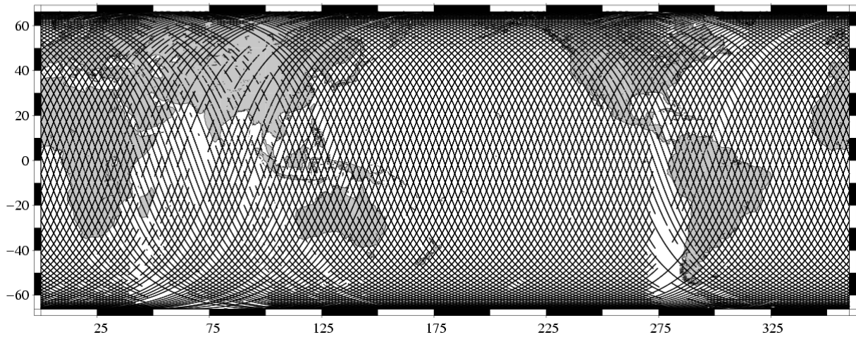
Missing measurements TOPEX/Poseidon Cycle 418 (19/01/2004 / 28/01/2004)
