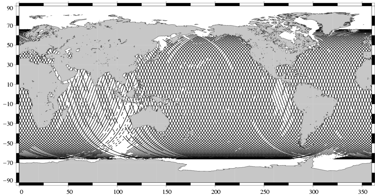
Edited measurements TOPEX Cycle 423 (08/03/2004 / 18/03/2004)
