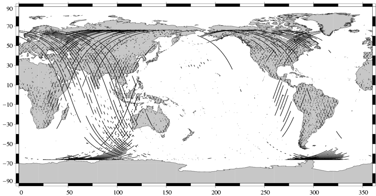
Missing measurements TOPEX/Poseidon Cycle 423 (08/03/2004 / 18/03/2004)
