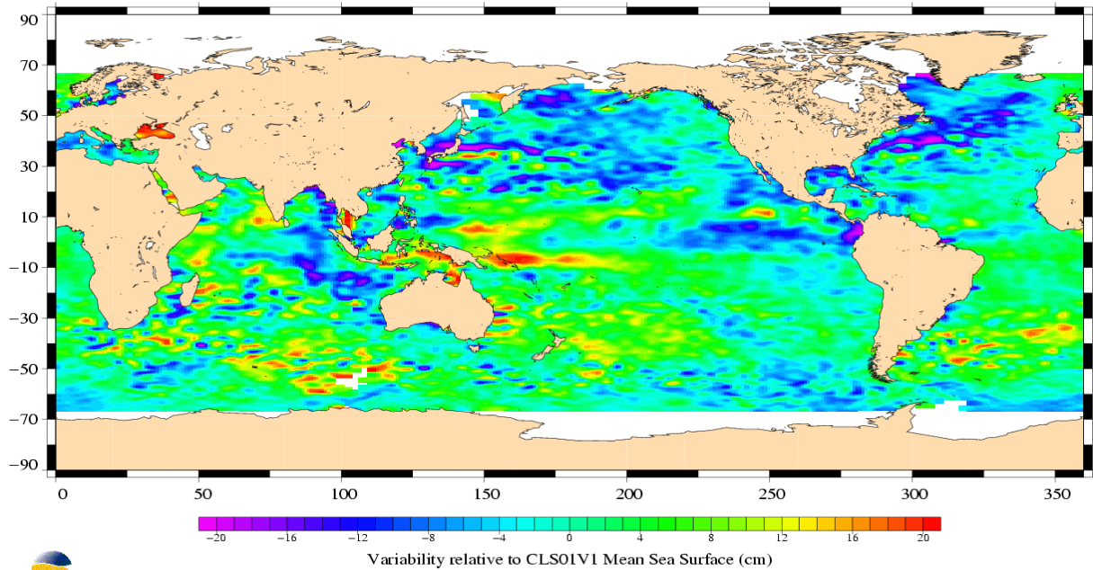
(SSH - MSS) differences greater than 0.3 m TOPEX/Poseidon Cycle 423 (08/03/2004 / 18/03/2004)
