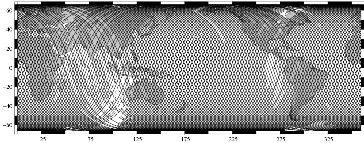
Missing measurements TOPEX/Poseidon Cycle 423 (08/03/2004 / 18/03/2004)
