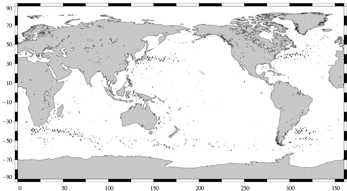
(SSH - MSS) differences greater than 0.3 m TOPEX/Poseidon Cycle 423 (08/03/2004 / 18/03/2004)
