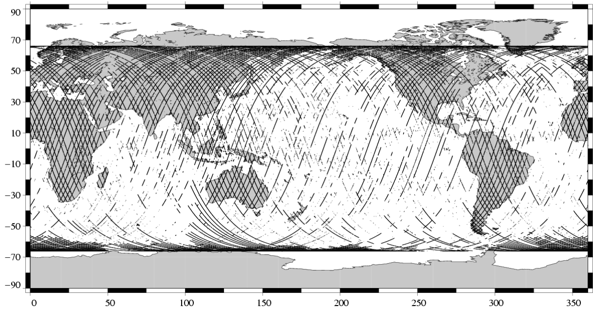
Edited measurements TOPEX Cycle 435 (05/07/2004 / 13/07/2004)
