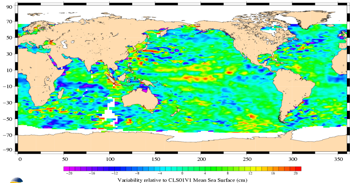
(SSH - MSS) differences greater than 0.3 m TOPEX/Poseidon Cycle 435 (05/07/2004 / 13/07/2004)
