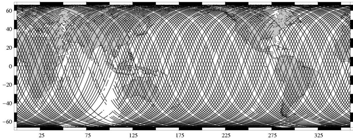
Missing measurements TOPEX/Poseidon Cycle 435 (05/07/2004 / 13/07/2004)
