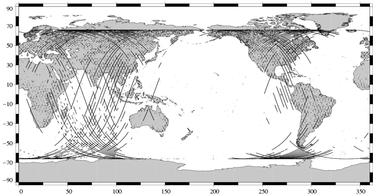
Missing measurements TOPEX/Poseidon Cycle 440 (24/08/2004 / 03/09/2004)
