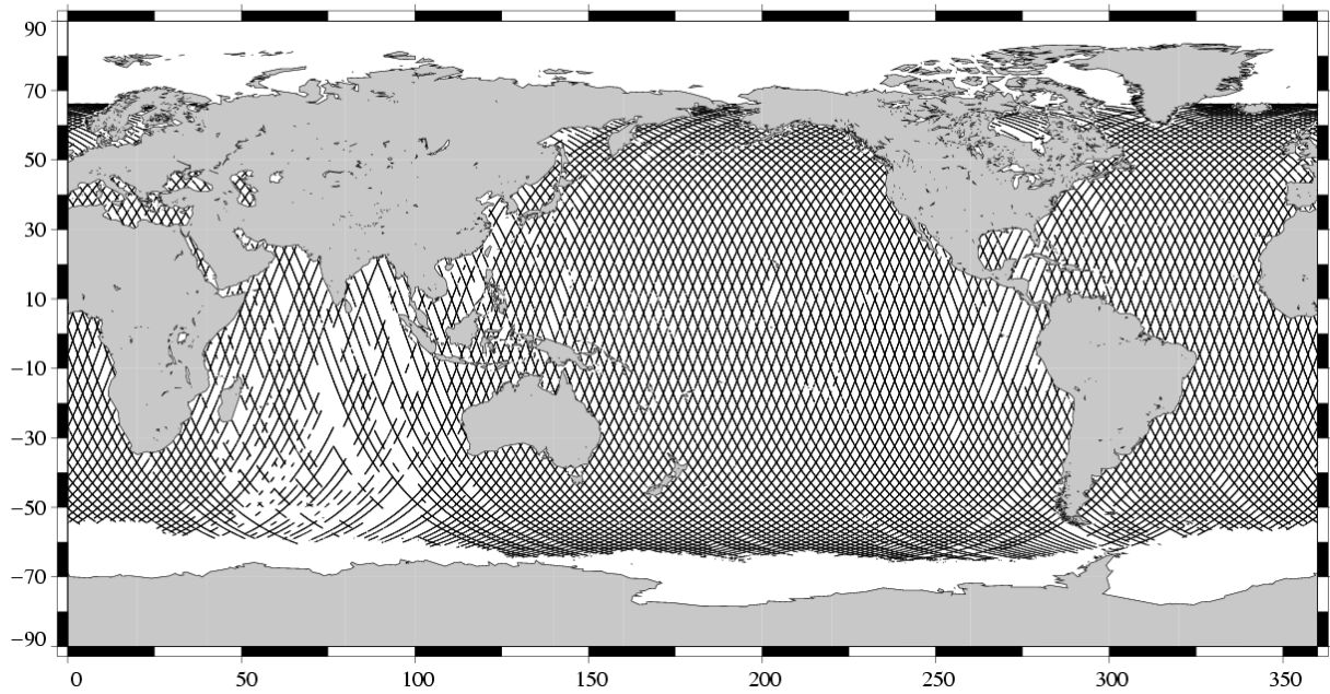
Edited measurements TOPEX Cycle 440 (24/08/2004 / 03/09/2004)
