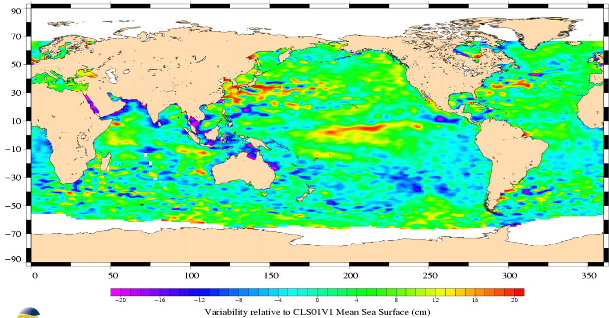
(SSH - MSS) differences greater than 0.3 m TOPEX/Poseidon Cycle 440 (24/08/2004 / 03/09/2004)
