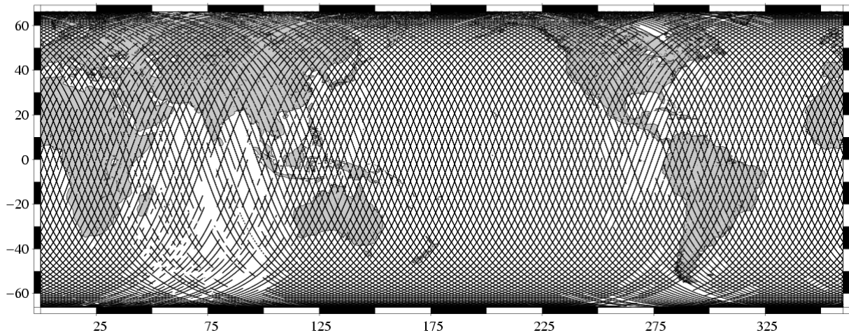
Missing measurements TOPEX/Poseidon Cycle 440 (24/08/2004 / 03/09/2004)
