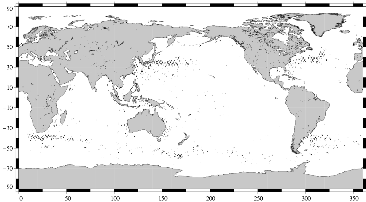
(SSH - MSS) differences greater than 0.3 m TOPEX/Poseidon Cycle 440 (24/08/2004 / 03/09/2004)
