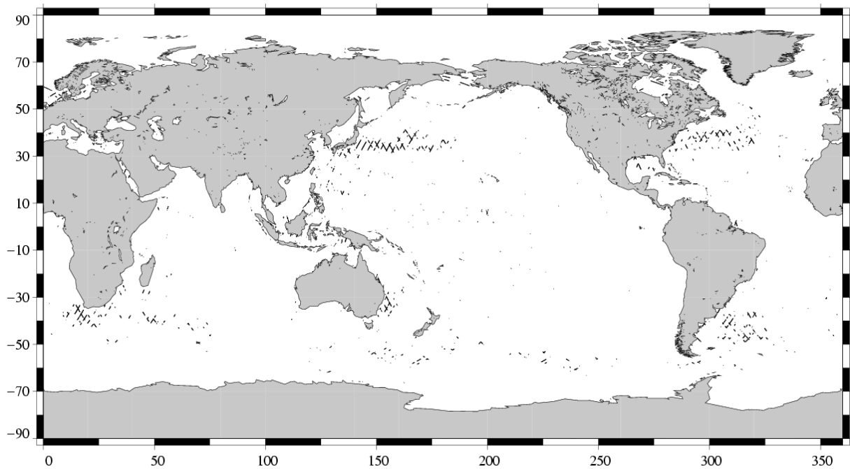
(SSH - MSS) differences greater than 0.3 m TOPEX/Poseidon Cycle 448 (11/11/2004 / 21/11/2004)
