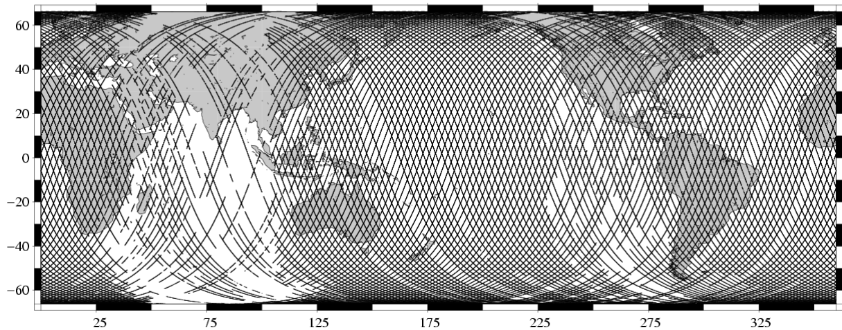
Missing measurements TOPEX/Poseidon Cycle 448 (11/11/2004 / 21/11/2004)
