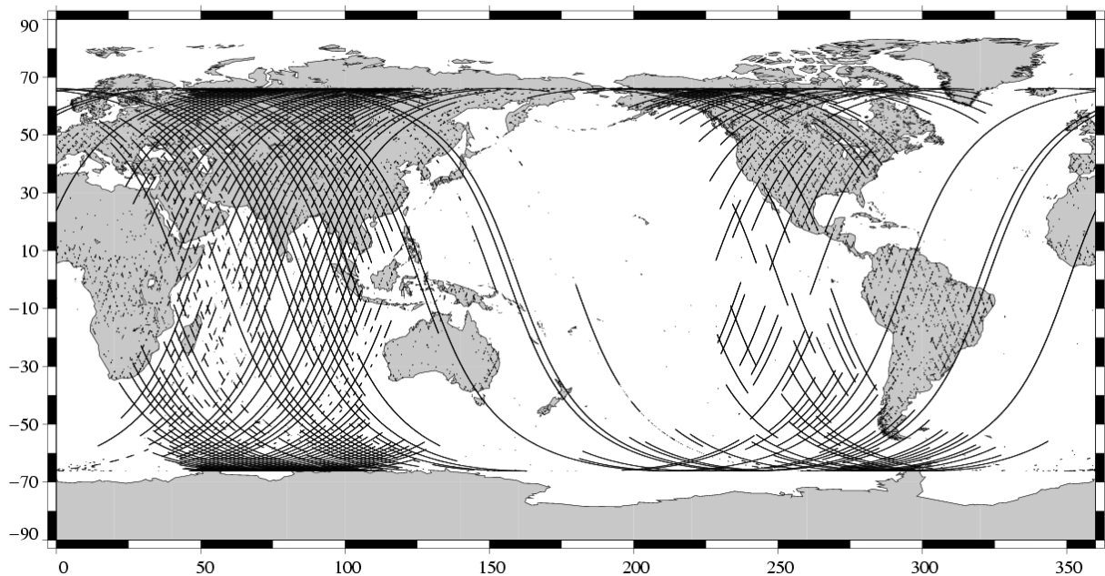
Missing measurements TOPEX/Poseidon Cycle 448 (11/11/2004 / 21/11/2004)
