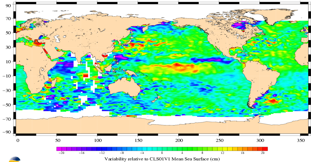
(SSH - MSS) differences greater than 0.3 m TOPEX/Poseidon Cycle 448 (11/11/2004 / 21/11/2004)
