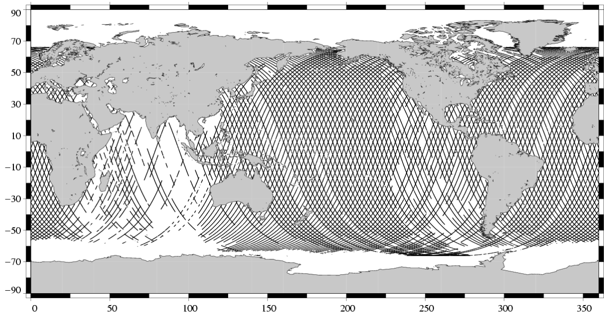
Edited measurements TOPEX Cycle 448 (11/11/2004 / 21/11/2004)
