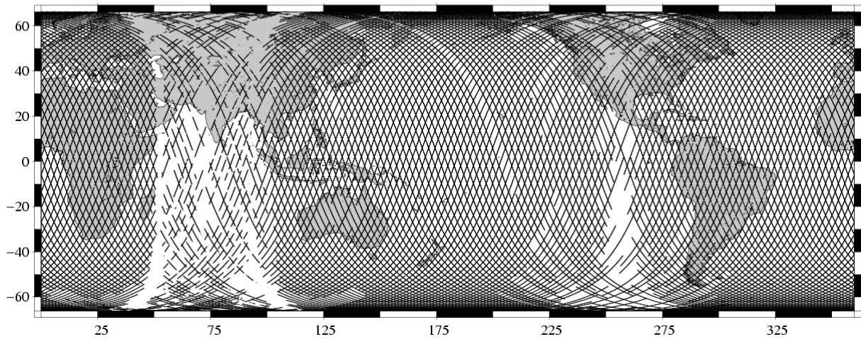
Missing measurements TOPEX/Poseidon Cycle 457 (08/02/2005 / 18/02/2005)
