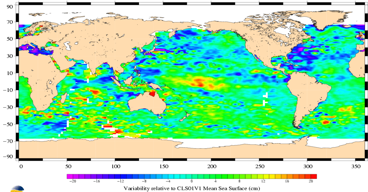
(SSH - MSS) differences greater than 0.3 m TOPEX/Poseidon Cycle 457 (08/02/2005 / 18/02/2005)
