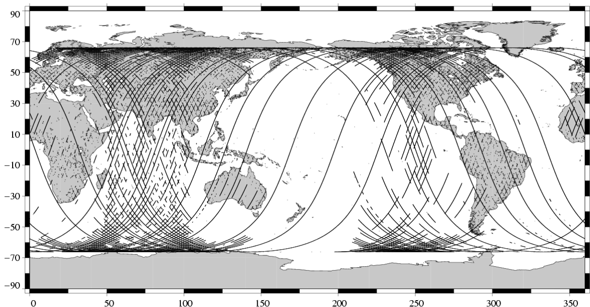
Missing measurements TOPEX/Poseidon Cycle 468 (28/05/2005 / 07/06/2005)
