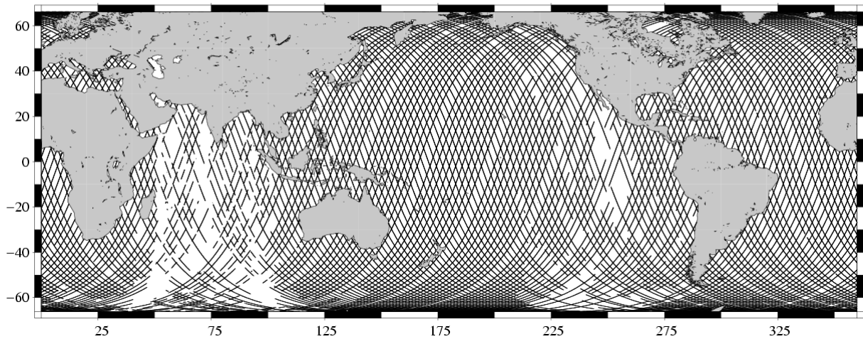
Missing measurements TOPEX/Poseidon Cycle 468 (28/05/2005 / 07/06/2005)
