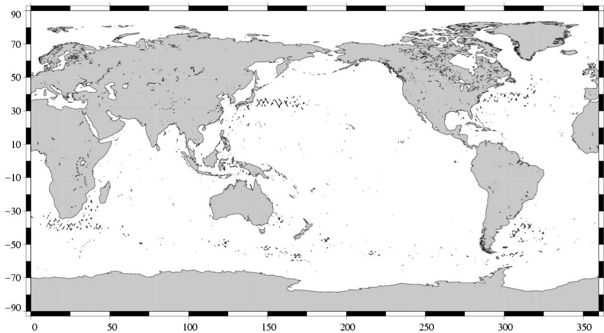
(SSH - MSS) differences greater than 0.3 m TOPEX/Poseidon Cycle 468 (28/05/2005 / 07/06/2005)
