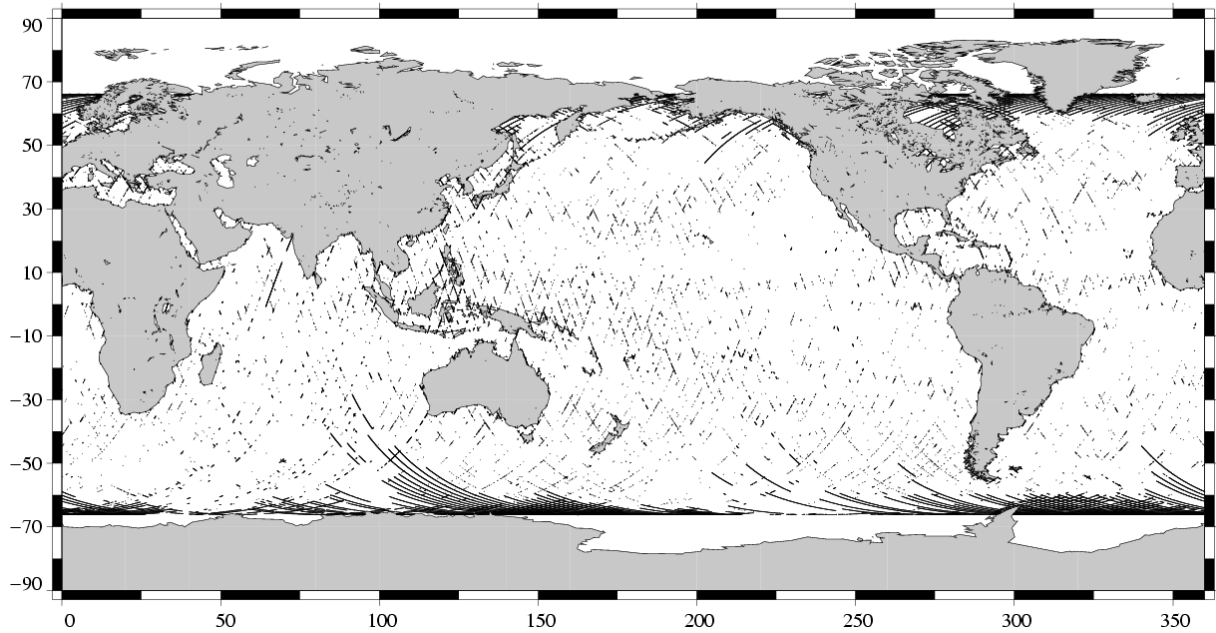
Edited measurements TOPEX Cycle 468 (28/05/2005 / 07/06/2005)
