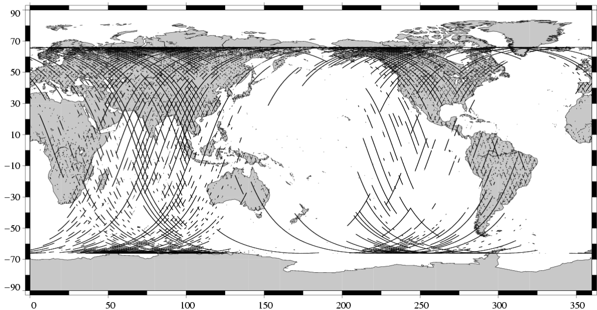
Missing measurements TOPEX/Poseidon Cycle 470 (17/06/2005 / 27/06/2005)
