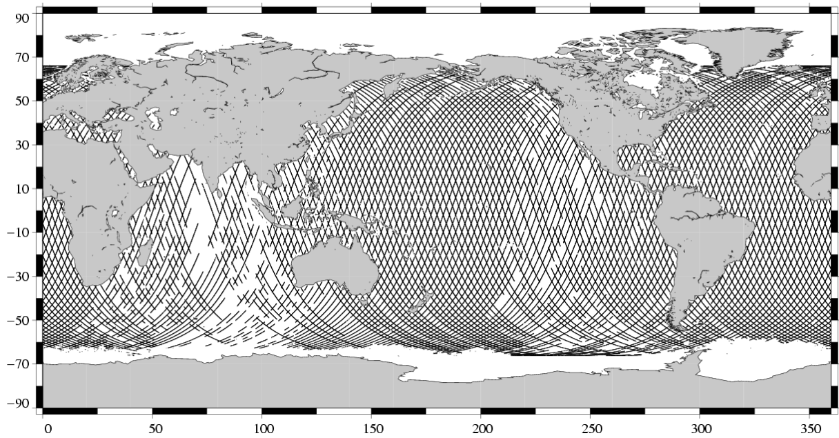
Edited measurements TOPEX Cycle 470 (17/06/2005 / 27/06/2005)
