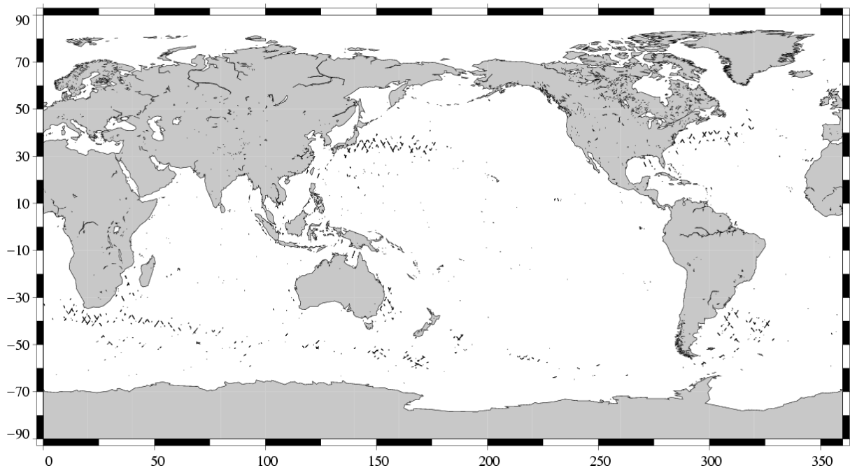
(SSH - MSS) differences greater than 0.3 m TOPEX/Poseidon Cycle 470 (17/06/2005 / 27/06/2005)
