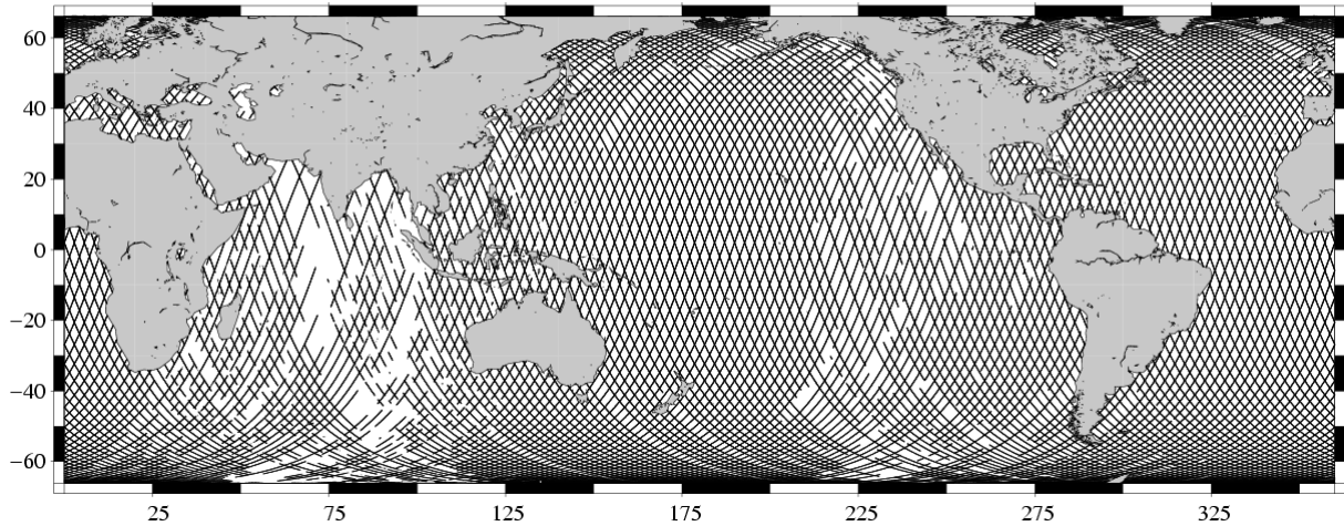
Missing measurements TOPEX/Poseidon Cycle 470 (17/06/2005 / 27/06/2005)
