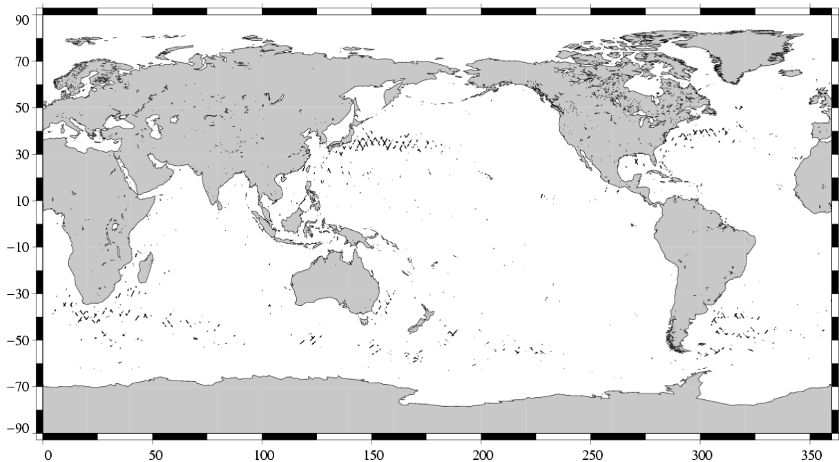
(SSH - MSS) differences greater than 0.3 m TOPEX/Poseidon Cycle 472 (07/07/2005 / 17/07/2005)
