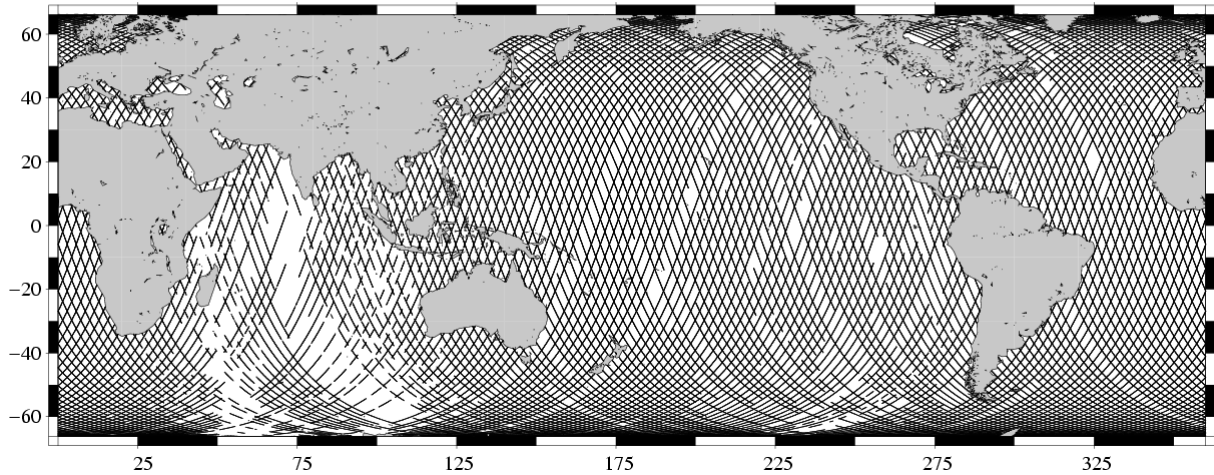
Missing measurements TOPEX/Poseidon Cycle 472 (07/07/2005 / 17/07/2005)
