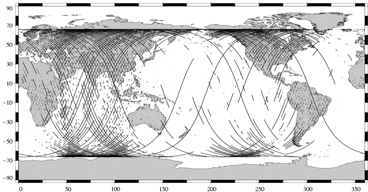
Missing measurements TOPEX/Poseidon Cycle 472 (07/07/2005 / 17/07/2005)
