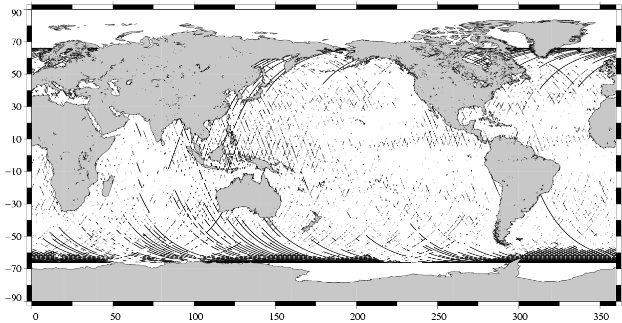
Edited measurements TOPEX Cycle 472 (07/07/2005 / 17/07/2005)
