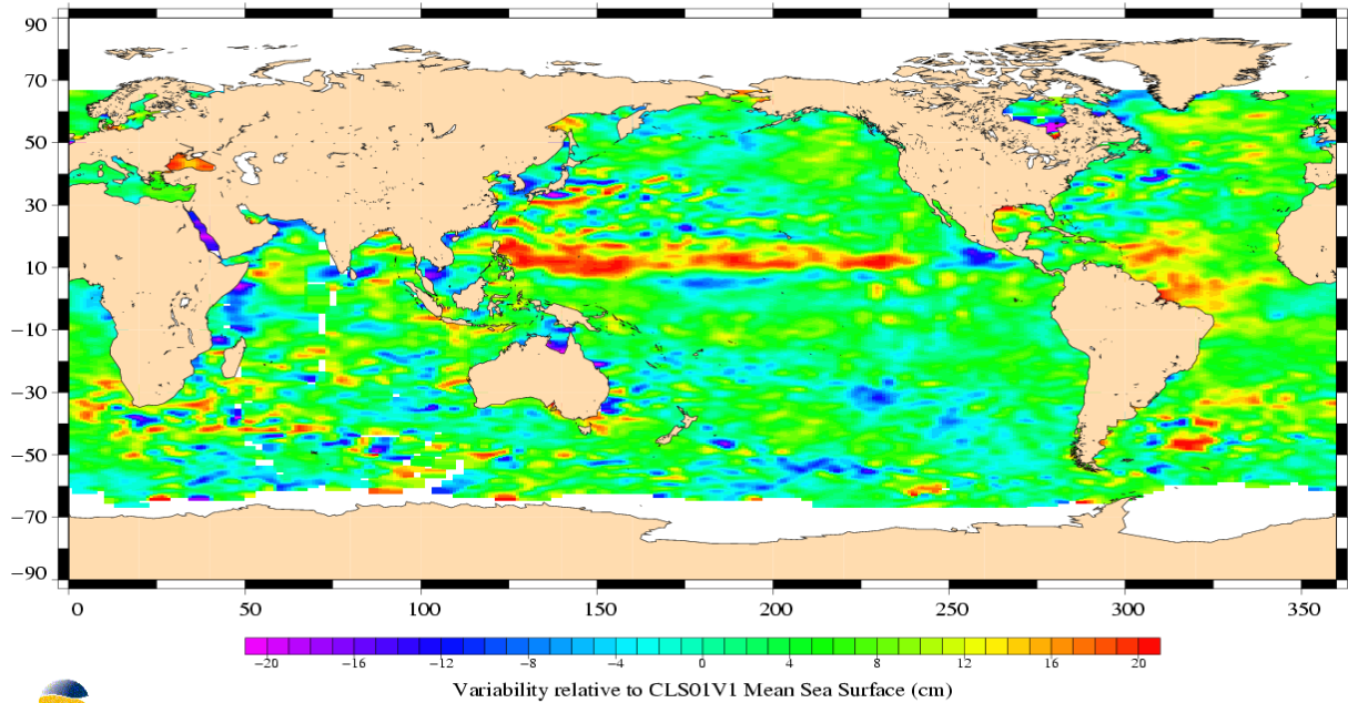
(SSH - MSS) differences greater than 0.3 m TOPEX/Poseidon Cycle 472 (07/07/2005 / 17/07/2005)
