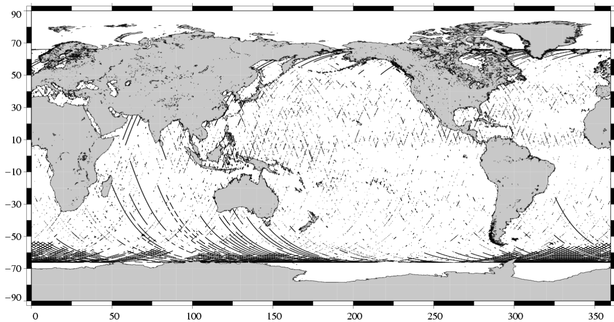
Edited measurements TOPEX Cycle 477 (26/08/2005 / 04/09/2005)
