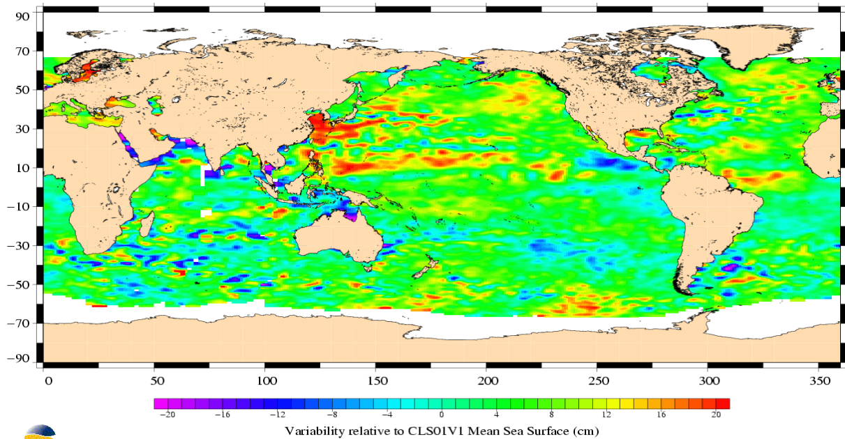
(SSH - MSS) differences greater than 0.3 m TOPEX/Poseidon Cycle 477 (26/08/2005 / 04/09/2005)
