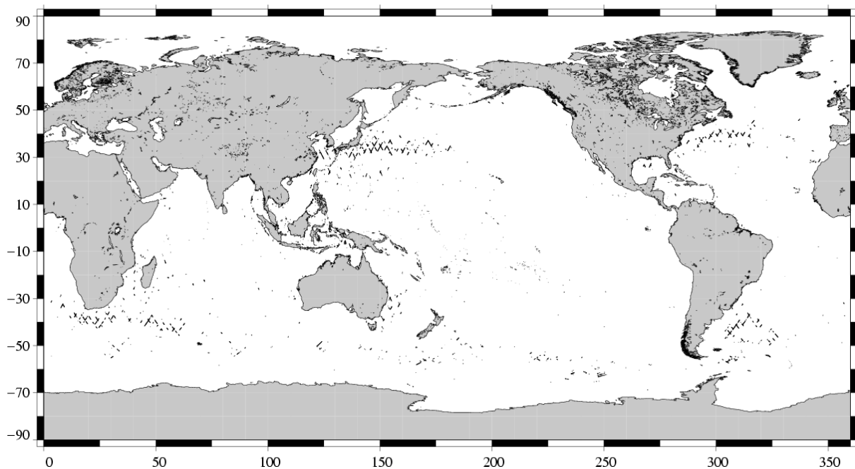
(SSH - MSS) differences greater than 0.3 m TOPEX/Poseidon Cycle 477 (26/08/2005 / 04/09/2005)
