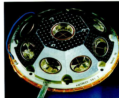
ERS-2 Laser Retro-Reflector An identical LRR will be flown on ENVISAT-1 (Photo courtesy of AEROSPATIALE)
