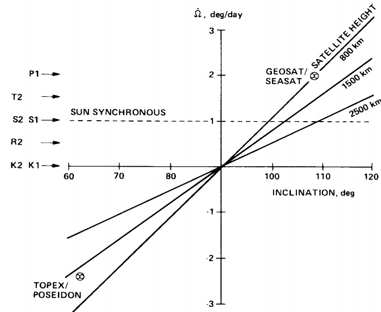
Fig. 7. The precession rate of the orbital plane as a function of inclination, with the altitude of the satellite as a parameter. To avoid aliasing the diurnal (K1, S1 and P1) and semidiurnal (T2, S2, R2, and K2) tides into long periods, orbits which are nearly sun-synchronous should be avoided. The indicated precession rates are those which alias the designated tidal constituent to zero frequency.
